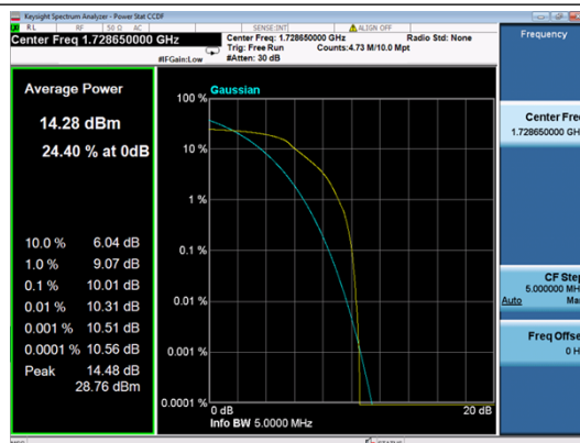
B4-15M-Mid CH-PAR-QPSK
