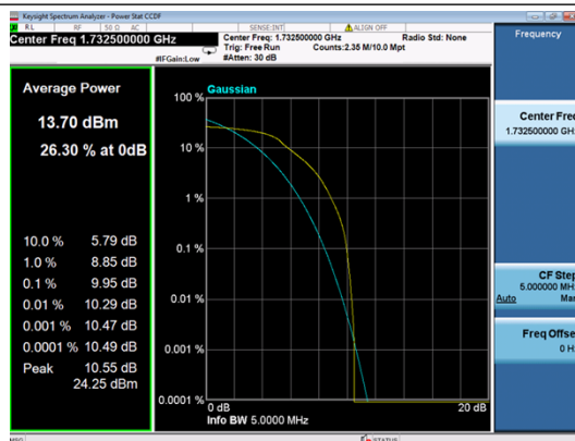
B4-3M-Mid CH-PAR-QPSK
