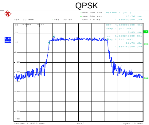
LTE Band 2: 99% Occupy bandwidth BW: 5MHz
