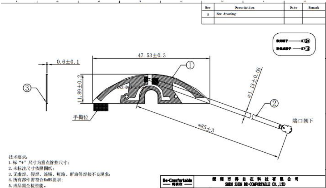
Zigbee antenna
