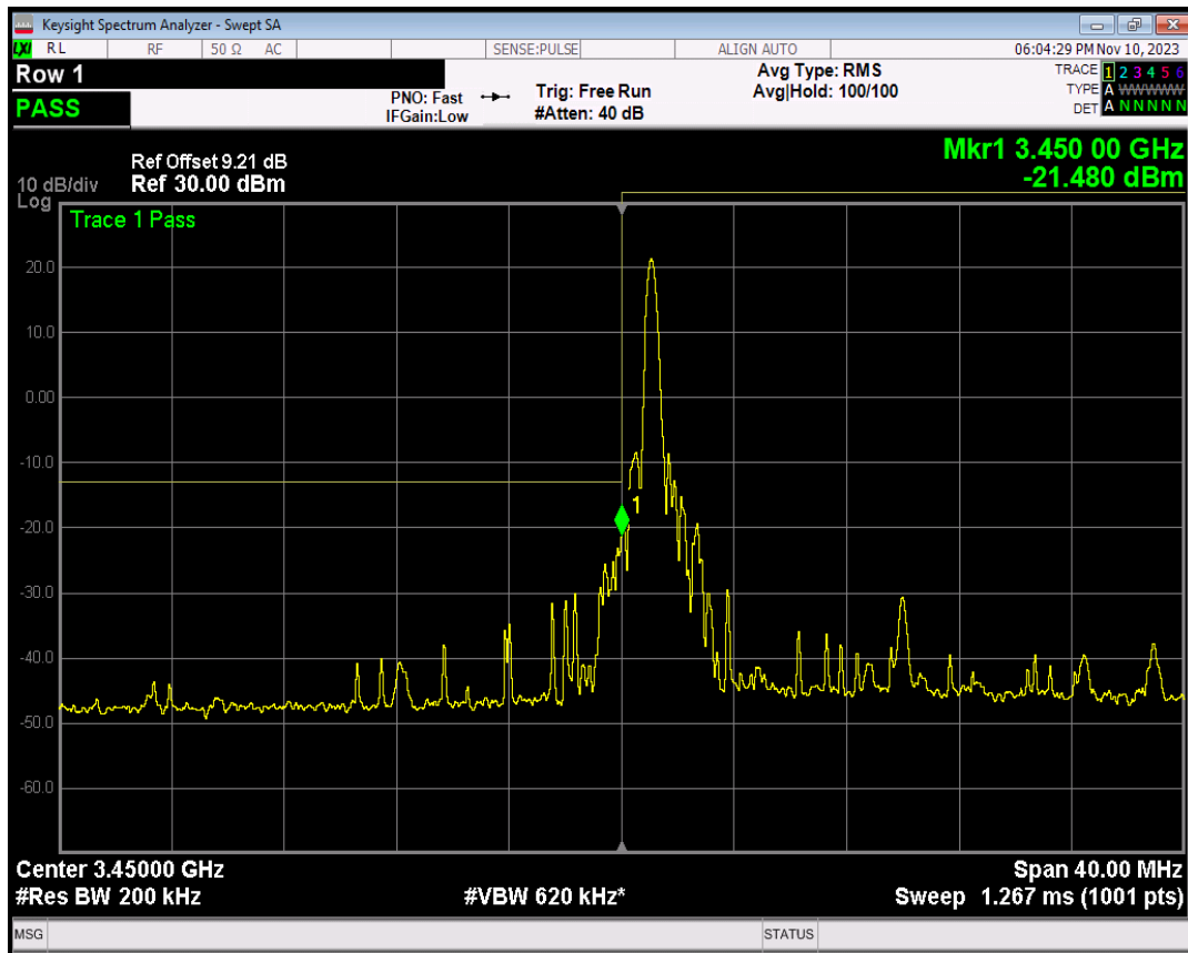
Band42 QPSK BW=20MHz Channel=42190 RB Size=1 Position=#Max
