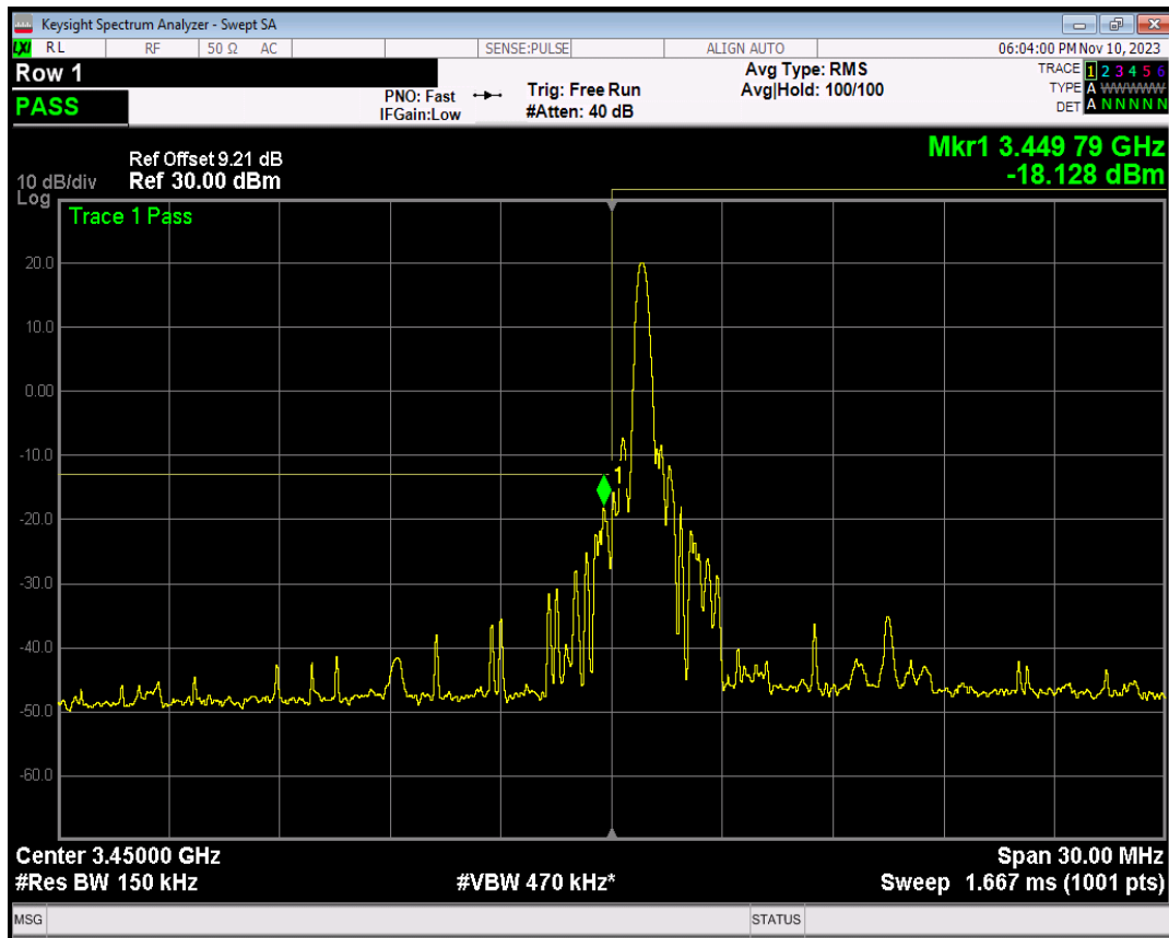
Band42 QPSK BW=15MHz Channel=42165 RB Size=1 Position=#Max
