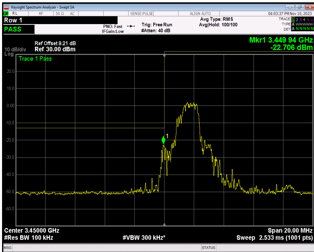
Band42 16QAM BW=10MHz Channel=42140 RB Size=1 Position=#Max
