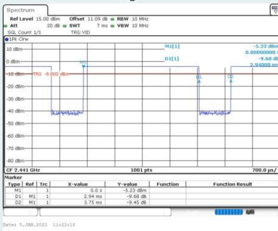
DH5_2441MHz
