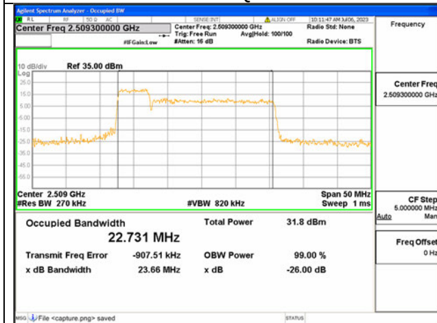
41C / 5+20MHz / 64QAM/ Low CH
