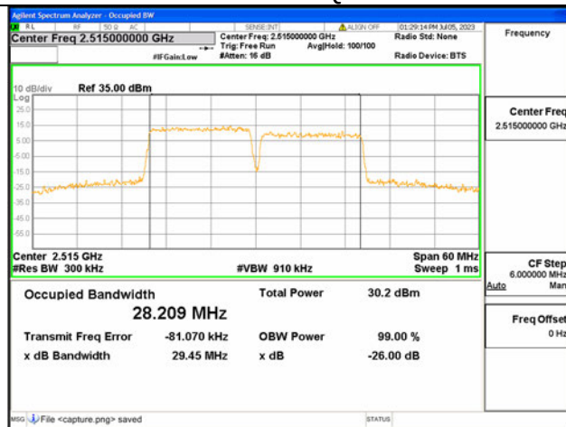
7C / 15+15MHz / 16QAM/ Low CH
