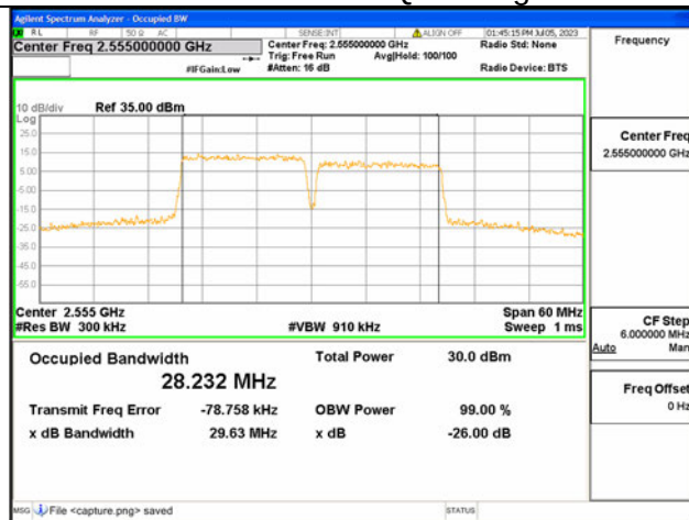
7C / 15+15MHz / 16QAM/ High CH
