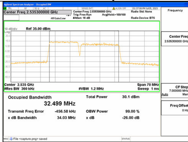
7C / 15+20MHz / 16QAM/ Mid CH
