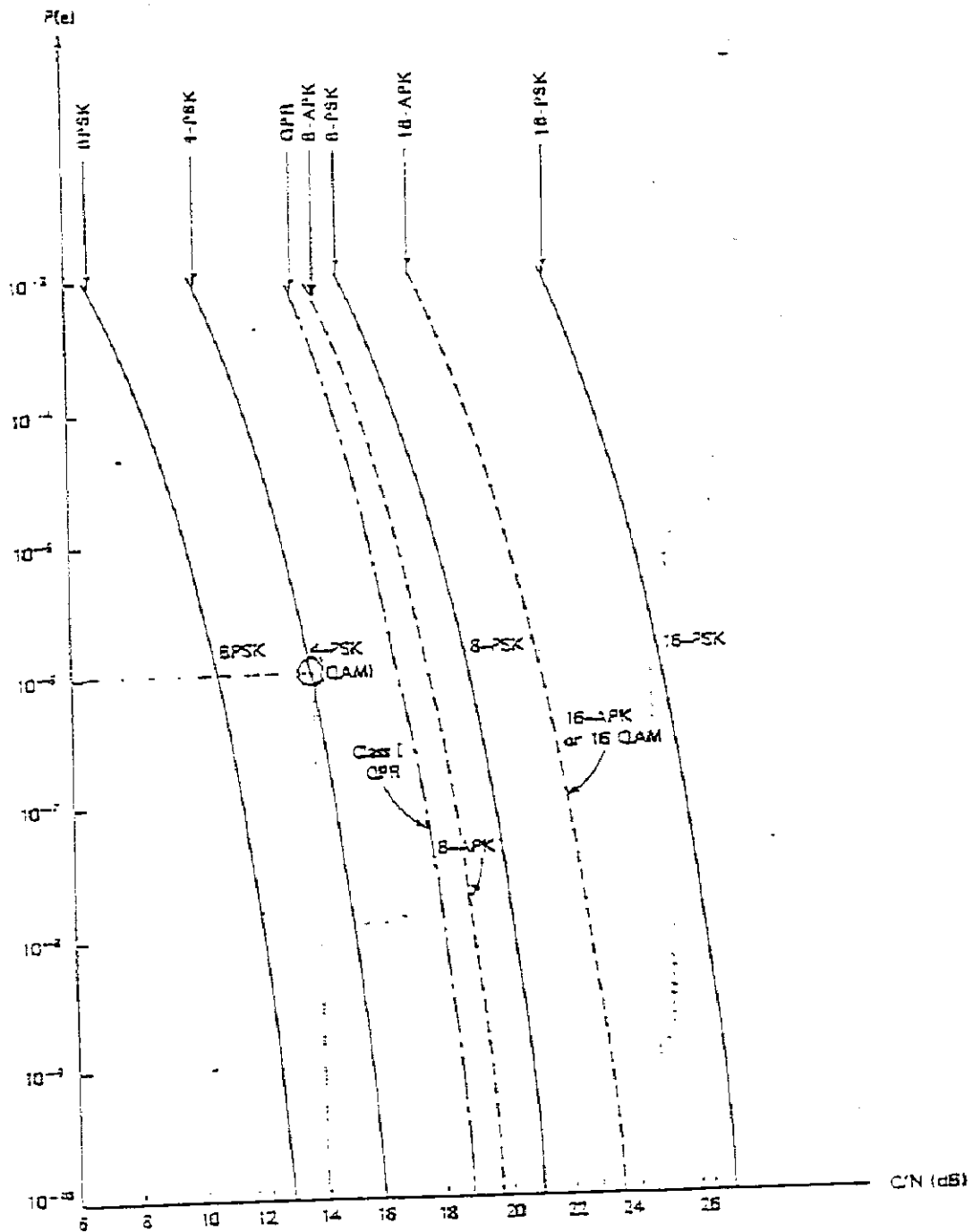
Fig. 1.11 P(e) performance of M -ary PSK, QAM, QPSK, and M -ary APSK coherent systems. The rms C/N is specified in the double-sided Nyquist bandwidth.
