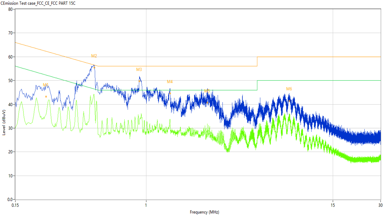
Figure 30: Conducted Emission on AC Mains, N Phase
