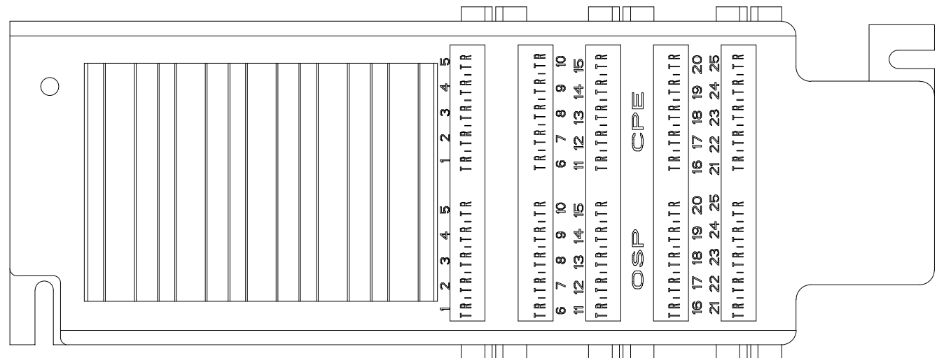
Figure 5-16: Punchdown Block
