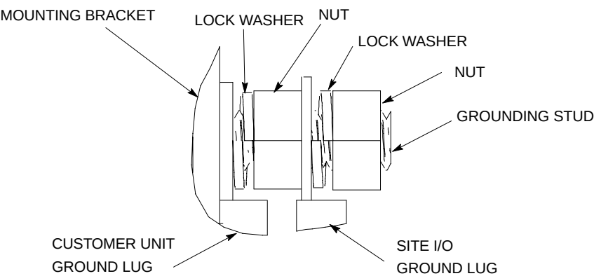
Figure 6-8: Grounding Stud on Mounting Bracket
