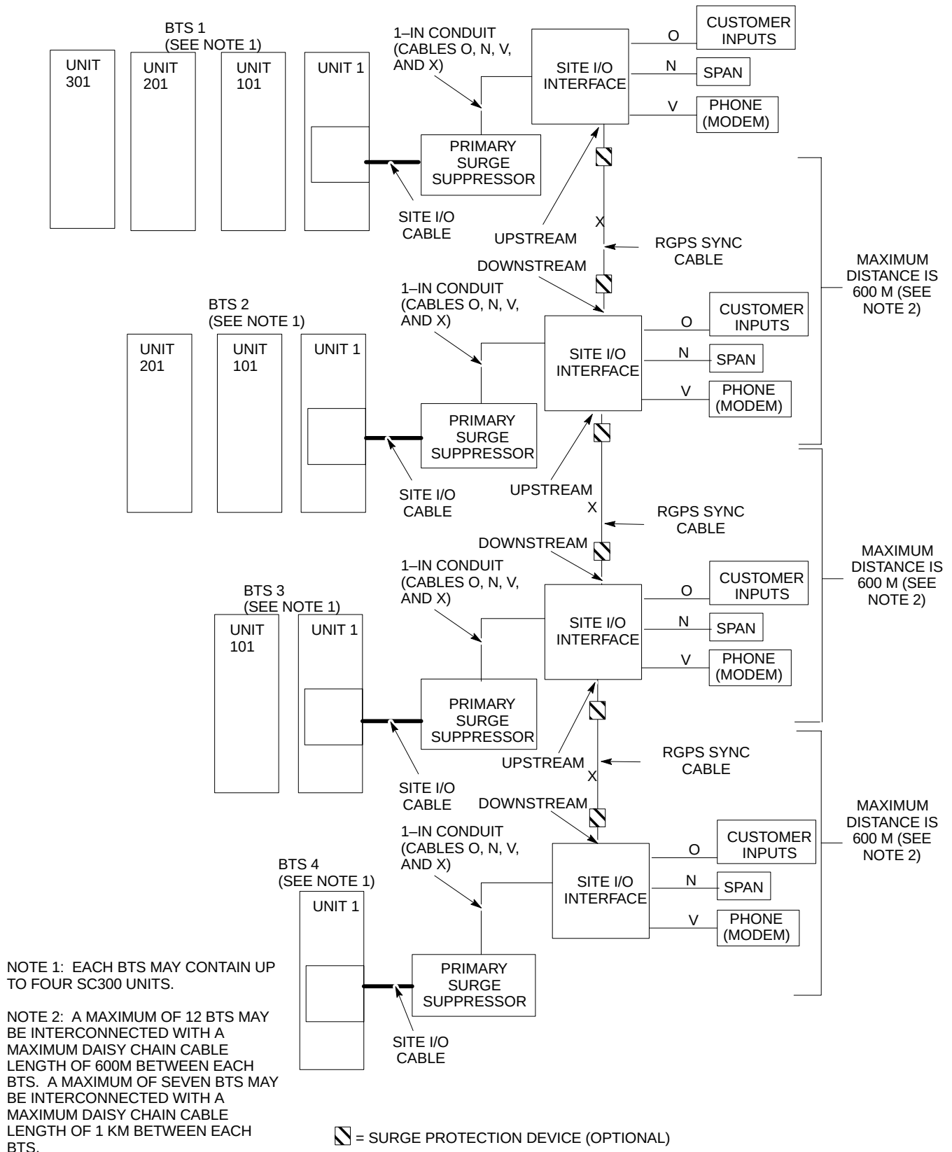
Figure 5-22: Site I/O Interface Cabling for HSO (Non-Synchronous) Configurations
