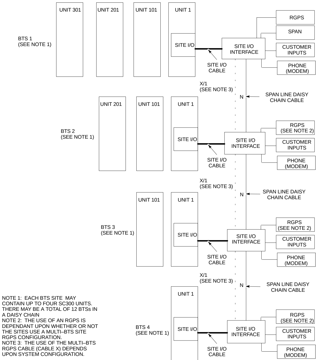
Figure 4-20: Site I/O Interface Cabling for Span Line Daisy Chain Cabling
