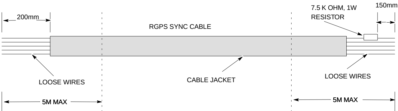
Figure 5-17: RGPS Sync Cable Diagram
