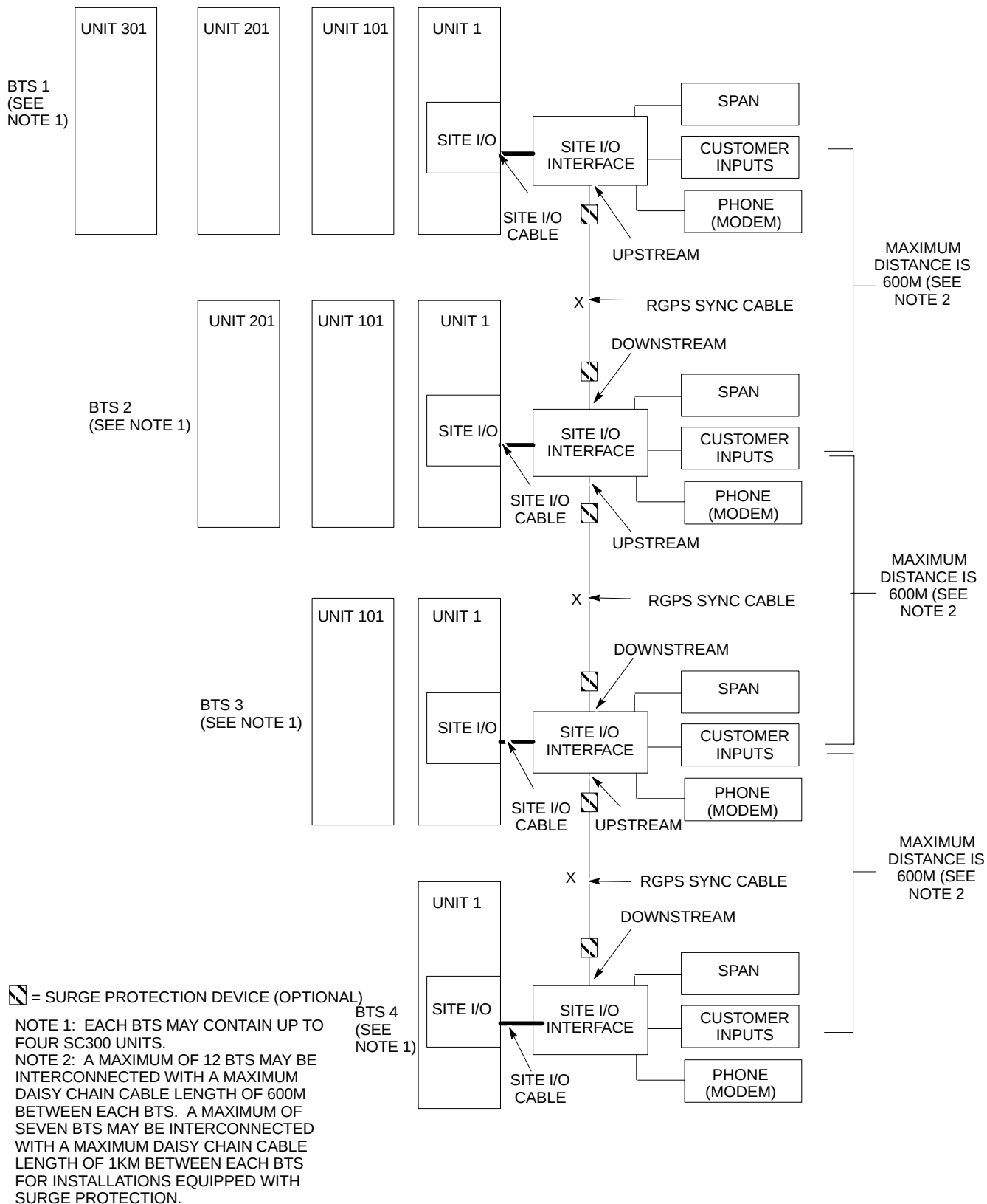
Figure 4-19: Site I/O Interface Cabling for HSO (Non-Synchronous) Configurations
