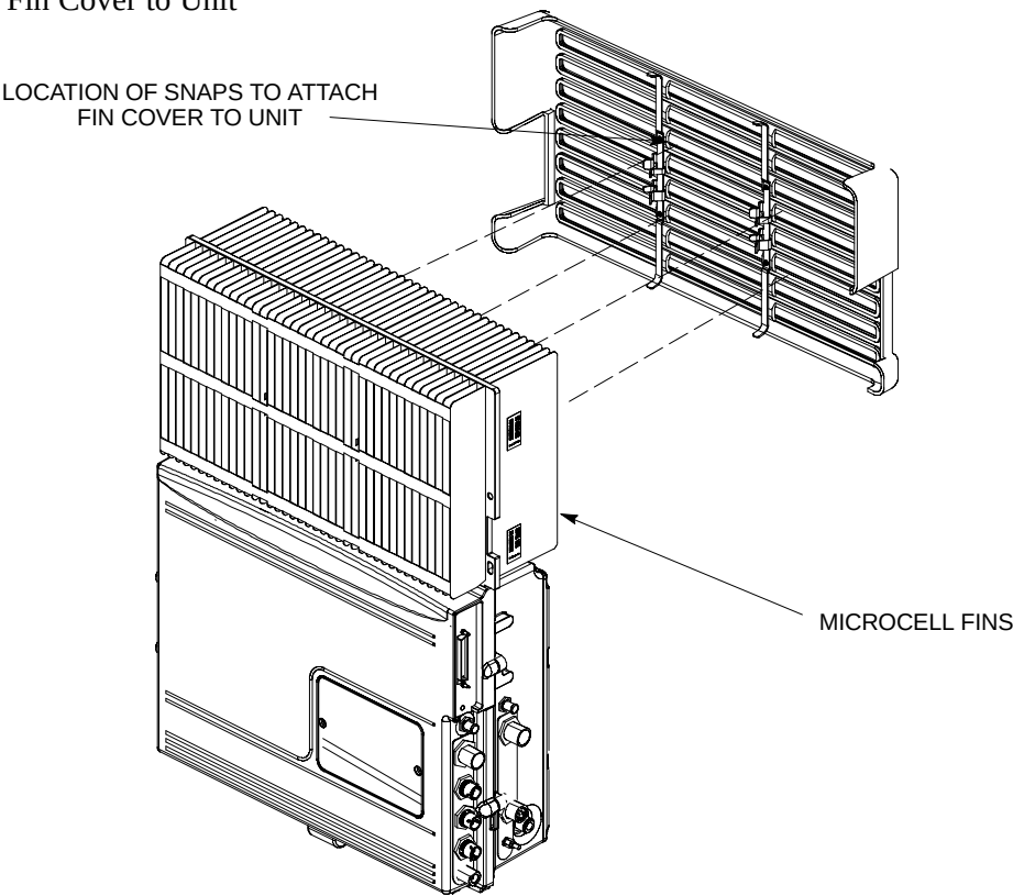
Figure 6-4: Attaching Back Fin Cover to Unit
