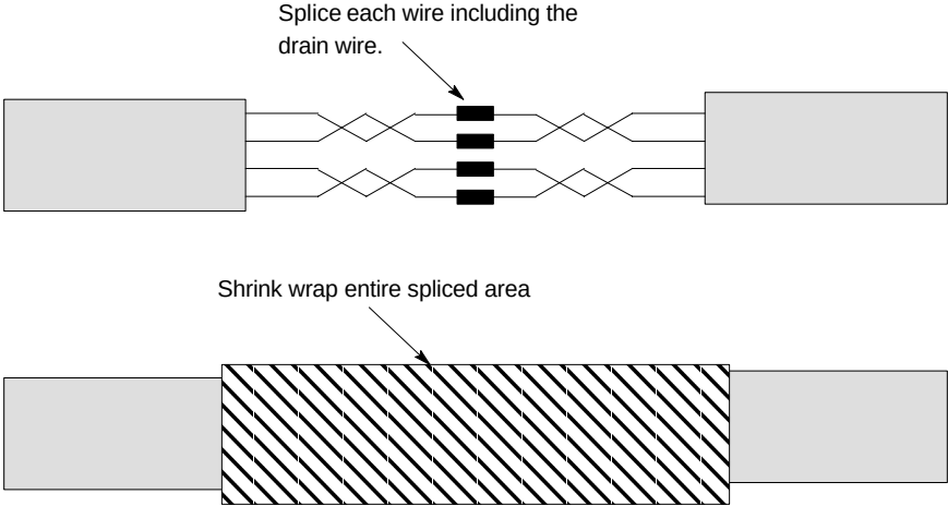
Figure 4-17: Cutting and Splicing RGPS Sync Cable
