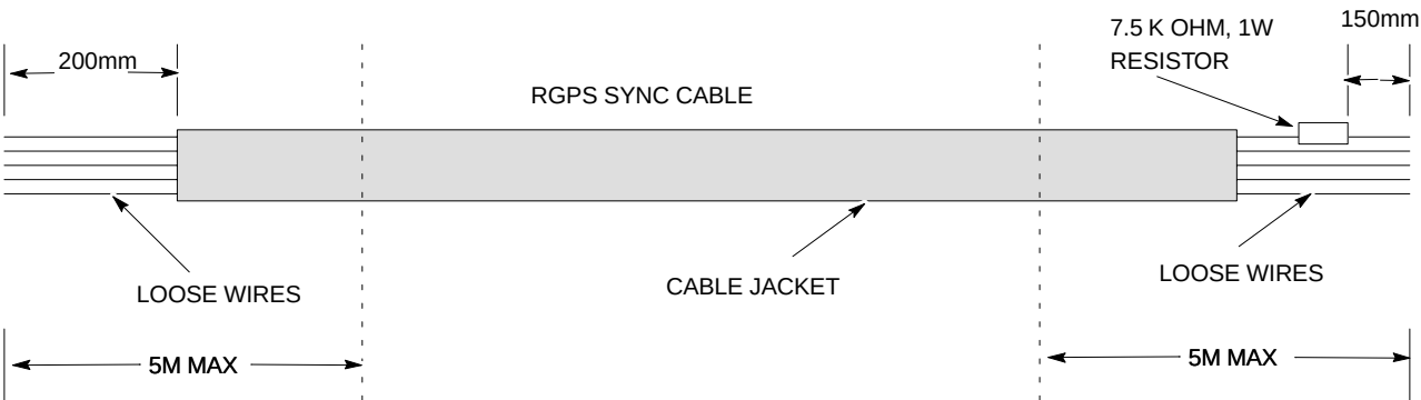
Figure 4-14: RGPS Sync Cable Diagram
