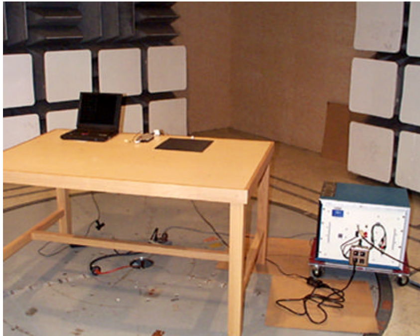
Conducted Emissions
