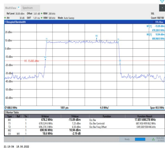
1-N71--15-20-H-5-DFT-256QAM-Outer_Full-100@0-A Ant1-17.852-18.600-≤20-PASS
