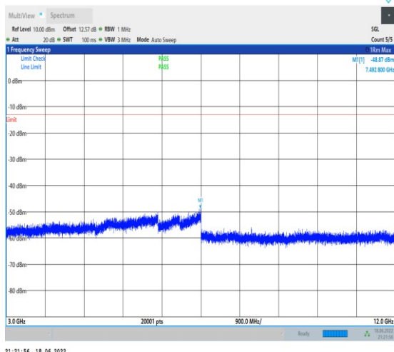
1-N71--15-20-L-1-DFT-PI2BPSK-Inner_1RB_Left-1 @1-3000-12000-Ant1--48.87--13-PASS
