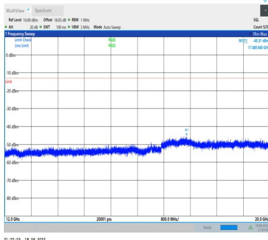
1-N71--15-20-L-1-DFT-PI2BPSK-Inner_1RB_Left-1@ 1-12000-20000-Ant1--45.31--13-PASS
