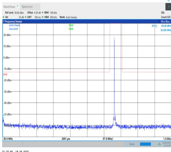
1-N71--15-20-M-1-DFT-PI2BPSK-Inner_1RB_Left-1 @1-30-1000-Ant1--54.28--13-PASS
