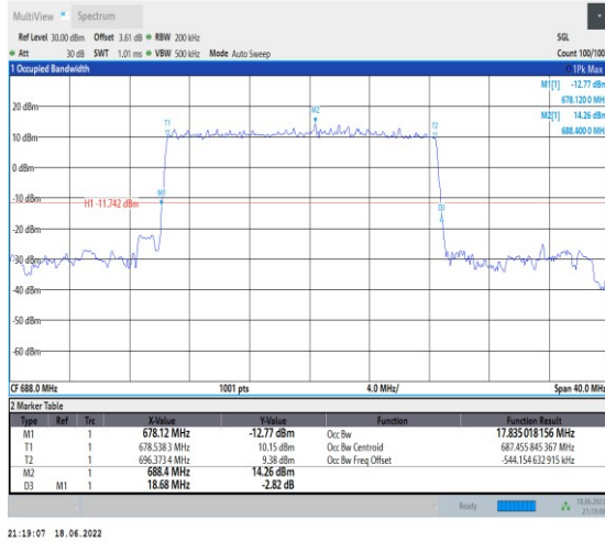
1-N71--15-20-H-2-DFT-PI2BPSK-Outer_Full-100@0-A Ant1-17.835-18.680-≤20-PASS
