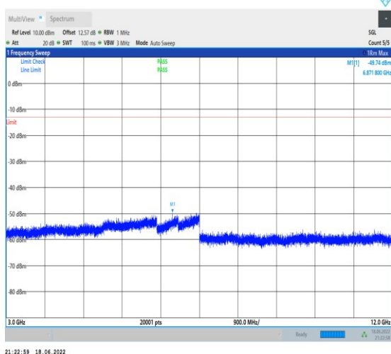
1-N71--15-20-M-1-DFT-PI2BPSK-Inner_1RB_Left-1 @1-3000-12000-Ant1--49.74--13-PASS
