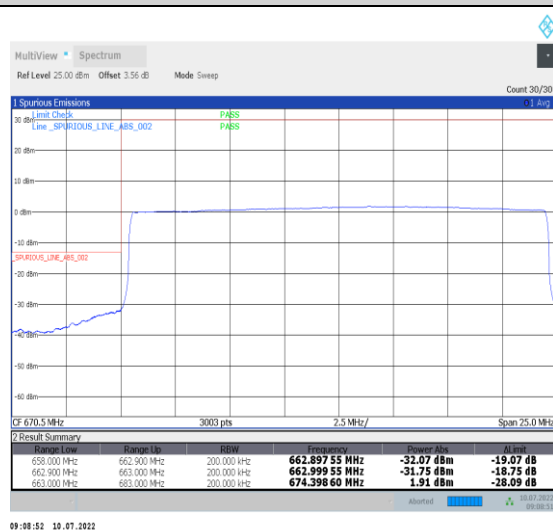
1-N71-PC3-15-20-L-6-CP-QPSK-Outer_Full- 106@0-Ant1-PASS-see graph
