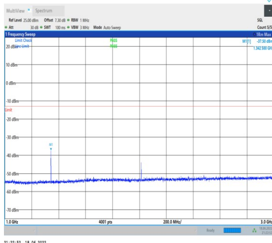
1-N71--15-20-M-1-DFT-PI2BPSK-Inner_1RB_Left-1 @1-1000-3000-Ant1--37.50--13-PASS
