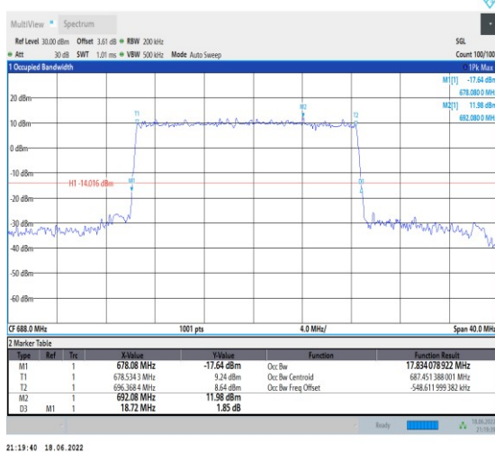
1-N71--15-20-H-4-DFT-64QAM-Outer_Full-100@0-A nt1-17.834-18.720-≤20-PASS
