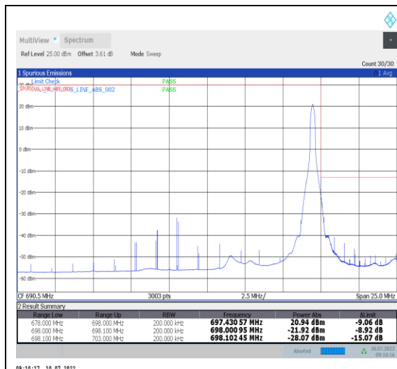
09:10:17 10.07.2022 1-N71-PC3-15-20-H-2-DFT-PI2BPSK-Edge_1RB_Right-1@105-Ant1-PASS-see graph
