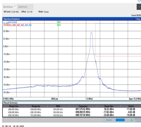
1-N71--15-10-H-5-CP-QPSK-Edge_1RB_Right-1@51- Ant1-PASS-see graph
