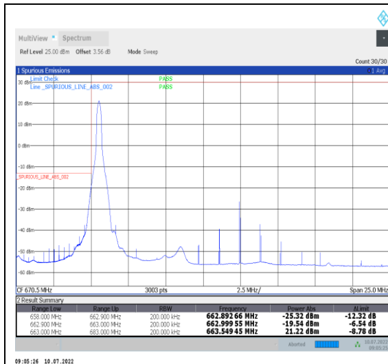
1-N71-PC3-15-20-L-1-DFT-PI2BPSK-Edge_1 RB_Left-1@0-Ant1-PASS-see graph
