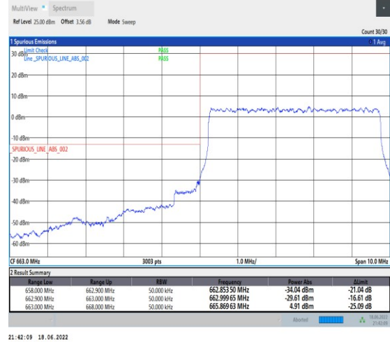
1-N71--15-5-L-3-DFT-PI2BPSK-Outer_Full-25@0-Ant1-PASS-see graph
