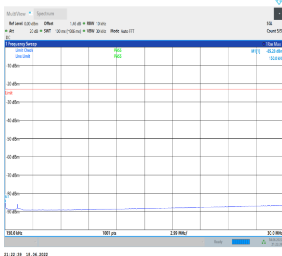
1-N71--15-20-M-1-DFT-PI2BPSK-Inner_1RB_Left-1 @1-0.15-30-Ant1--85.28--23-PASS
