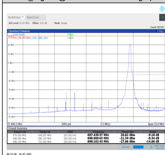
09:12:34 10.07.2022 1-N71-PC3-15-20-H-5-CP-QPSK-Edge_1RB_Right-1@105-Ant1-PASS-see graph
