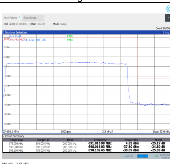
09:11:24 10.07.2022 1-N71-PC3-15-20-H-3-DFT-PI2BPSK-Outer_Full-100@0-Ant1-PASS-see graph
