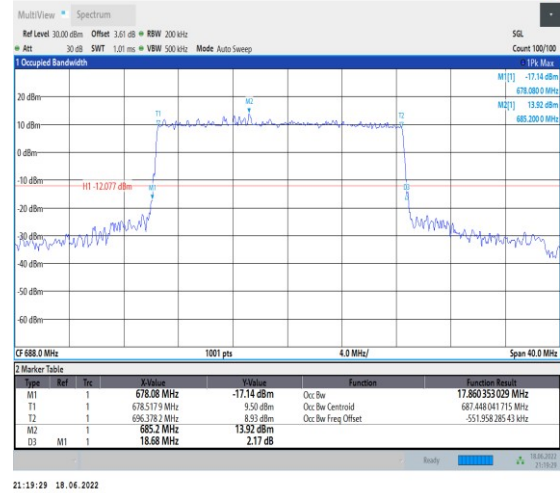
1-N71--15-20-H-3-DFT-16QAM-Outer_Full-100@0-A nt1-17.86-18.680-≤20-PASS
