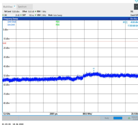
1-N71--15-20-M-1-DFT-PI2BPSK-Inner_1RB_Left-1 @1-12000-20000-Ant1--45.85--13-PASS
