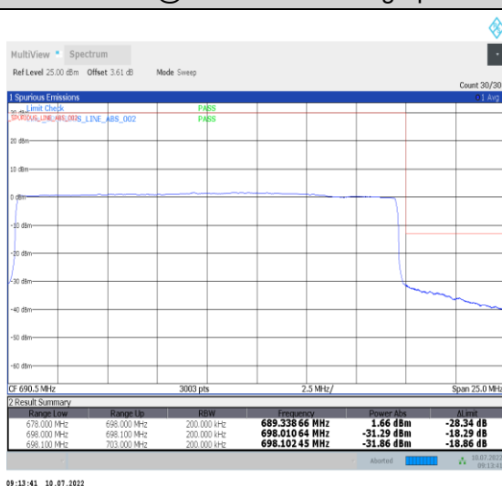
09:13:41 10.07.2022 1-N71-PC3-15-20-H-6-CP-QPSK-Outer_Full-106@0-Ant1-PASS-see graph
