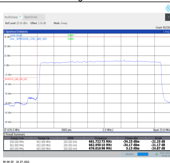
1-N71-PC3-15-20-L-3-DFT-PI2BPSK-Outer_ Full-100@0-Ant1-PASS-see graph
