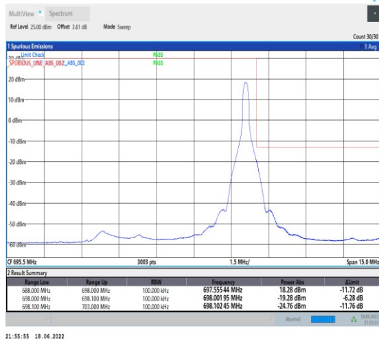
1-N71--15-10-H-2-DFT-PI2BPSK-Edge_1RB_Right-1@ 51-Ant1-PASS-see graph
