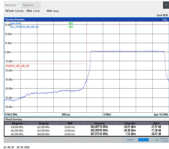
1-N71--15-5-L-6-CP-QPSK-Outer_Full-25@0-Ant1-PASS-see graph
