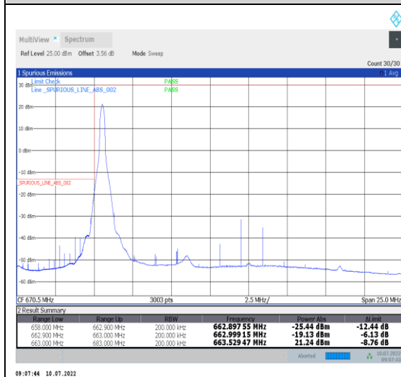
1-N71-PC3-15-20-L-4-CP-QPSK-Edge_1RB _Left-1@0-Ant1-PASS-see graph
