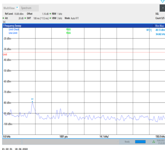
1-N71--15-20-M-1-DFT-PI2BPSK-Inner_1RB_Left-1 @1-0.009-0.15-Ant1--80.13--33-PASS
