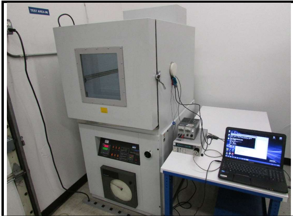
Test Setup Photo # 7
