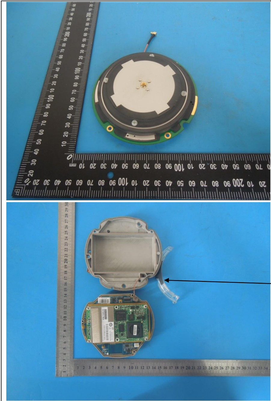
2G/3G Antenna
