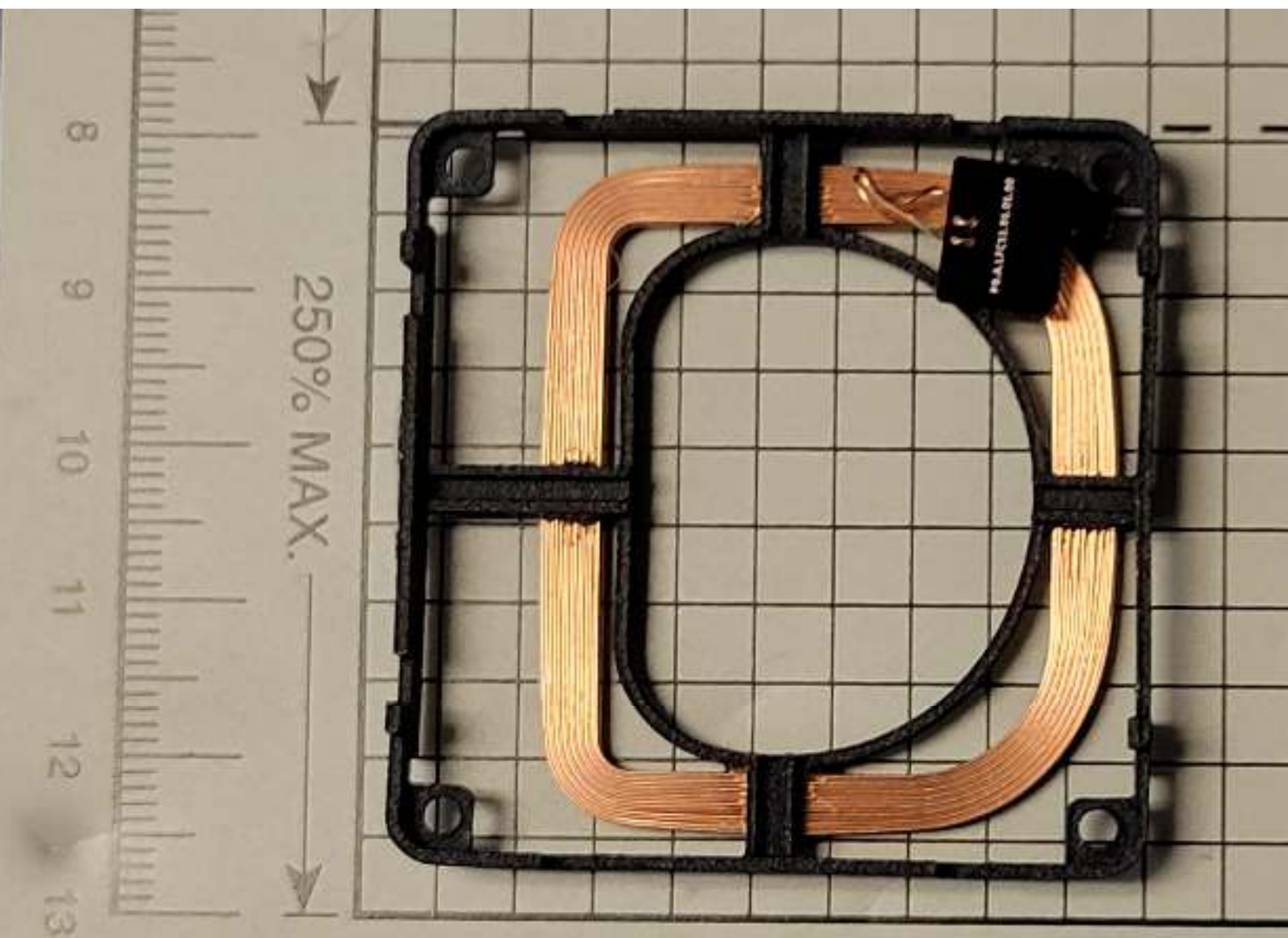
LF ANTENNA
