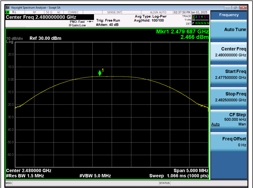
Test_Graph_LE1M_ANT1_2480_1Mbps_Peak Power
