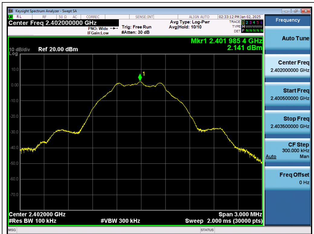
Test_Graph_LE1M_ANT1_2402_1Mbps_Reference Level
