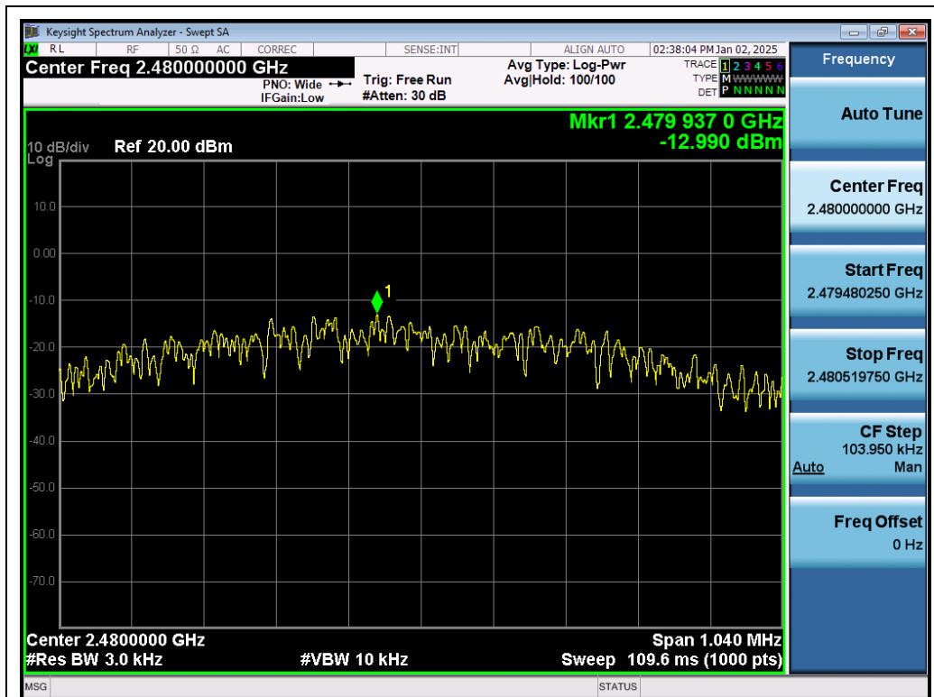
Test_Graph_LE1M_ANT1_2480_1Mbps_PSD
