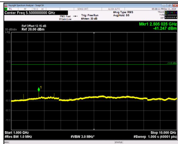
5-5-5MHz-3MHz-QPSK-QPSK-20510-20549-1RB#0-0RB#0-1000~10000MHz-PASS
