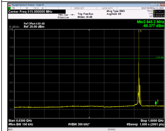
5-5-5MHz-3MHz-QPSK-QPSK-20510-20549-1RB#0-0RB#0-30~1000MHz-PASS
