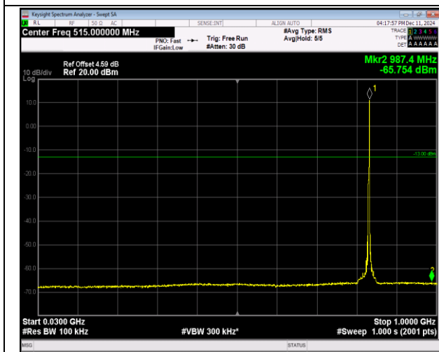
5-5-3MHz-5MHz-QPSK-QPSK-20501-20540-1RB#14-0RB B#0-30~1000MHz-PASS
