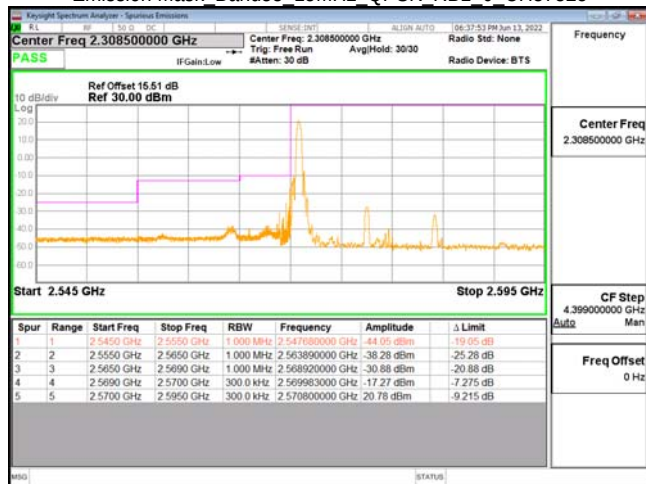
Emission Mask Band38 15MHz QPSK RB1 74 CH38175
