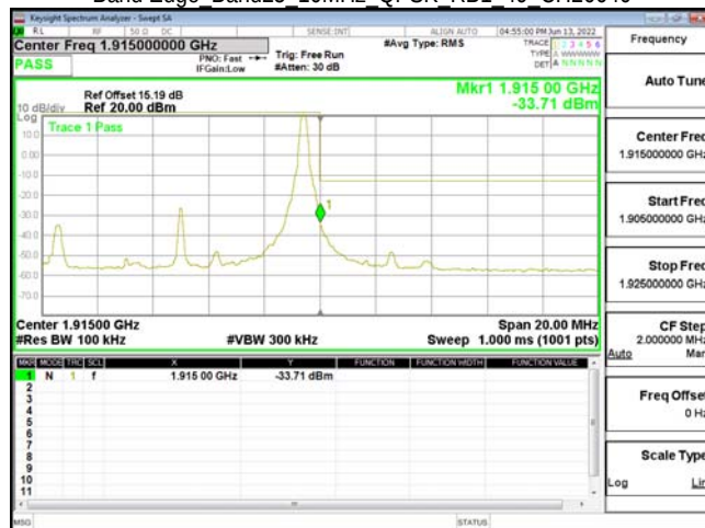
Band Edge Band25 10MHz QPSK RB1 49 CH26640
