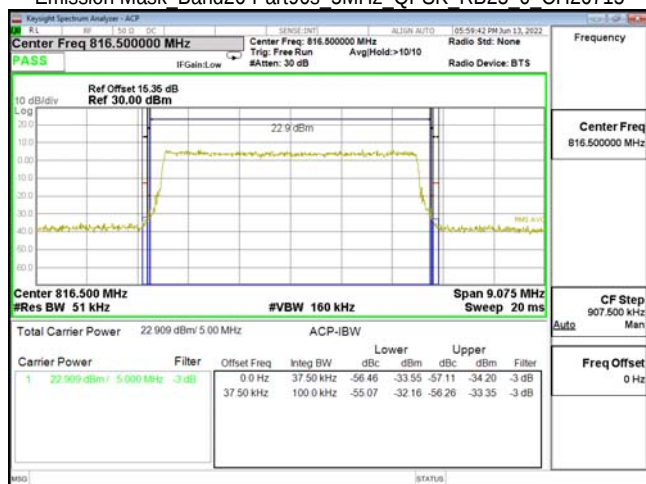
Emission Mask Band26-Part90s 5MHz QPSK RB25 0 CH26715
