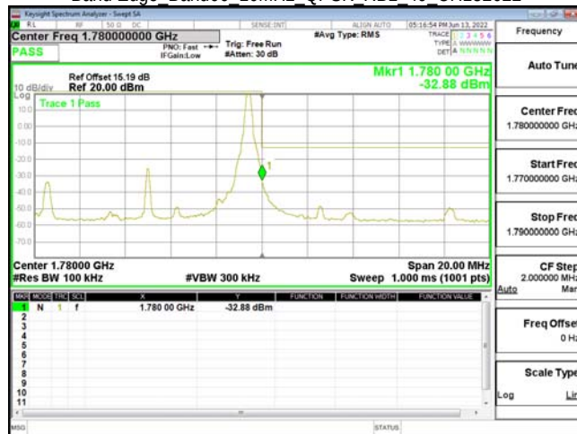
Band Edge Band66 10MHz QPSK RB50 0 CH132022
