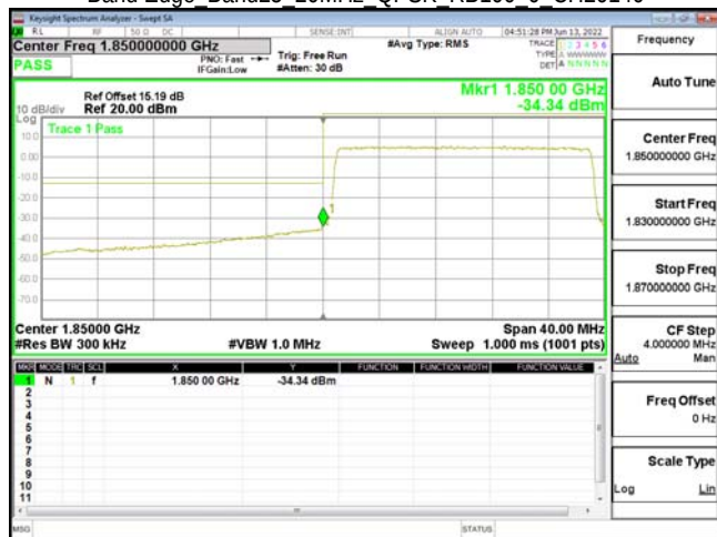
Band Edge Band25 20MHz QPSK RB100 0 CH26140
