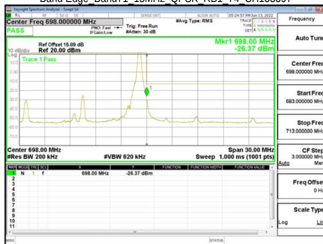
Band Edge Band71 15MHz QPSK RB1 74 CH133397
