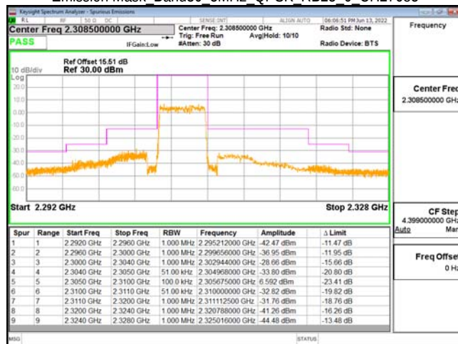
Emission Mask Band30 5MHz QPSK RB25 0 CH27685
