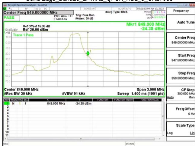
Band Edge Band26 1.4MHz QPSK RB1 5 CH27033
