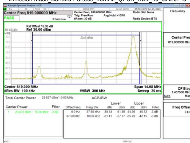
Emission Mask Band26-Part90s 10MHz QPSK RB1 49 CH26740
