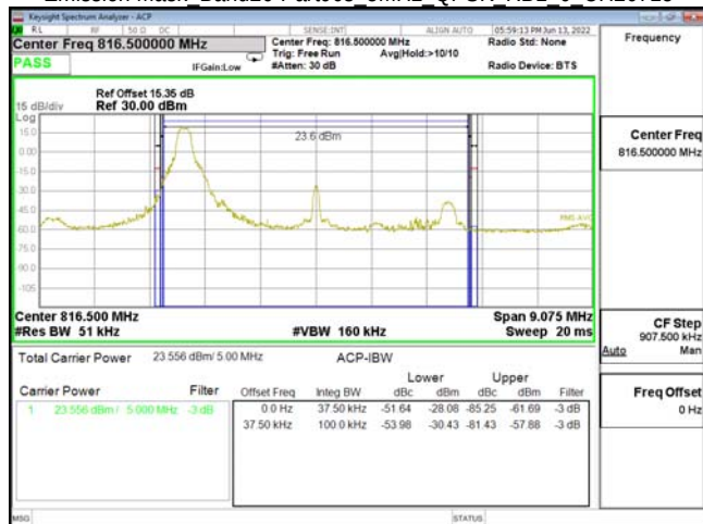
Emission Mask Band26-Part90s 5MHz QPSK RB1 24 CH26765
