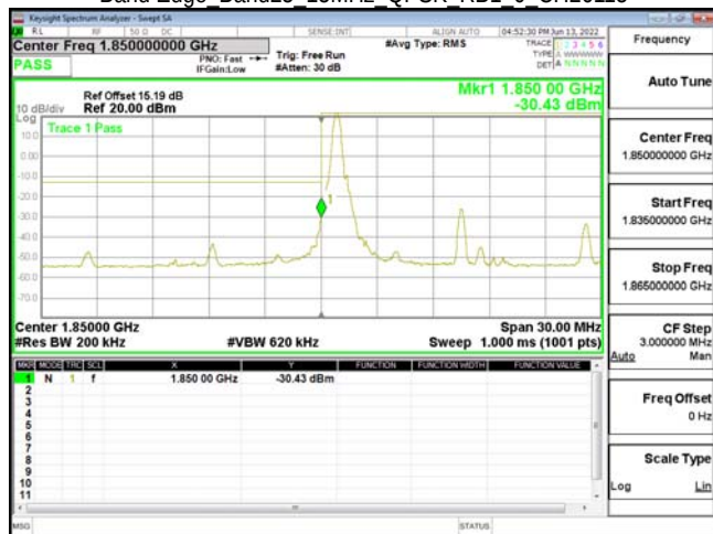
Band Edge Band25 15MHz QPSK RB1 0 CH26115
