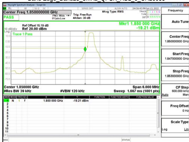
Band Edge Band25 3MHz QPSK RB1 0 CH26055
