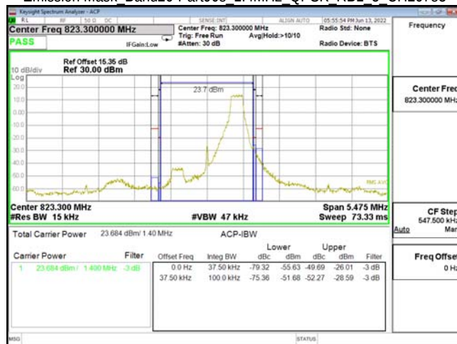
Emission Mask Band26-Part90s 1.4MHz QPSK RB1 5 CH26783
