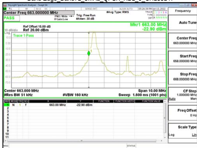
Band Edge Band71 5MHz QPSK RB1 0 CH133147
