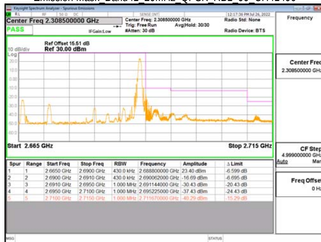
Emission Mask Band41 20MHz QPSK RB1 99 CH41490
