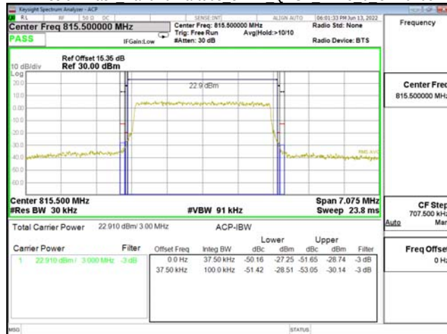
Emission Mask Band26-Part90s 3MHz QPSK RB15 0 CH26775
