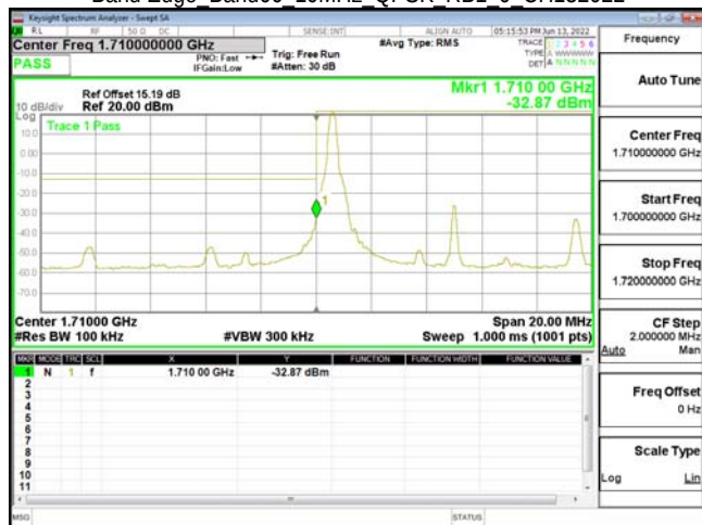
Band Edge Band66 10MHz QPSK RB1 0 CH132022
