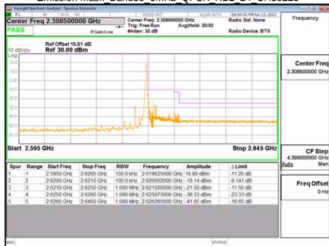
Emission Mask Band38 5MHz QPSK RB1 24 CH38225
