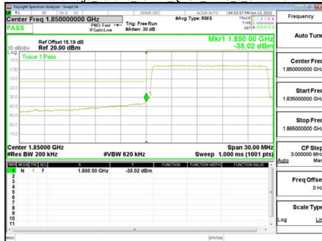
Band Edge Band25 15MHz QPSK RB75 0 CH26615
