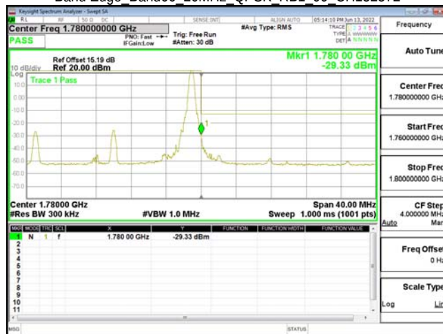
Band Edge Band66 20MHz QPSK RB1 99 CH132572
