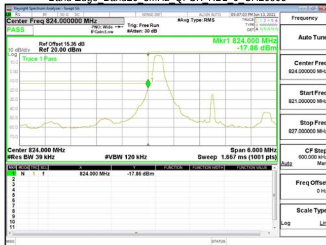
Band Edge Band26 3MHz QPSK RB1 0 CH26805
