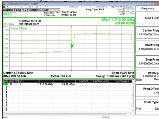
Band Edge Band66 5MHz QPSK RB25 0 CH132647
