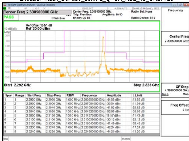
Emission Mask Band30 10MHz QPSK RB1 49 CH27710
