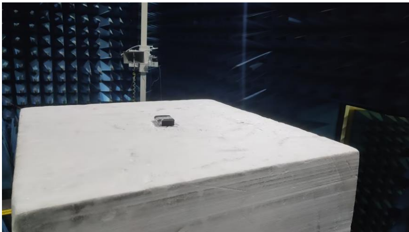
Radiated emissions spurious(Above 1GHz)
