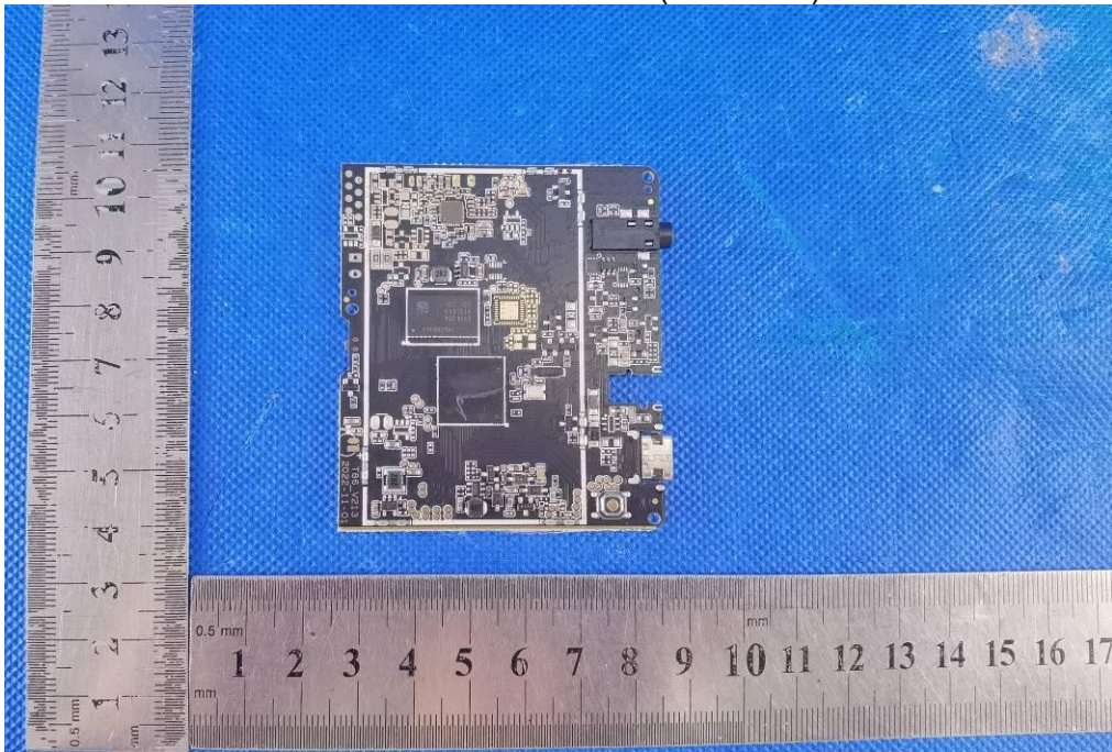
INTERNAL VIEW OF EUT(FIGURE 7)
