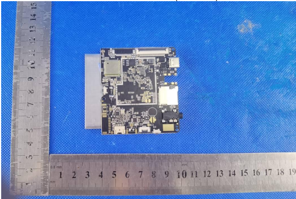
INTERNAL VIEW OF EUT(FIGURE 5)
