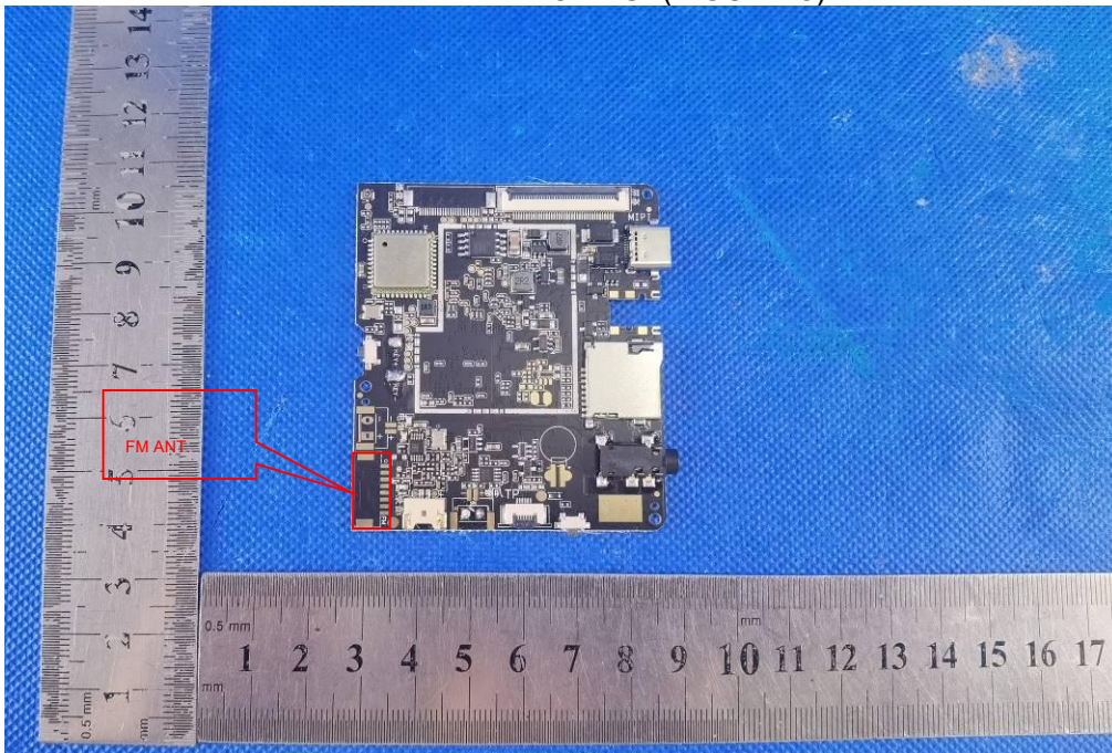
INTERNAL VIEW OF EUT(FIGURE 8)
