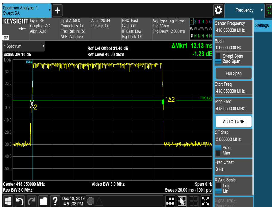
Figure 64 - Burst Length
