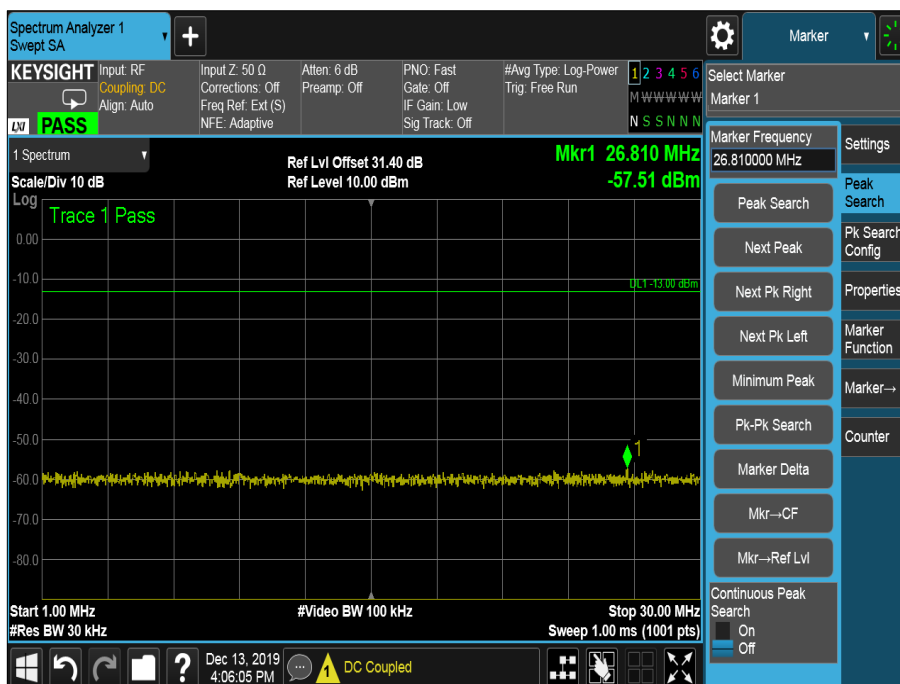
Figure 18 - 469.975 MHz - 1 MHz to 30 MHz
