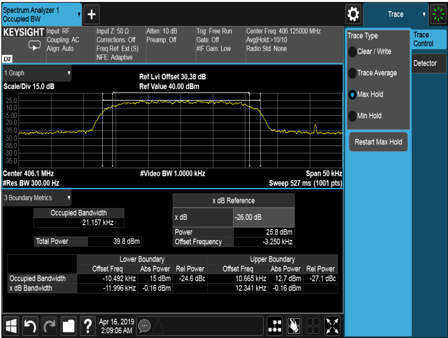
Figure 4 - 406.125 MHz Occupied Bandwidth
