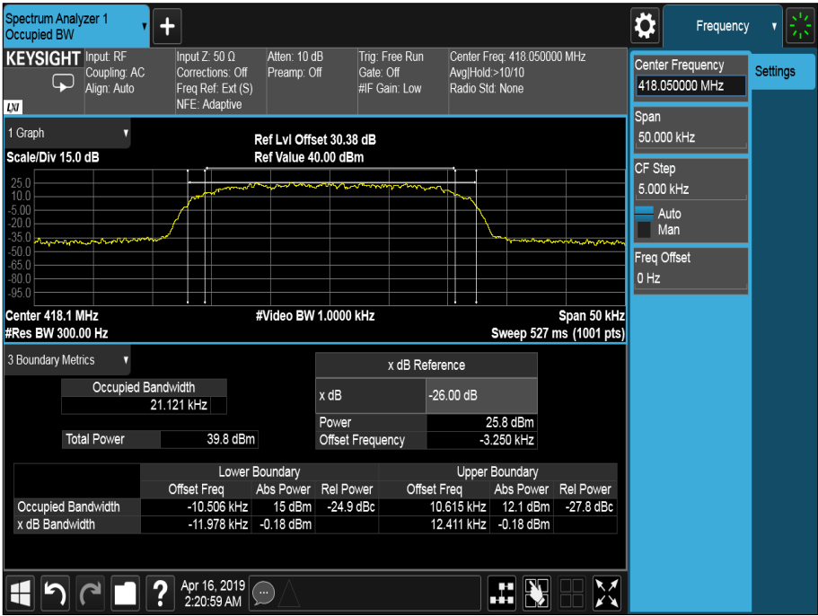
Figure 5 - 418.050 MHz Occupied Bandwidth
