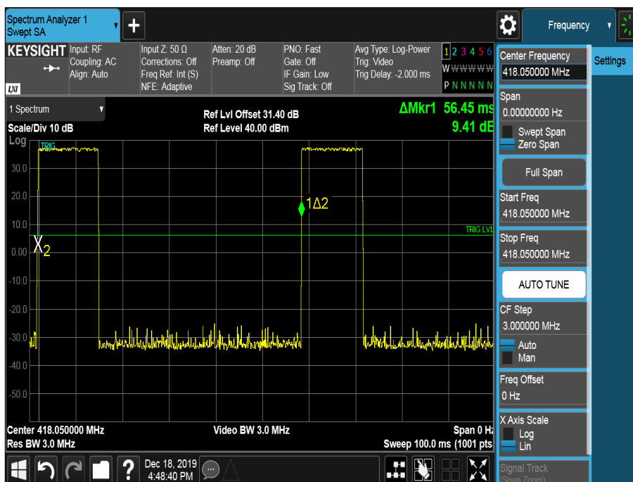
Figure 65 - Burst Period
