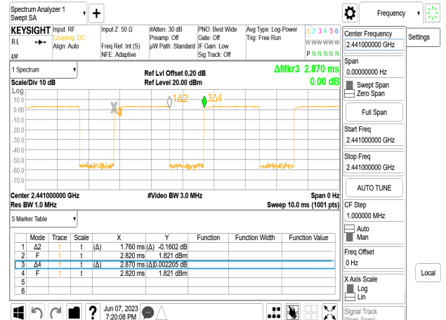
Dwell Time_π/4DQPSK_2M_DH5_2441MHz
