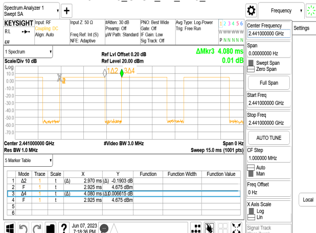
Dwell Time_GFSK_1M_DH5_2441MHz
