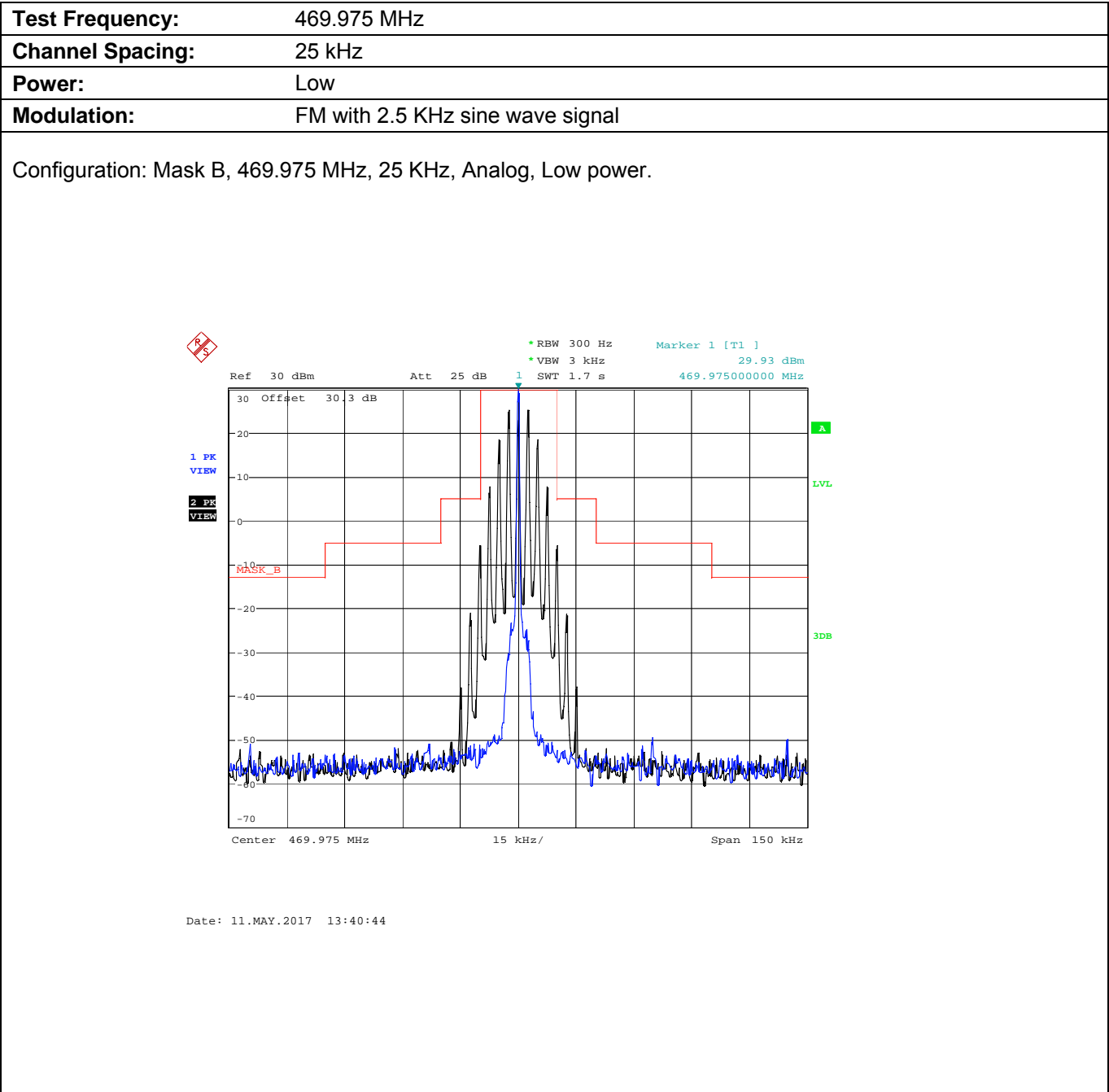
Plot 5.8.4.4.6. Emission Mask B, Low Power
