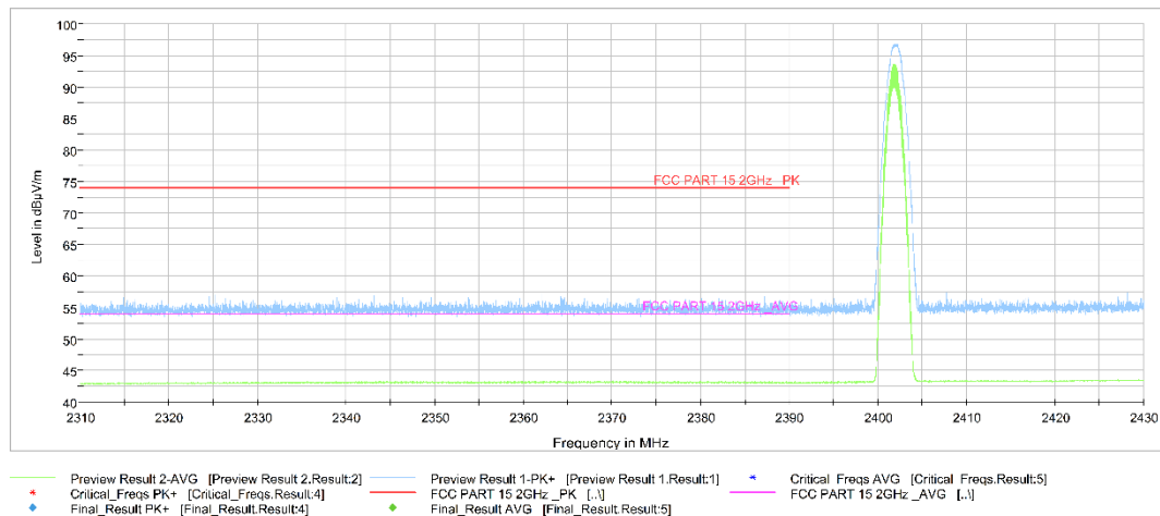
Fig.15. Frequency Band Edges: \pi/4 DQPSK, Channel 0, Hopping Off, 2.31 GHz - 2.43GHz
