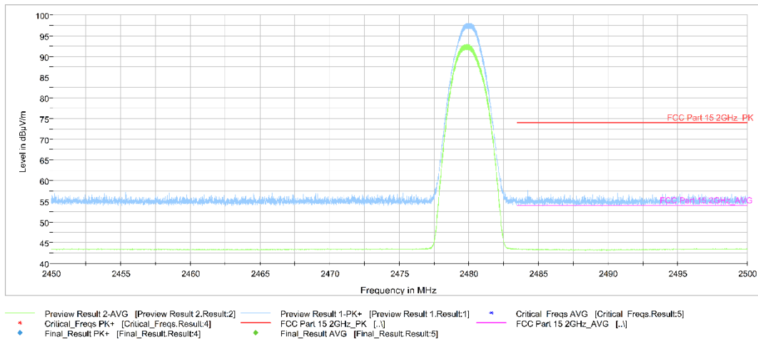
Fig.18. Frequency Band Edges: 8DPSK, Channel 78, 2.45 GHz - 2.50GHz
