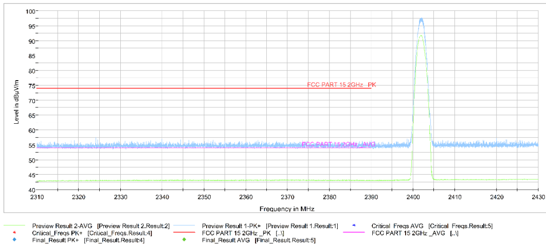
Fig.17. Frequency Band Edges: 8DPSK, Channel 0, 2.31 GHz - 2.43GHz
