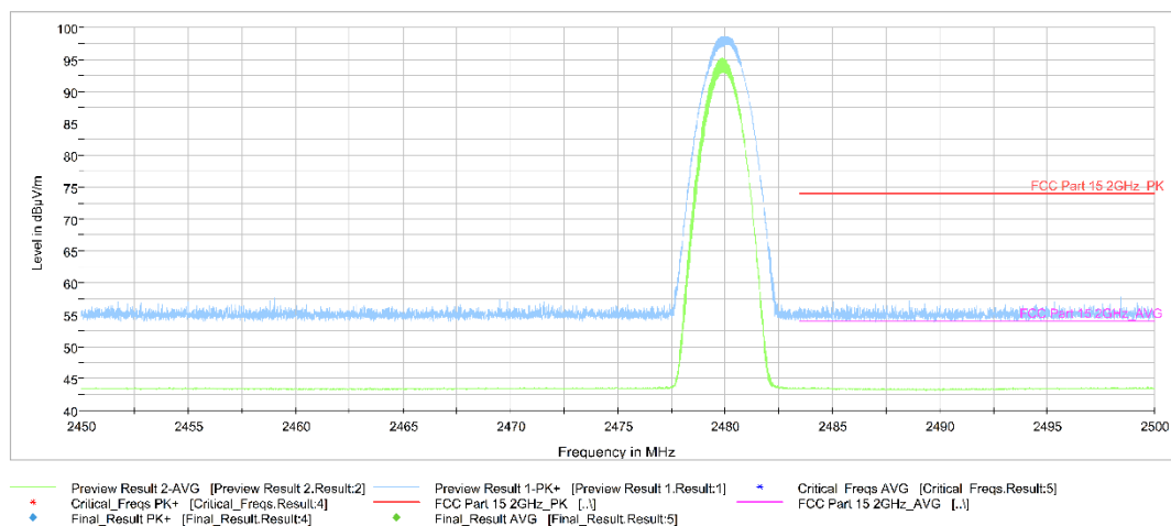
Fig.16. Frequency Band Edges: \pi/4 DQPSK, Channel 78, Hopping Off, 2.45 GHz - 2.50GHz
