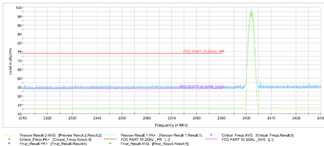
Fig.13. Frequency Band Edges: GFSK, Channel 0, Hopping Off, 2.31 GHz – 2.43GHz
