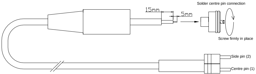
NAV-CABLE assembly detail
