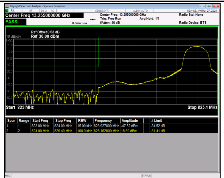
Band5_1.4MHz_16QAM_20407_1RB#5
