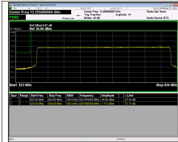
Band5_10MHz_64QAM_20450_50RB#0
