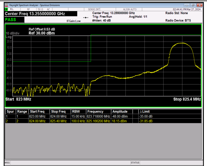
Band5_1.4MHz_64QAM_20407_1RB#5
