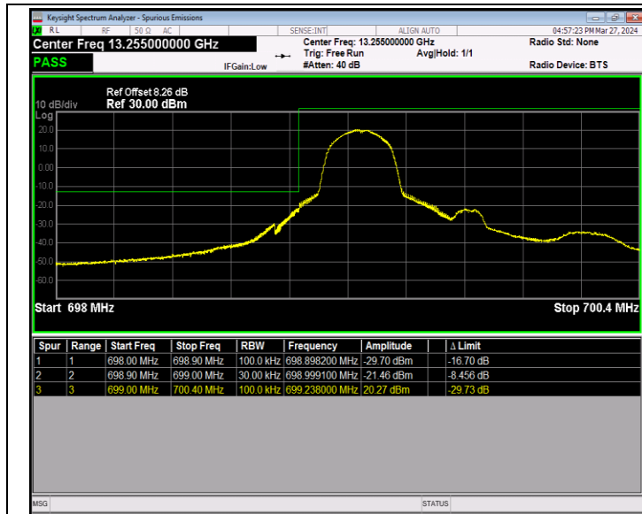
Band12_1.4MHz_QPSK_23017_1RB#0
