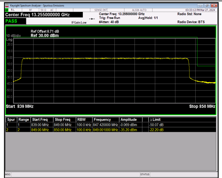
Band5_10MHz_16QAM_20600_50RB#0
