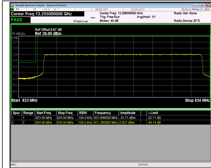
Band5_10MHz_QPSK_20450_50RB#0
