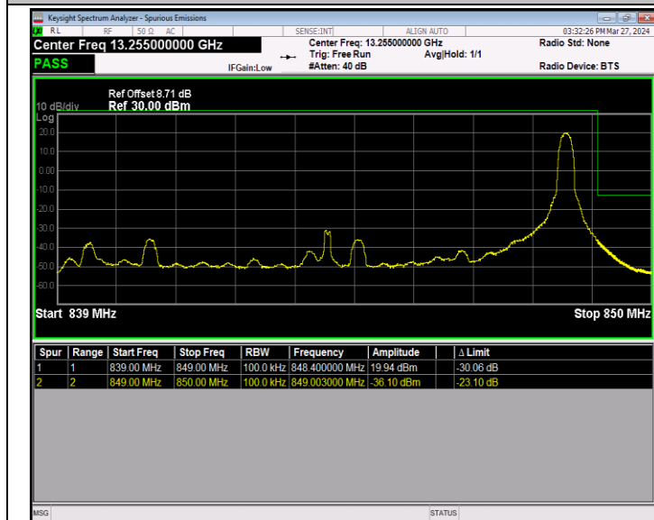
Band5_10MHz_QPSK_20600_1RB#49
