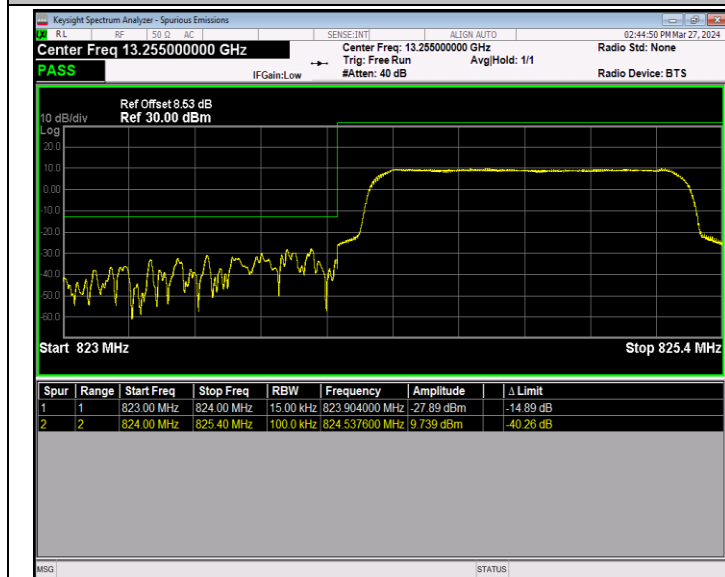
Band5_1.4MHz_QPSK_20407_6RB#0
