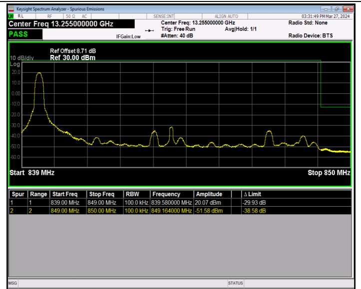
Band5_10MHz_QPSK_20600_1RB#0
