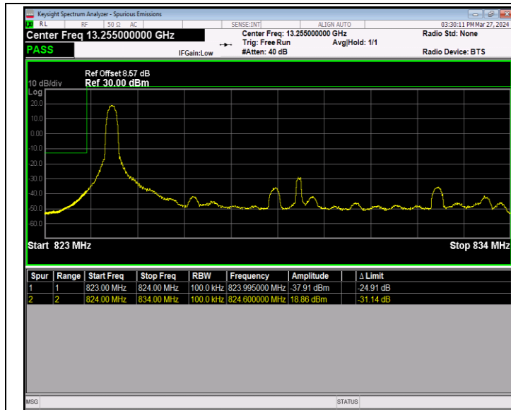
Band5_10MHz_16QAM_20450_1RB#0
