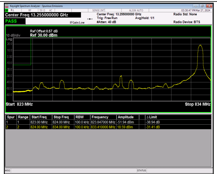
Band5_10MHz_16QAM_20450_1RB#49
