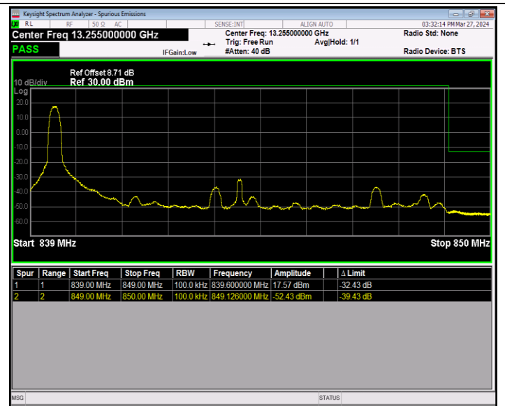
Band5_10MHz_64QAM_20600_1RB#0
