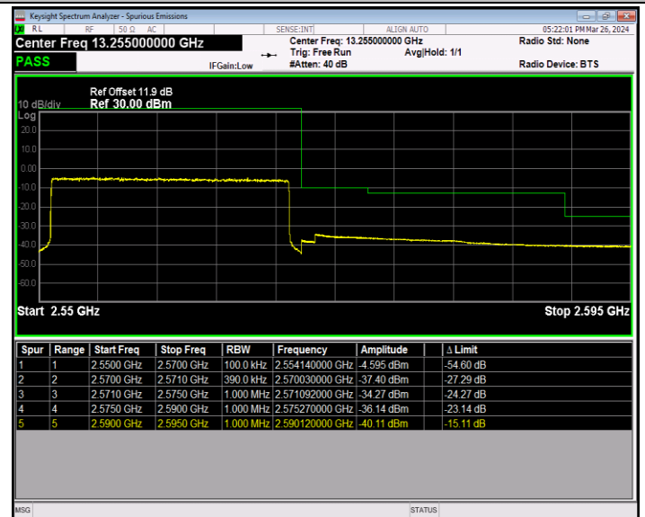
Band7_20MHz_64QAM_21350_100RB#0
