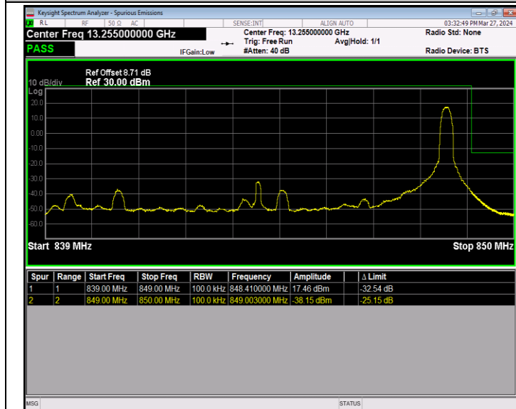
Band5_10MHz_64QAM_20600_1RB#49
