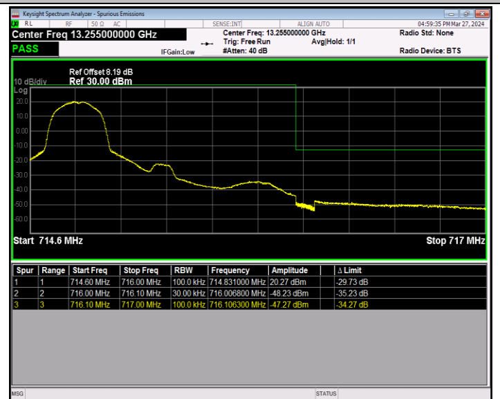
Band12_1.4MHz_QPSK_23173_1RB#0
