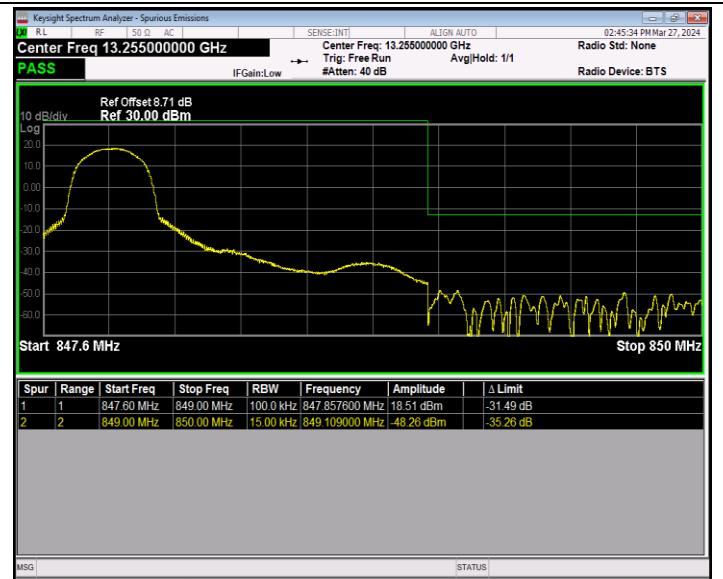
Band5_1.4MHz_16QAM_20643_1RB#0
