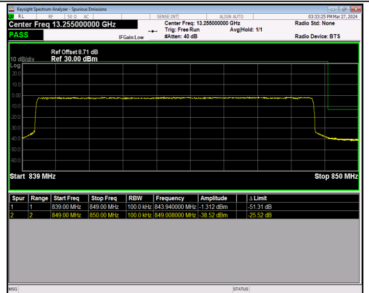
Band5_10MHz_64QAM_20600_50RB#0
