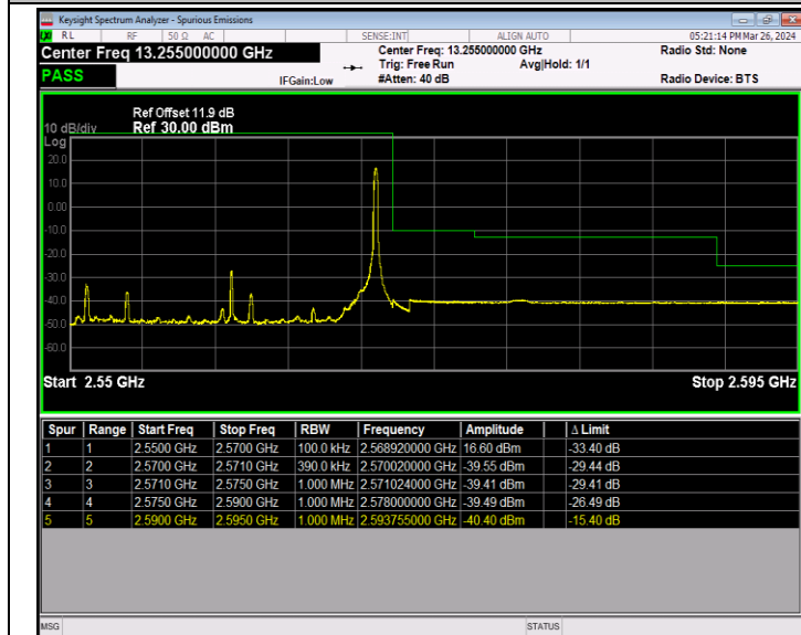
Band7_20MHz_64QAM_21350_1RB#99
