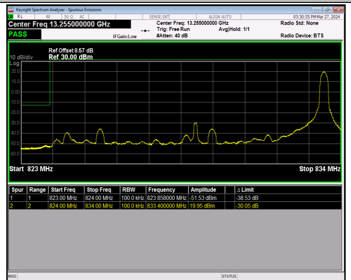
Band5_10MHz_QPSK_20450_1RB#49
