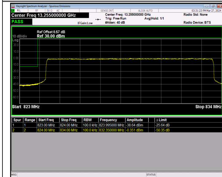
Band5_10MHz_16QAM_20450_50RB#0
