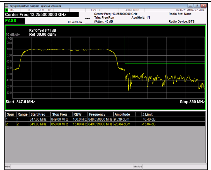
Band5_1.4MHz_QPSK_20643_6RB#0
