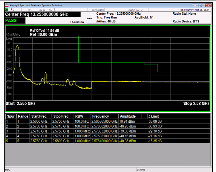
Band7_5MHz_64QAM_21425_1RB#0
