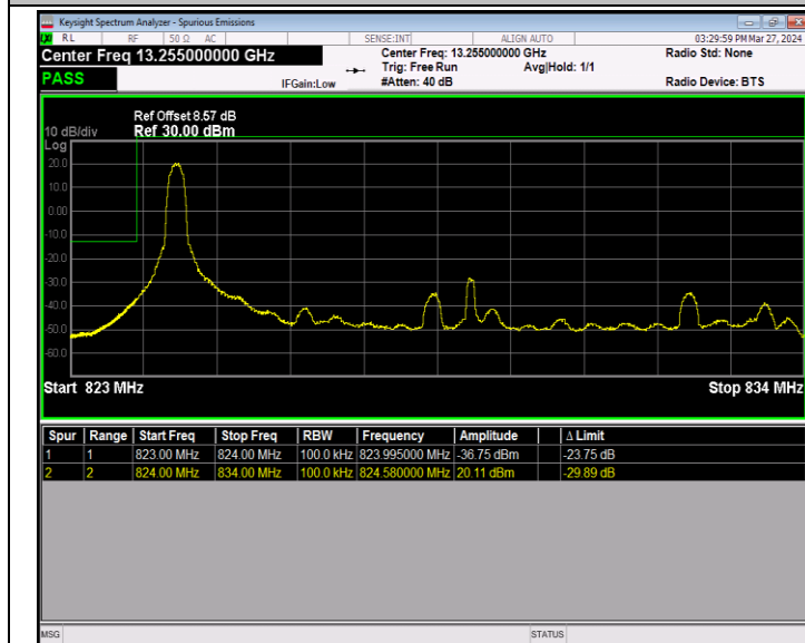
Band5_10MHz_QPSK_20450_1RB#0
