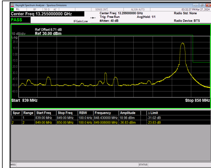
Band5_10MHz_16QAM_20600_1RB#49
