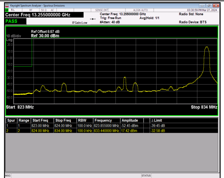
Band5_10MHz_64QAM_20450_1RB#49
