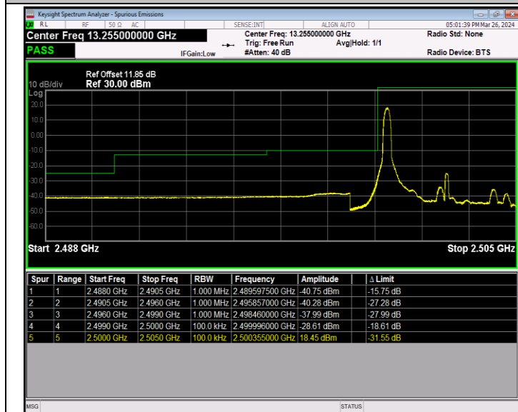
Band7_5MHz_16QAM_20775_1RB#0
