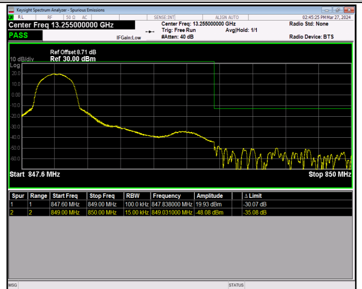
Band5_1.4MHz_QPSK_20643_1RB#0
