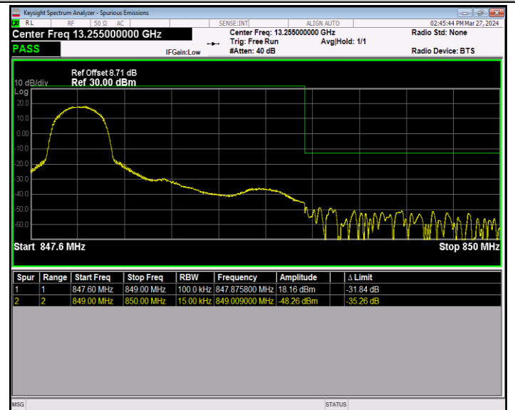
Band5_1.4MHz_64QAM_20643_1RB#0
