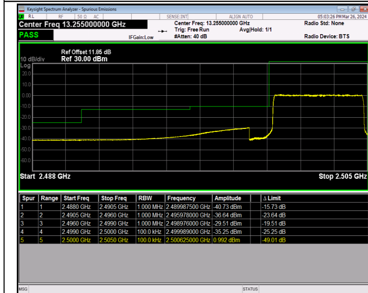
Band7_5MHz_64QAM_20775_25RB#0
