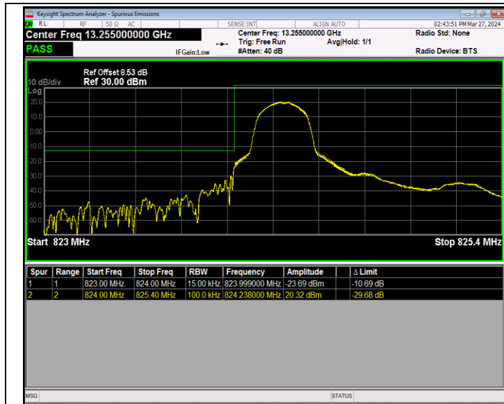
Band5_1.4MHz_QPSK_20407_1RB#0
