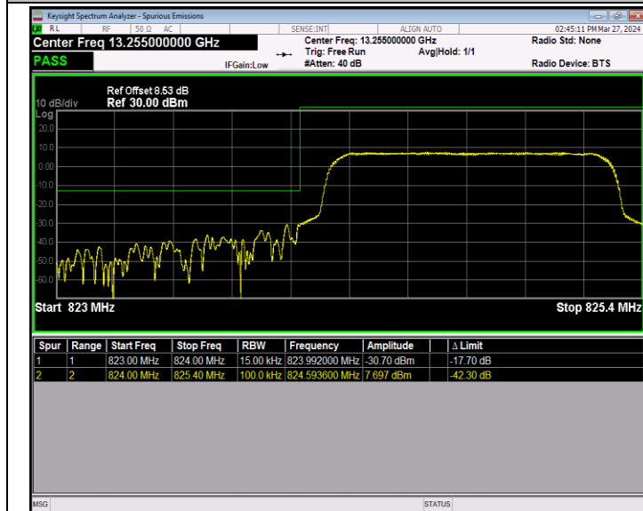
Band5_1.4MHz_64QAM_20407_6RB#0
