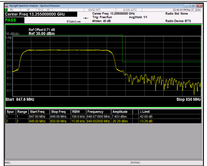
Band5_1.4MHz_64QAM_20643_6RB#0
