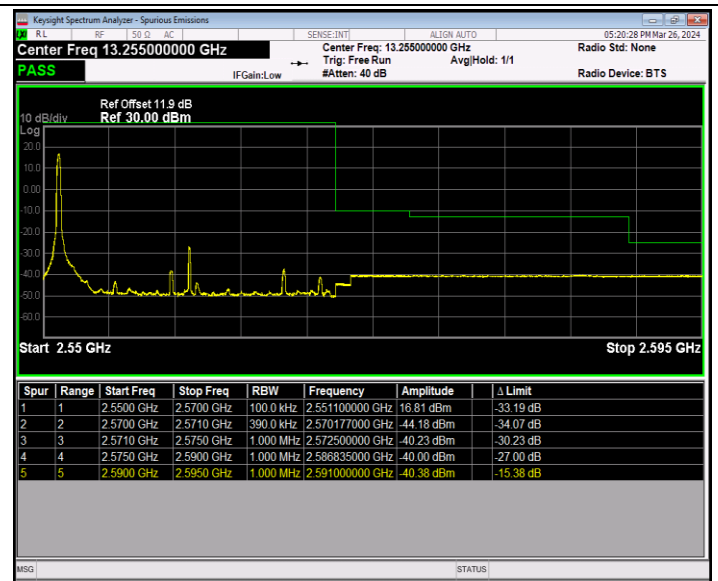
Band7_20MHz_64QAM_21350_1RB#0
