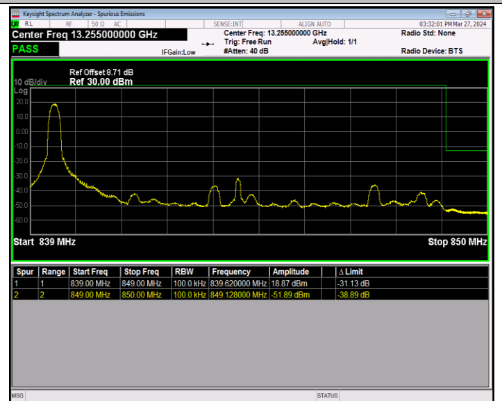
Band5_10MHz_16QAM_20600_1RB#0
