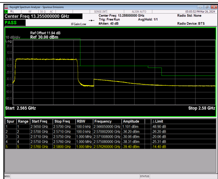
Band7_5MHz_64QAM_21425_25RB#0
