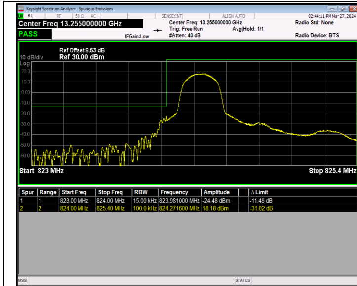
Band5_1.4MHz_64QAM_20407_1RB#0
