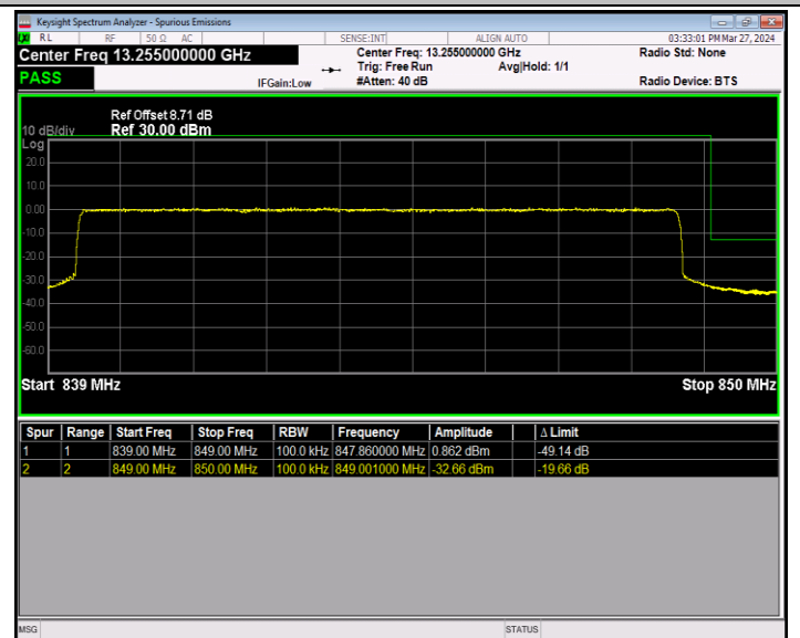
Band5_10MHz_QPSK_20600_50RB#0
