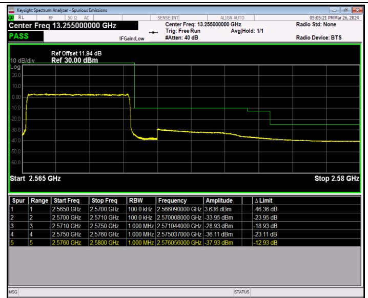
Band7_5MHz_QPSK_21425_25RB#0
