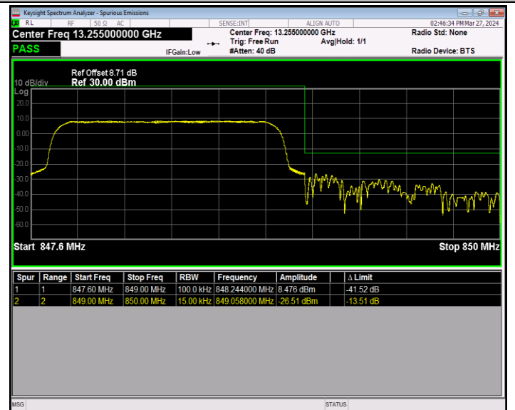
Band5_1.4MHz_16QAM_20643_6RB#0
