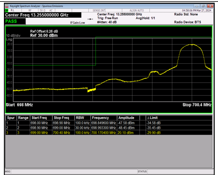
Band12_1.4MHz_QPSK_23017_1RB#5
