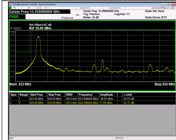
Band5_10MHz_64QAM_20450_1RB#0
