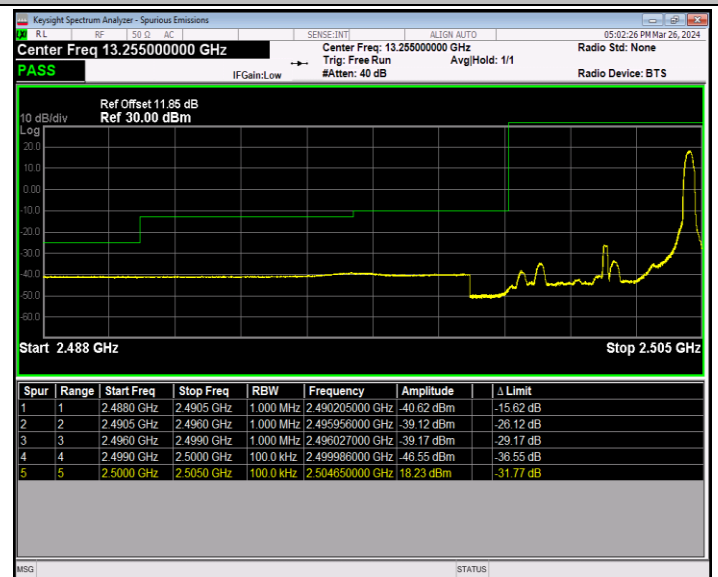
Band7_5MHz_16QAM_20775_1RB#24
