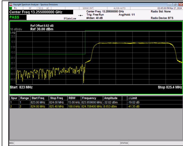
Band5_1.4MHz_16QAM_20407_6RB#0
