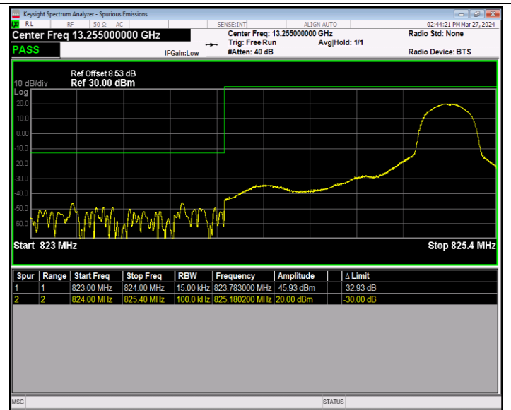
Band5_1.4MHz_QPSK_20407_1RB#5
