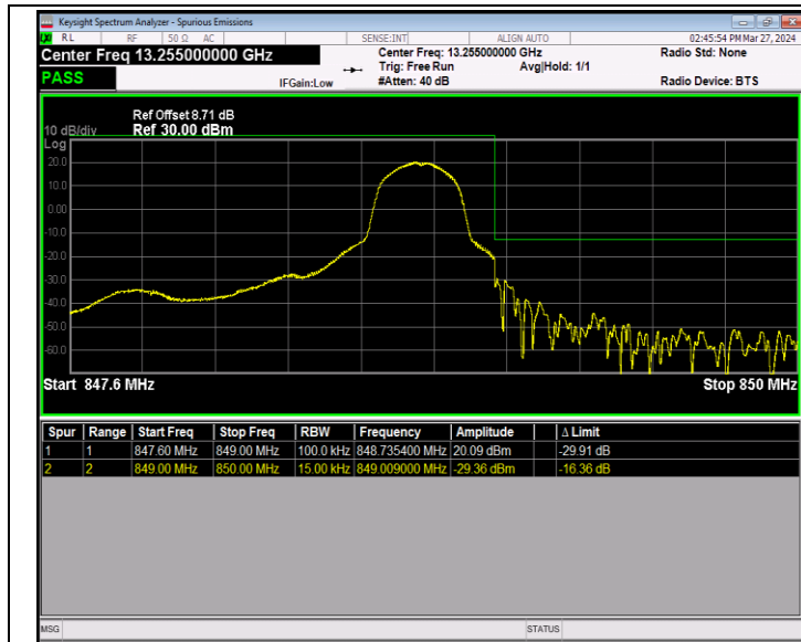
Band5_1.4MHz_QPSK_20643_1RB#5
