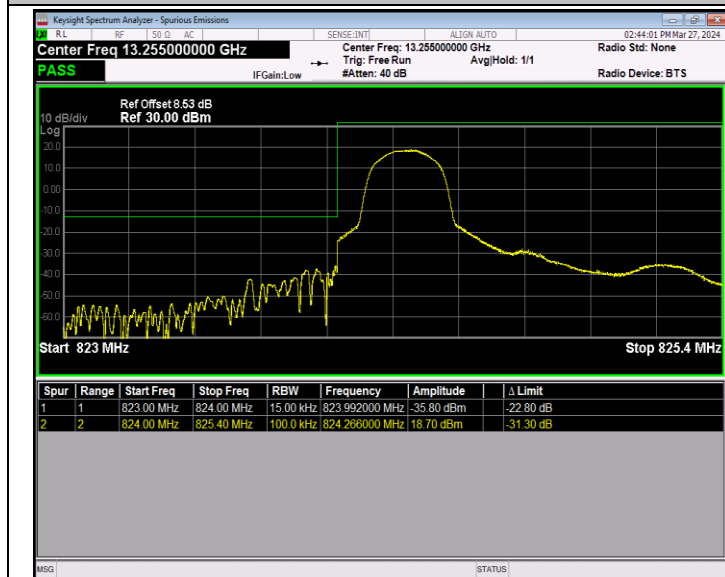
Band5_1.4MHz_16QAM_20407_1RB#0
