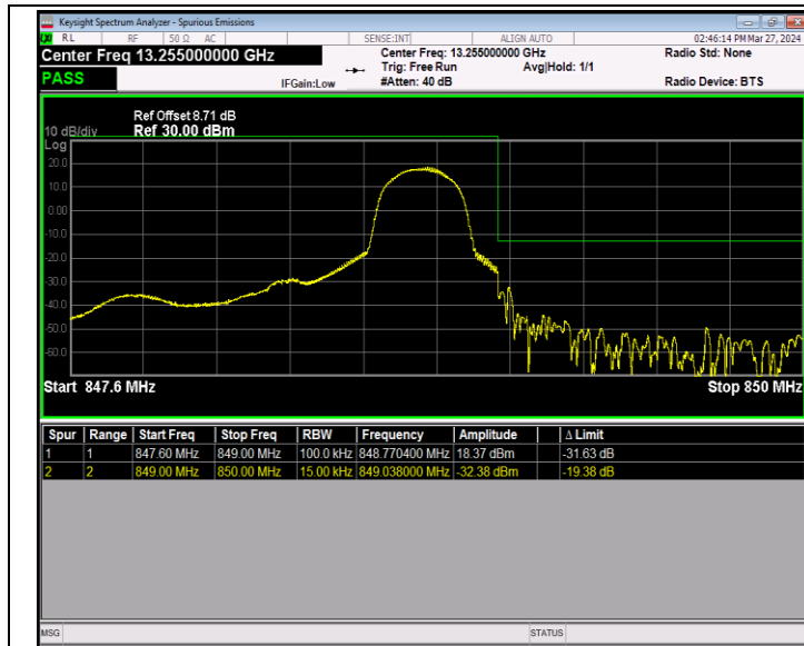
Band5_1.4MHz_64QAM_20643_1RB#5
