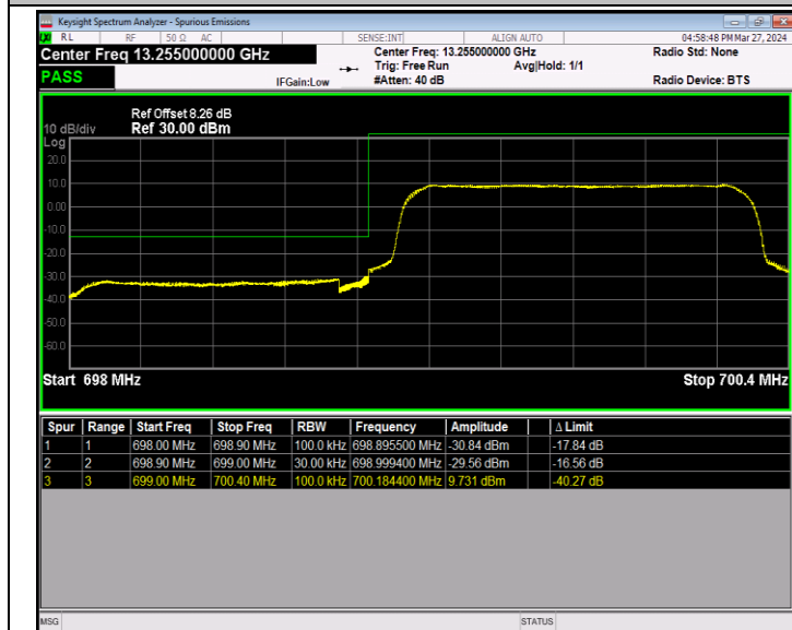
Band12_1.4MHz_QPSK_23017_6RB#0
