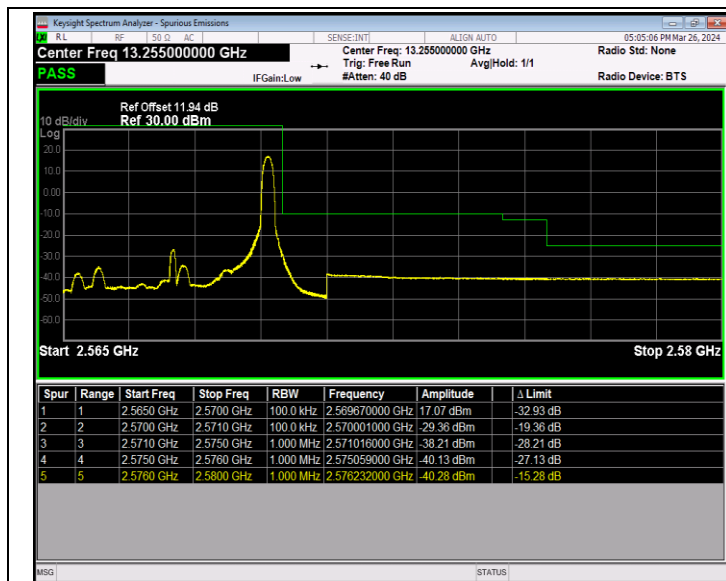
Band7_5MHz_64QAM_21425_1RB#24
