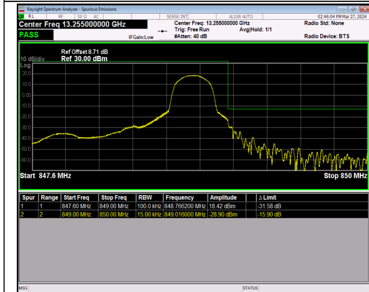
Band5_1.4MHz_16QAM_20643_1RB#5
