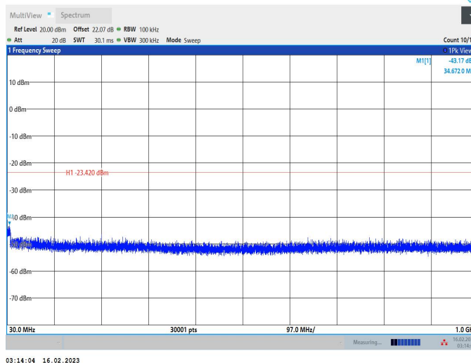
BLE_1M_Ant1_2440_30~1000
