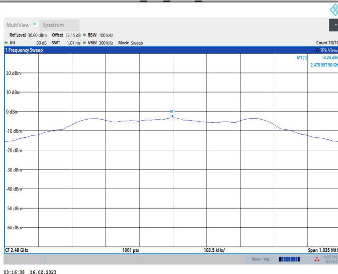
BLE_1M_Ant1_2480
