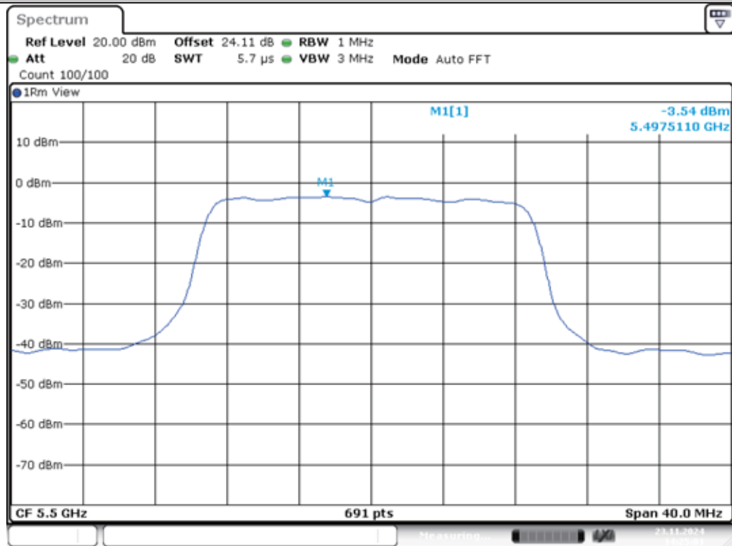
11N20MIMO-Ant1-5500-PASS
