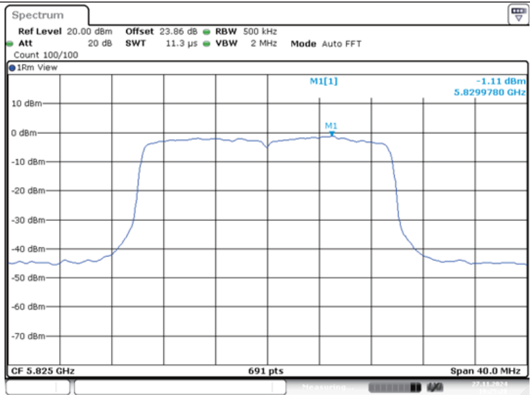
11AX20MIMO-Ant1-5825-PASS
