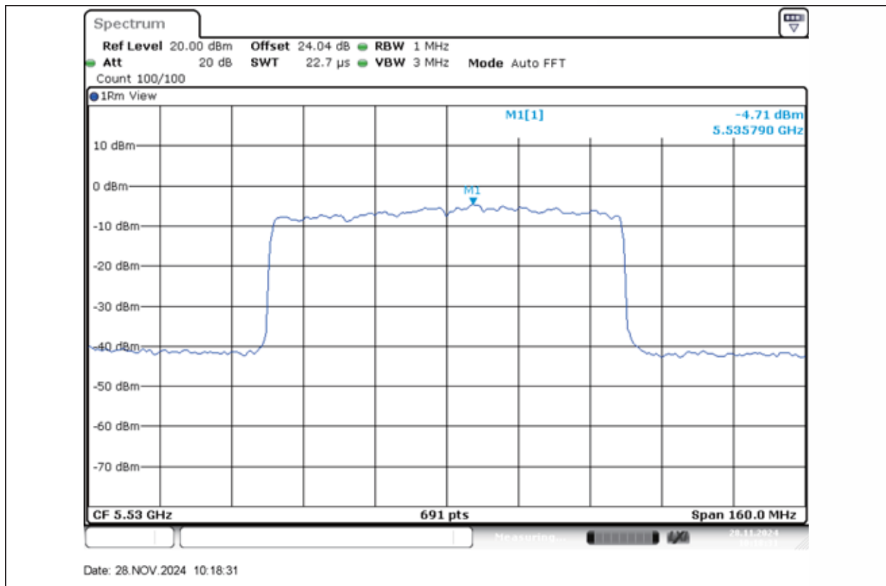
11AX80MIMO-Ant1-5530-PASS
