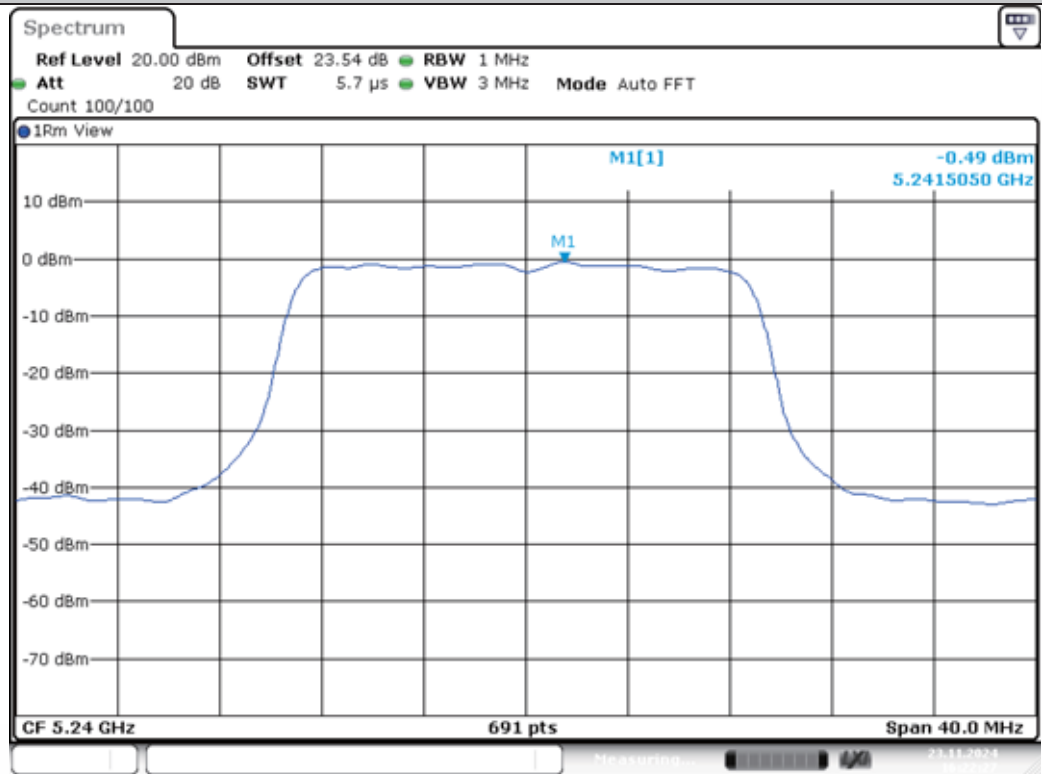
11AC20MIMO-Ant1-5240-PASS
