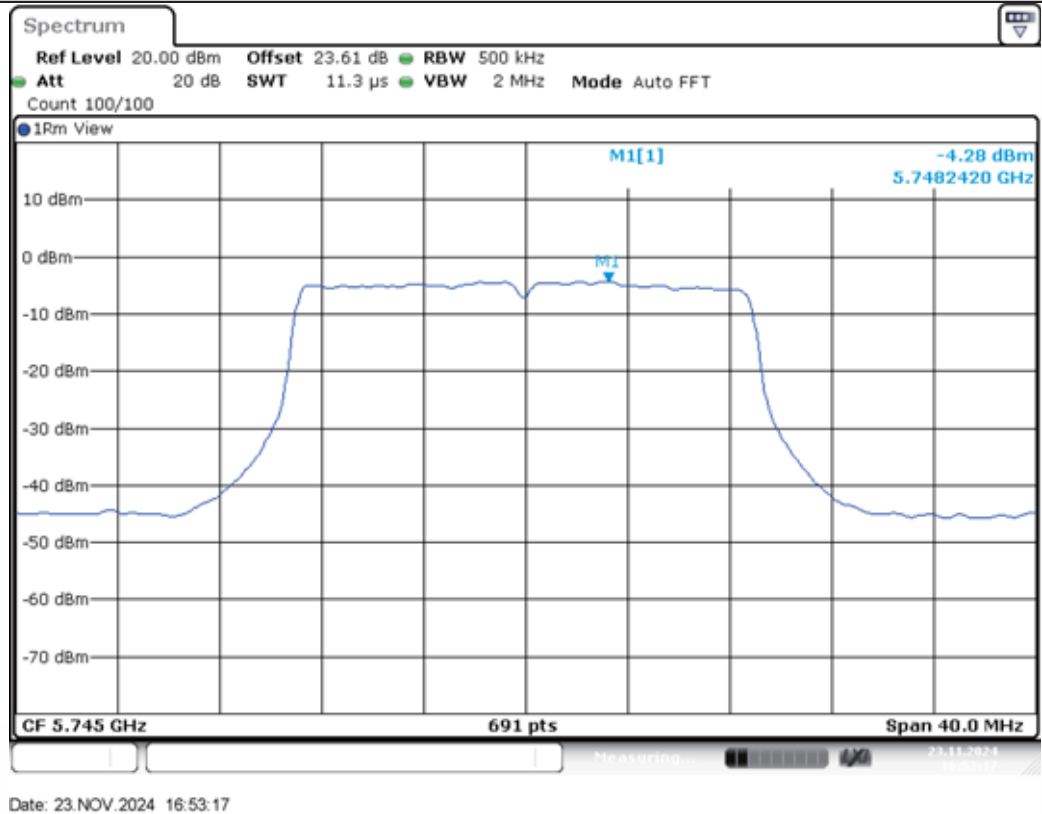
11AC20MIMO-Ant2-5745-PASS
