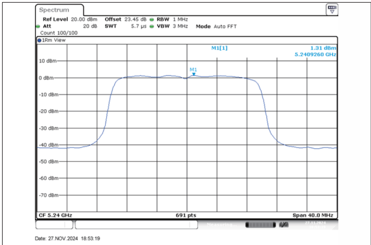
11AX20MIMO-Ant1-5240-PASS
