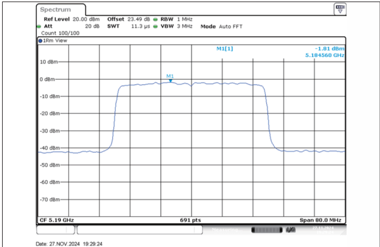
11AX40MIMO-Ant1-5190-PASS
