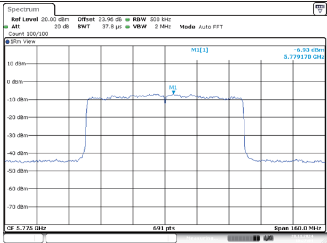
11AX80MIMO-Ant1-5775-PASS
