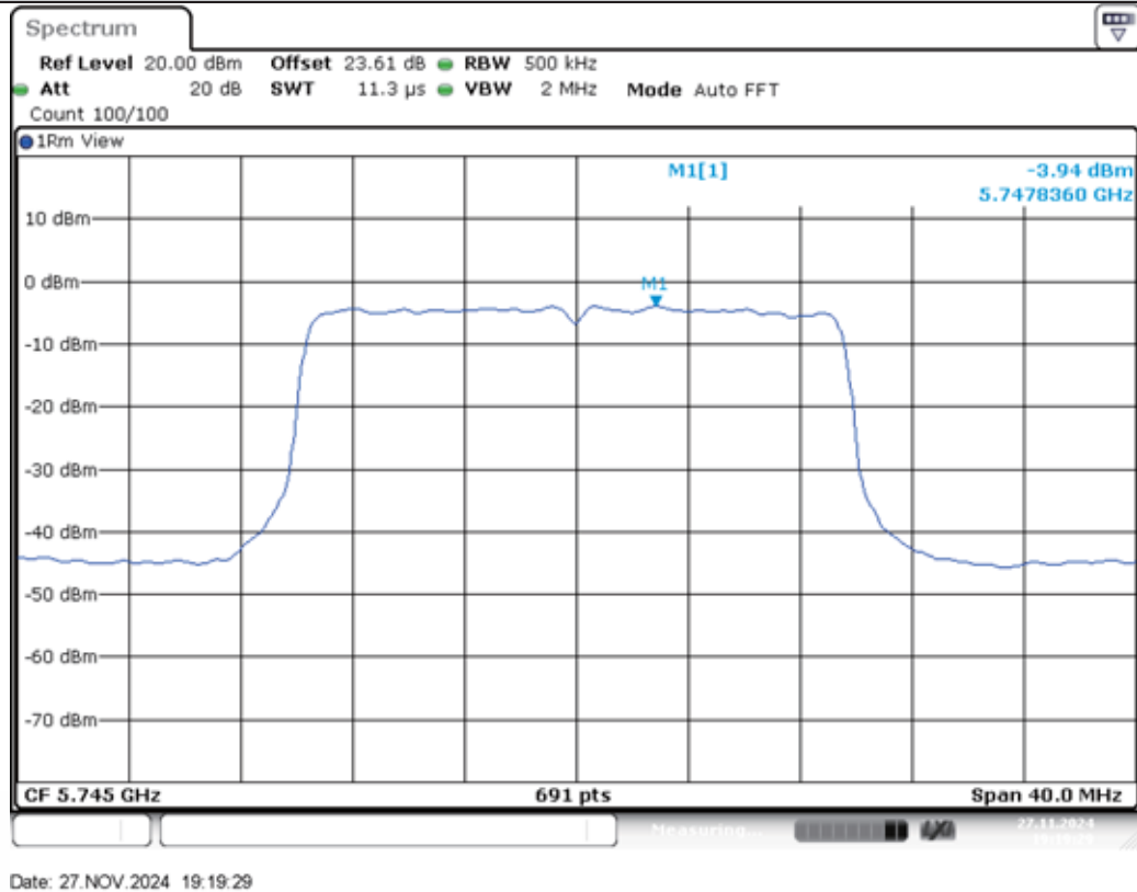
11AX20MIMO-Ant2-5745-PASS
