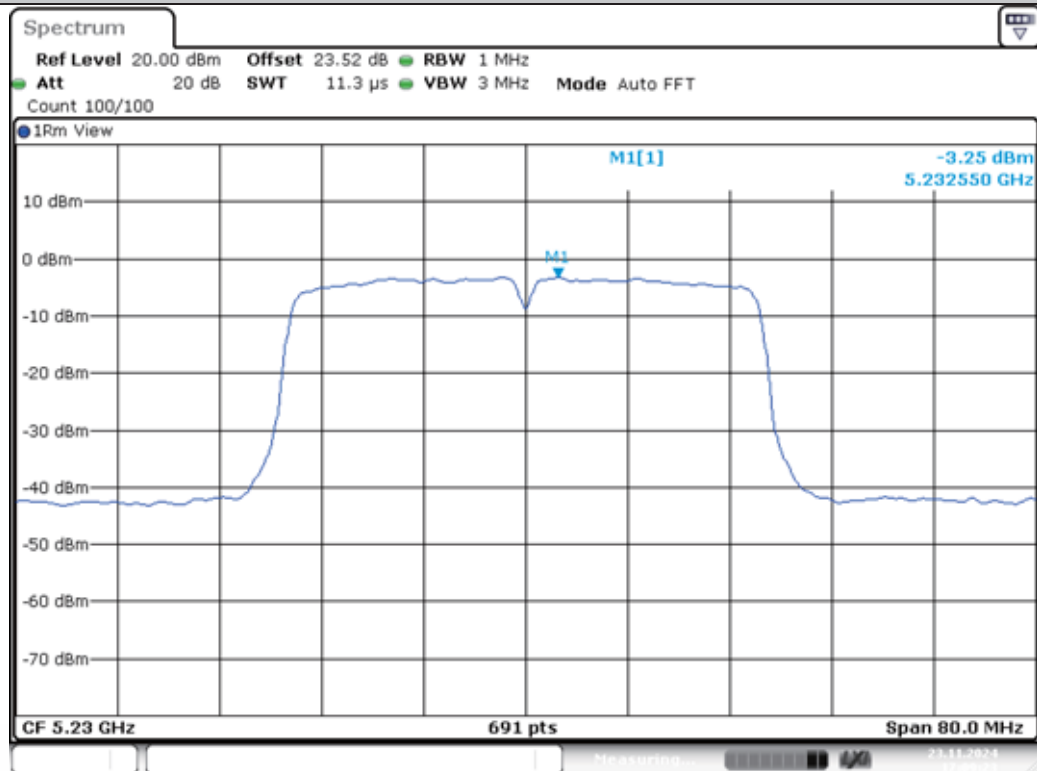
11AC40MIMO-Ant1-5230-PASS
