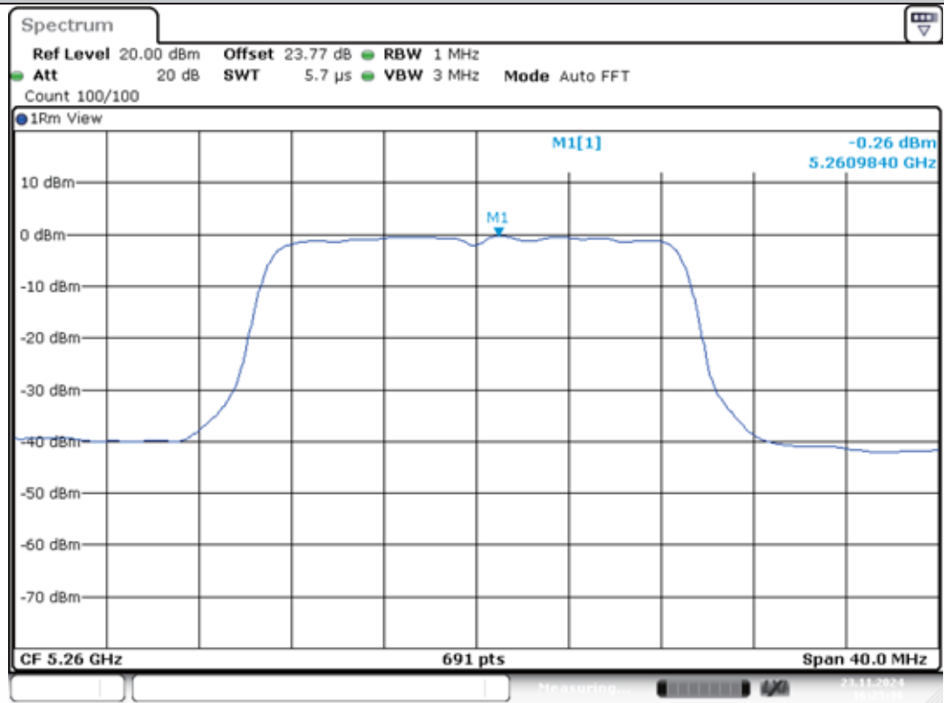
11AC20MIMO-Ant1-5260-PASS
