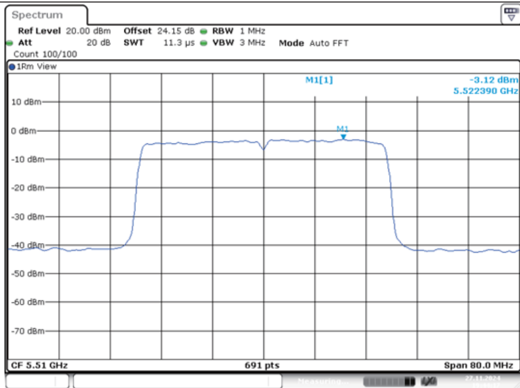
11AX40MIMO-Ant1-5510-PASS
