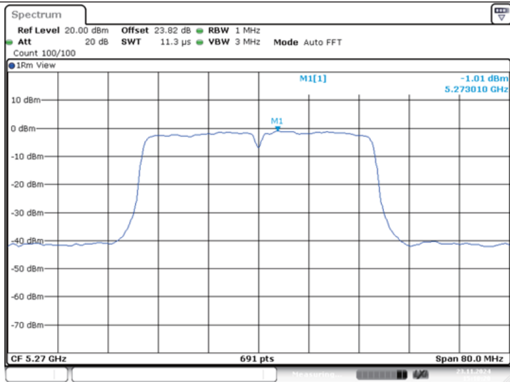
11N40MIMO-Ant1-5270-PASS
