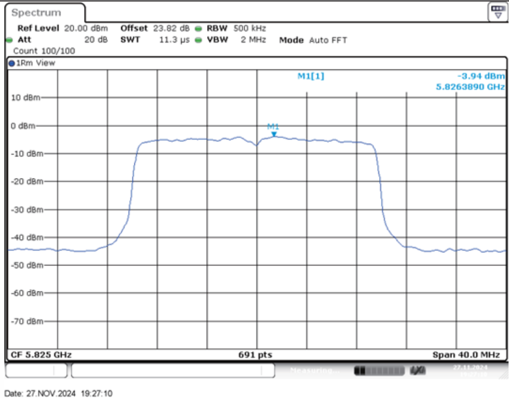
11AX20MIMO-Ant2-5825-PASS
