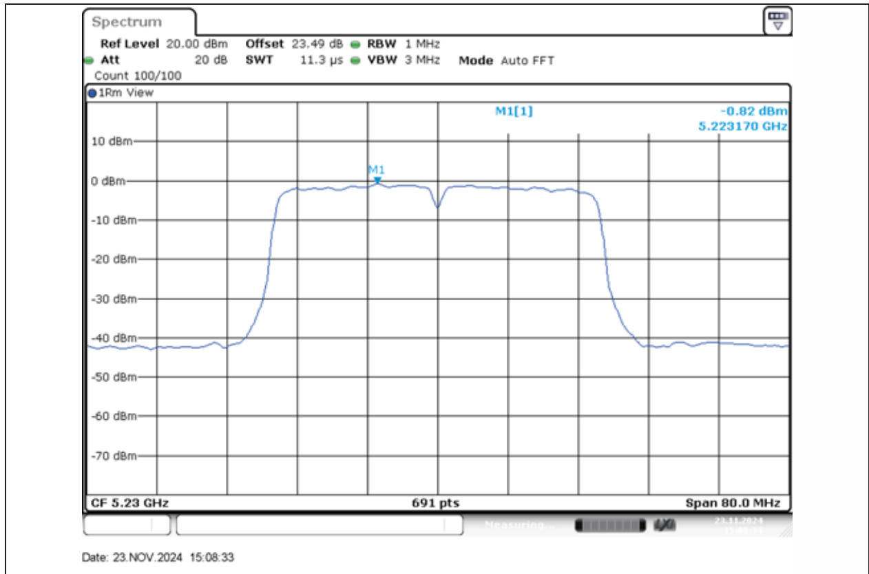
11N40MIMO-Ant1-5230-PASS
