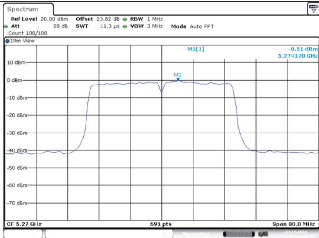
11AC40MIMO-Ant1-5270-PASS
