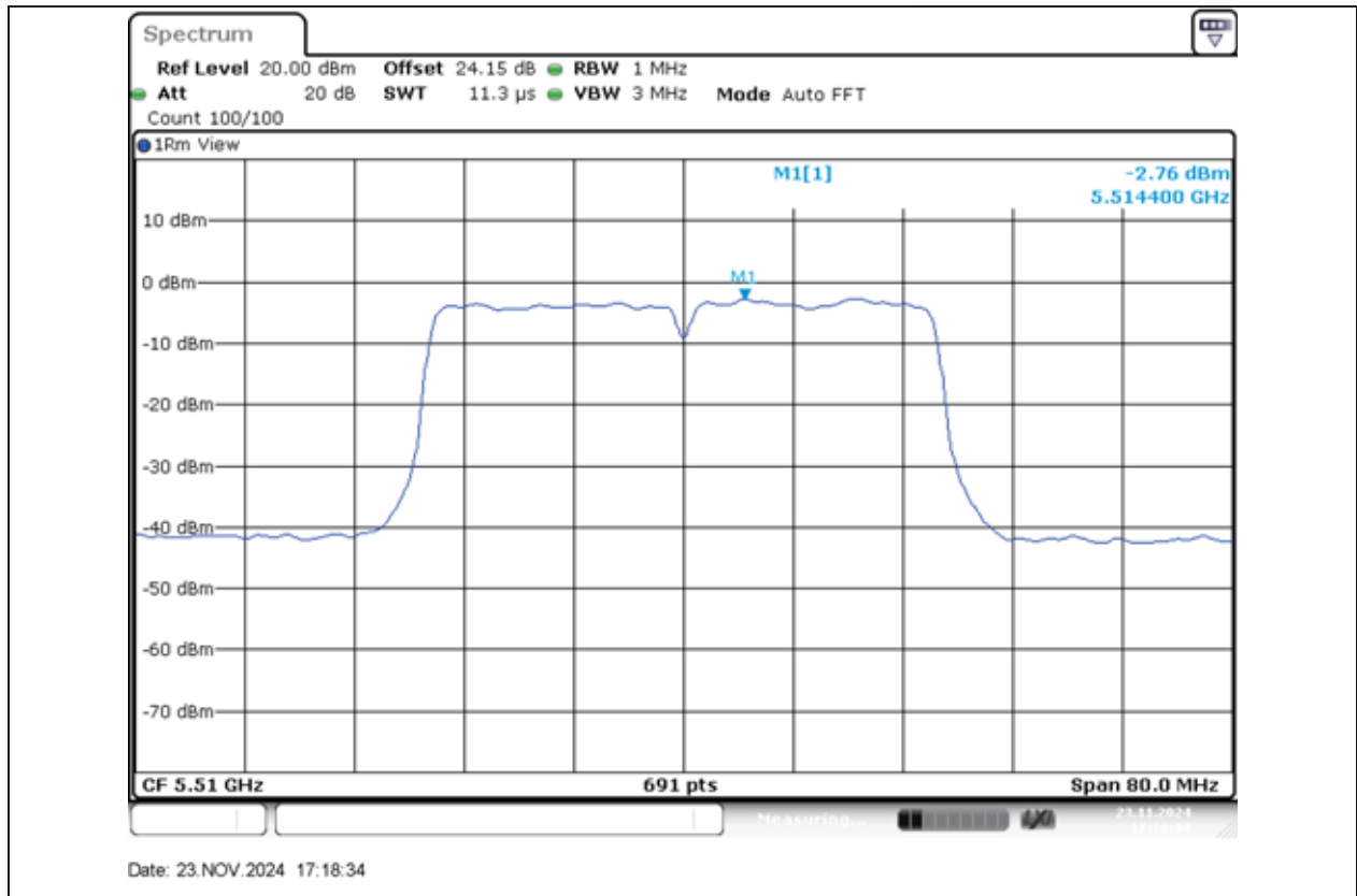
11AC40MIMO-Ant1-5510-PASS
