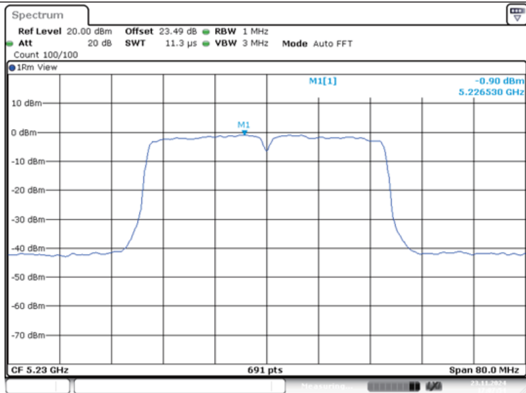
11AC40MIMO-Ant1-5230-PASS
