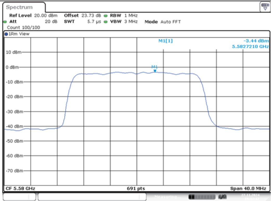
11AX20MIMO-Ant1-5580-PASS
