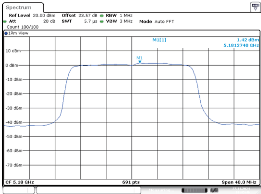
11AX20MIMO-Ant1-5180-PASS
