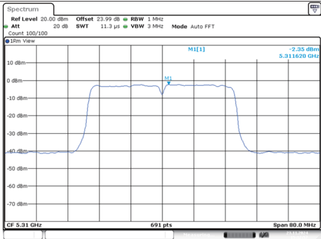
11N40MIMO-Ant1-5310-PASS
