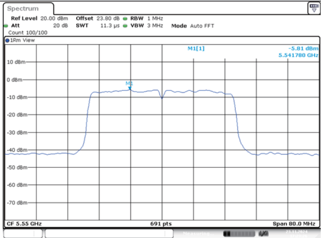
11AC40MIMO-Ant1-5550-PASS
