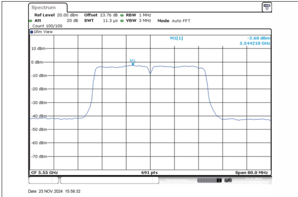
11N40MIMO-Ant1-5550-PASS
