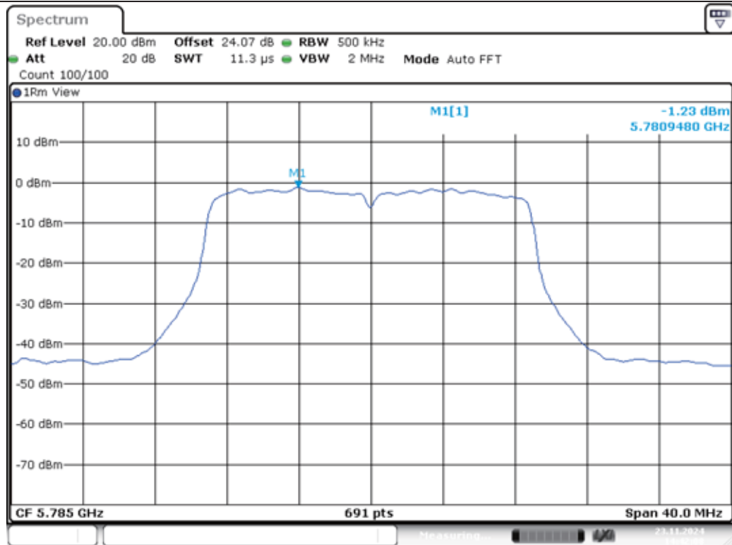
11N20MIMO-Ant1-5785-PASS
