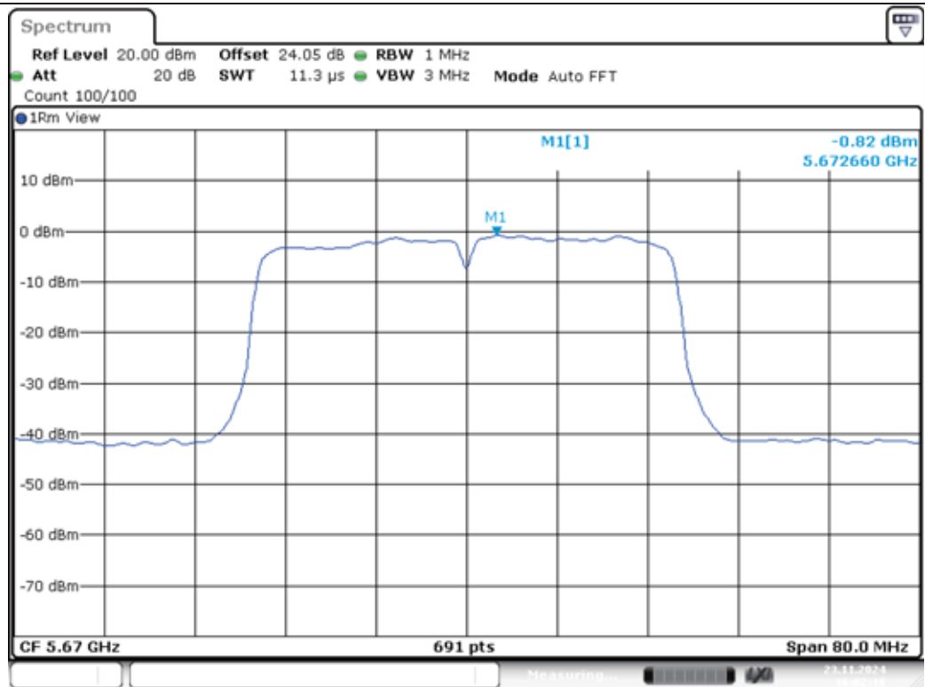
11N40MIMO-Ant1-5670-PASS
