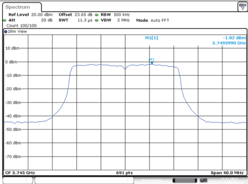
11AC20MIMO-Ant1-5745-PASS
