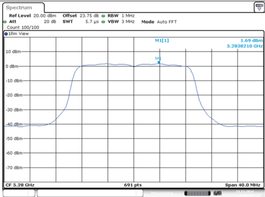
11AC20MIMO-Ant1-5280-PASS
