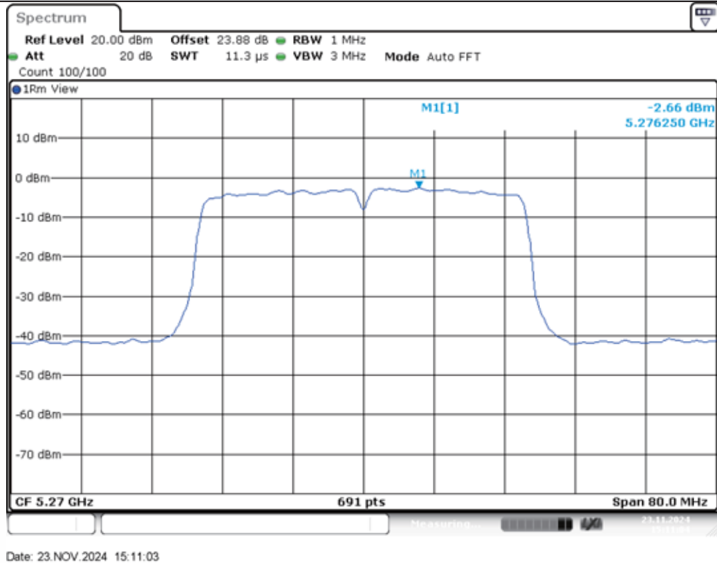
11N40MIMO-Ant2-5270-PASS
