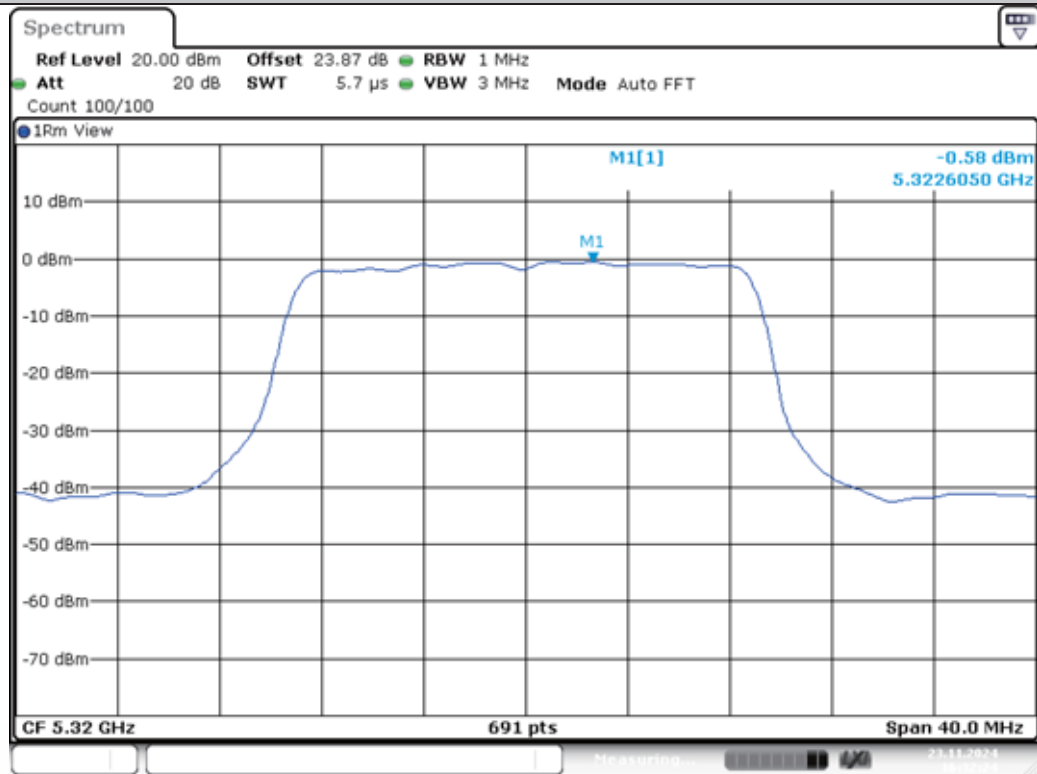
11AC20MIMO-Ant1-5320-PASS
