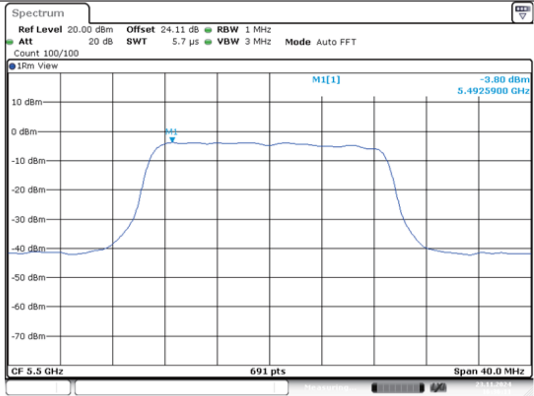
11AC20MIMO-Ant1-5500-PASS
