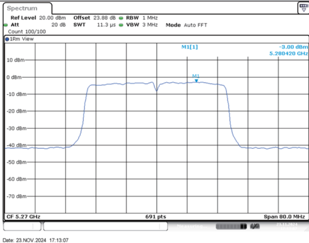
11AC40MIMO-Ant2-5270-PASS
