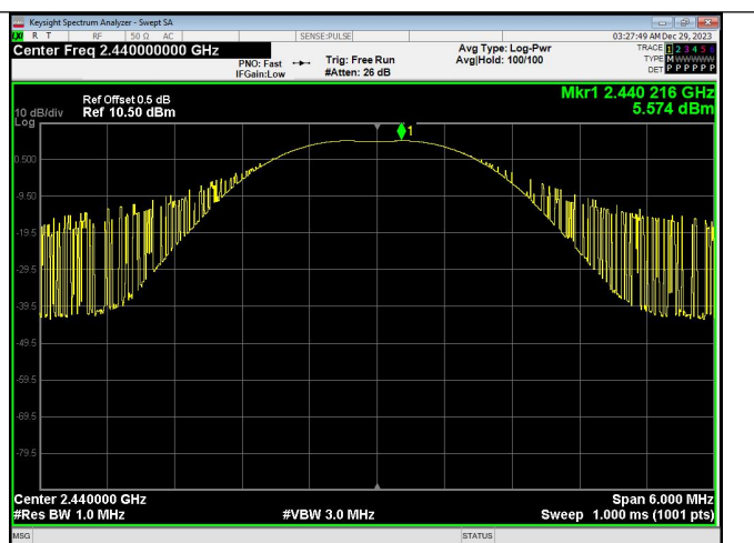
Peak Output Power LE_Channel 19
