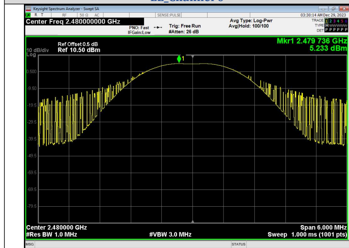
Peak Output Power LE_Channel 39
