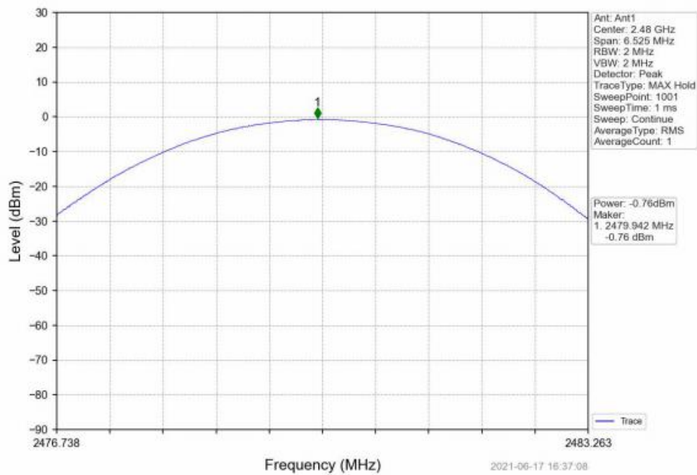
8DPSK_3DH5_HCH_2480MHz_Ant1_NTNV
