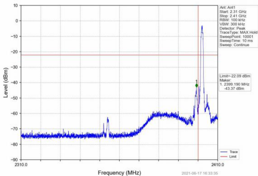
8DPSK_3DH5_LCH_2402MHz_Ant1_NTNV
