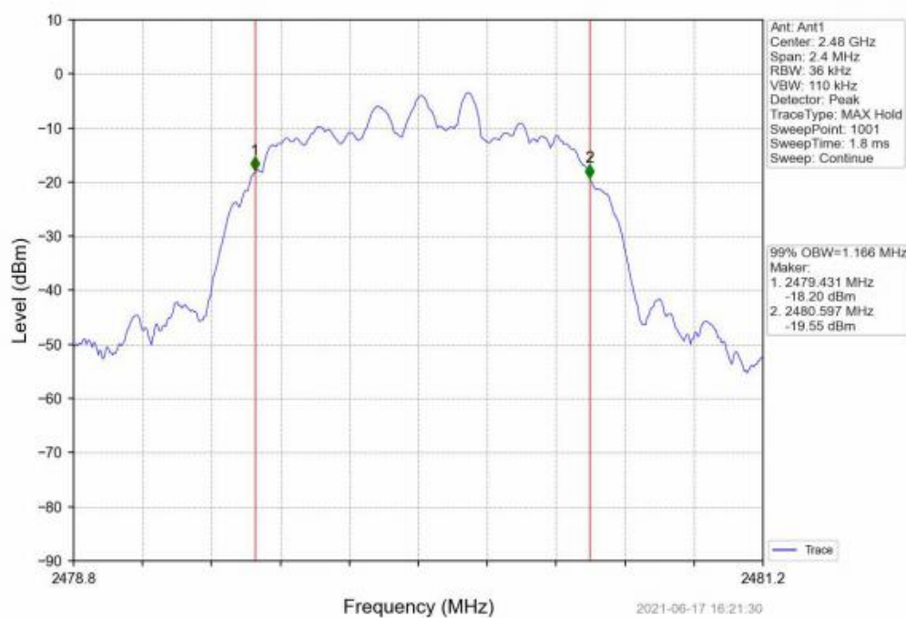
\pi/4 -DQPSK_2DH5_HCH_2480MHz_Ant1_NTNV
