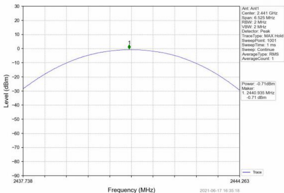
8DPSK_3DH5_MCH_2441MHz_Ant1_NTNV
