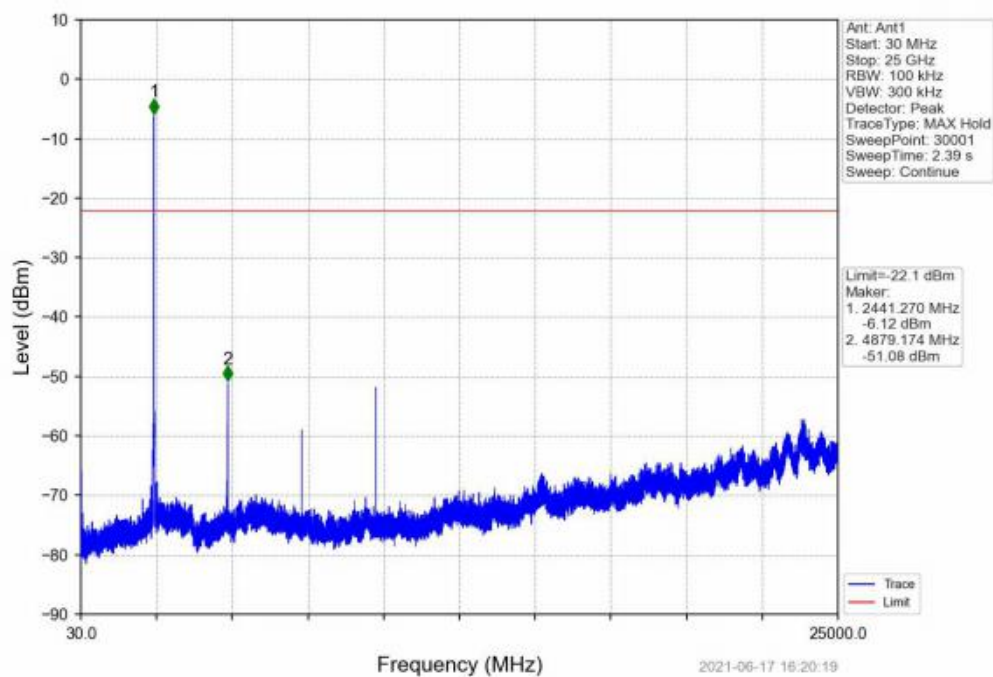
\pi /4-DQPSK_2DH5_MCH_2441MHz_Ant1_NTNV
