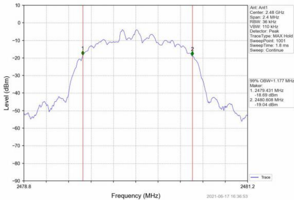
8DPSK_3DH5_HCH_2480MHz_Ant1_NTNV
