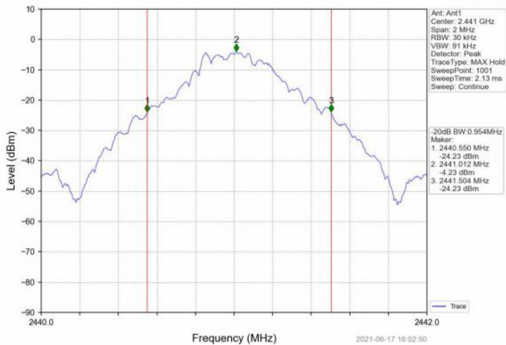
GFSK_DH5_MCH_2441MHz_Ant1_NTNV
