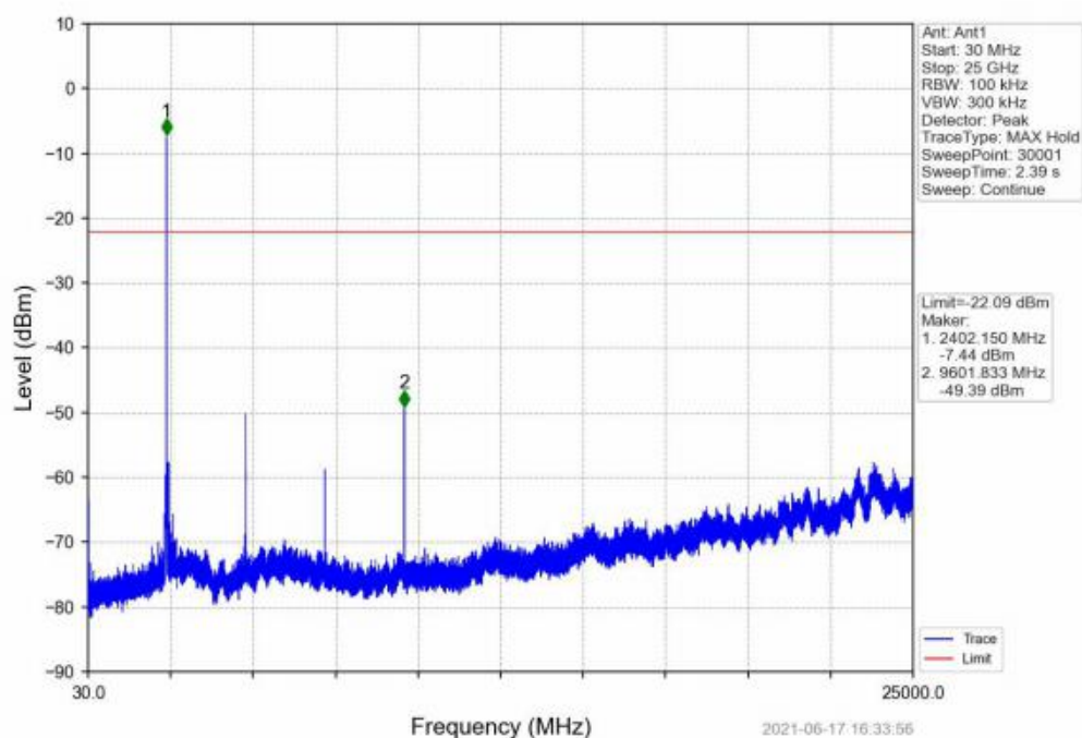
8DPSK_3DH5_LCH_2402MHz_Ant1_NTNV
