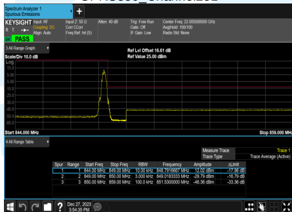
GPRS850_Channel251
