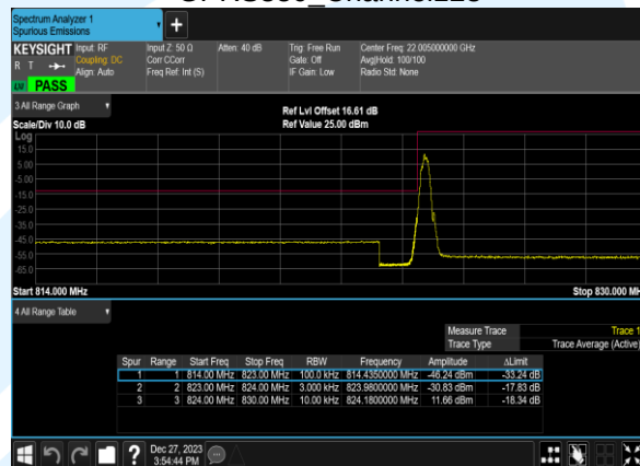
GPRS850_Channel128
