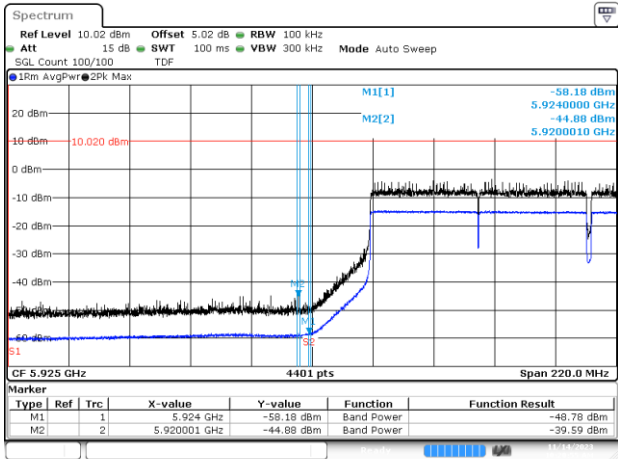
BE-NR-LOW, MIMO-B, 802.11ax160-HE0, Ch15
