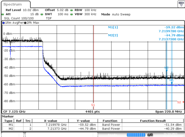
BE-NR-HIGH, MIMO-B, 802.11ax160-HE0, Ch207
