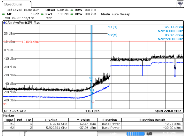
BE-NR-LOW, MIMO-B, 802.11be320-EHT0, Ch31
