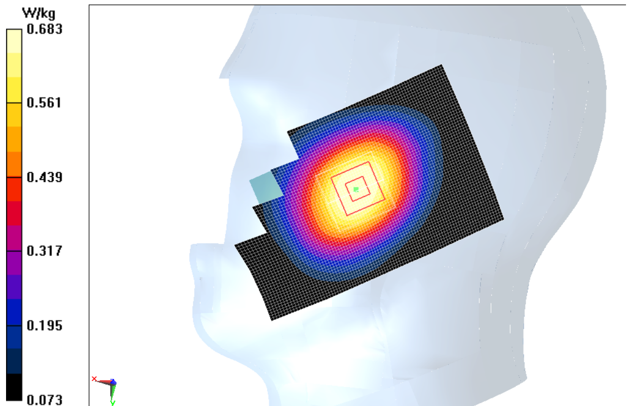
Fig.1 850MHz CH251
