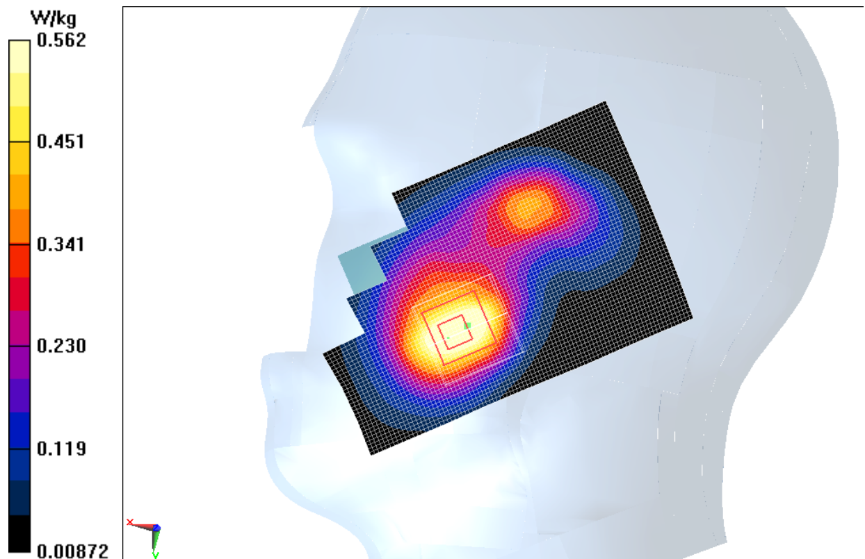
Fig.3 1900 MHz CH810
