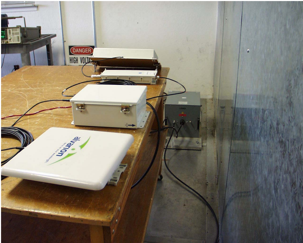
Line conducted test set-up
