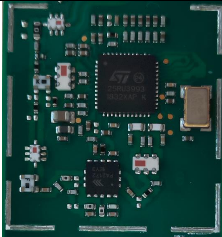
(14) EUT Photo (BT&WIFI Antenna)
