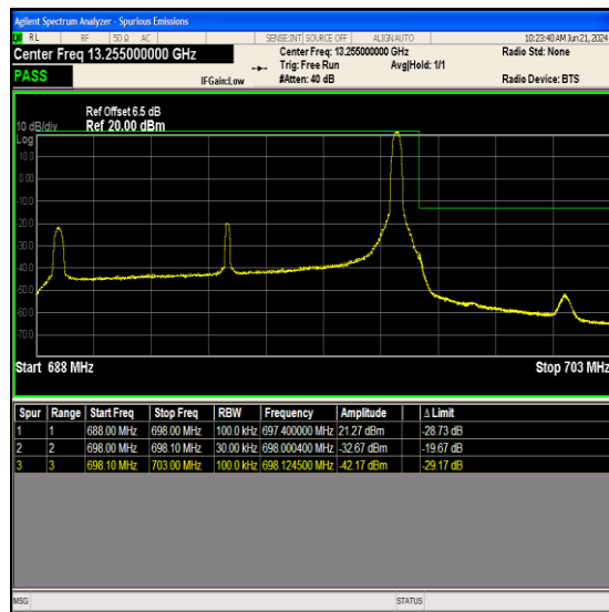
Band71_10MHz_QPSK_133422_1RB#49
