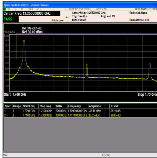
Band66_20MHz_16QAM_132072_1RB#0
