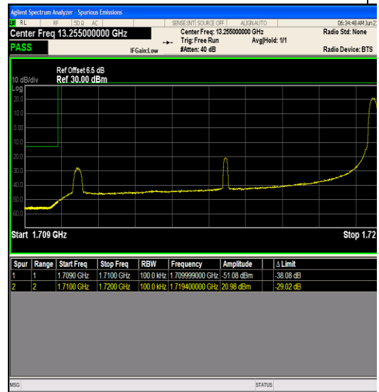
Band66_10MHz_QPSK_132022_1RB#49
