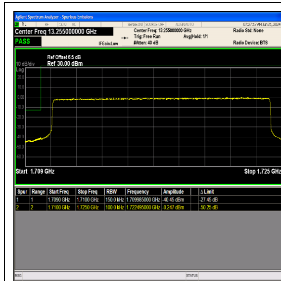
Band66_15MHz_16QAM_132047_75RB#0
