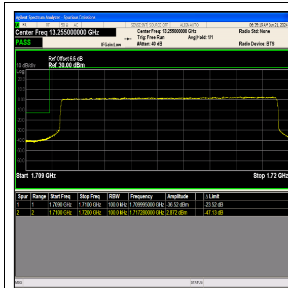
Band66_10MHz_QPSK_132022_50RB#0
