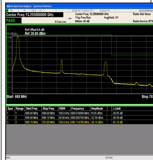
Band71_10MHz_64QAM_133422_1RB#0
