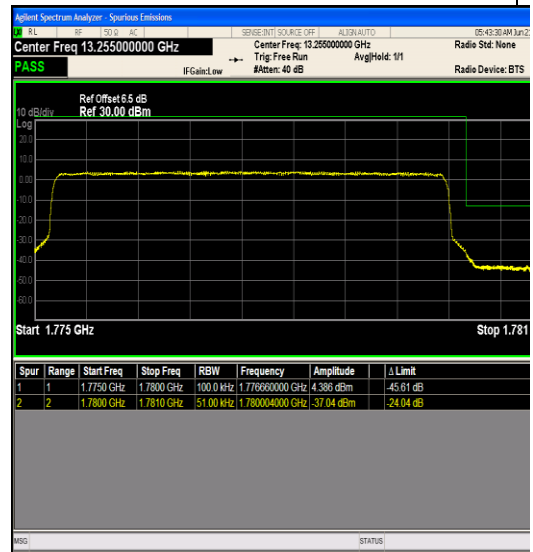
Band66_5MHz_16QAM_132647_25RB#0
