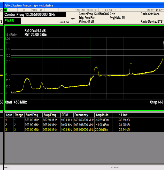
Band71_5MHz_16QAM_133147_1RB#24
