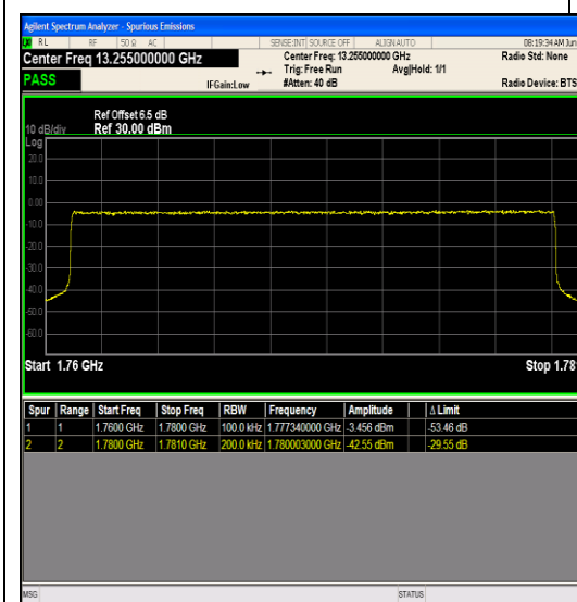
Band66_20MHz_64QAM_132572_1RB#0
