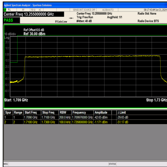
Band66_20MHz_16QAM_132072_100RB#0
