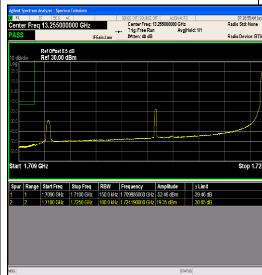
Band66_15MHz_64QAM_132047_1RB#74
