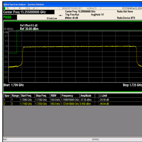
Band66_15MHz_QPSK_132047_75RB#0
