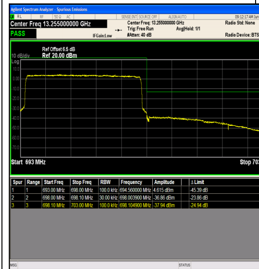
Band71_5MHz_16QAM_133447_25RB#0
