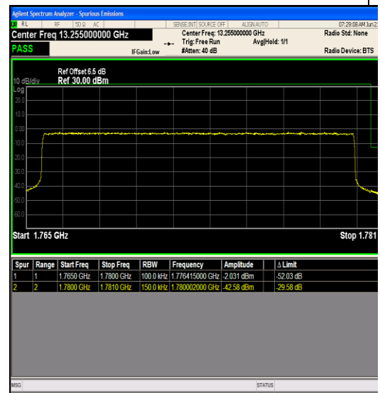
Band66_15MHz_64QAM_132597_75RB#0
