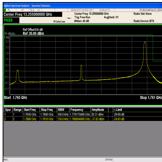
Band66_15MHz_16QAM_132597_1RB#74
