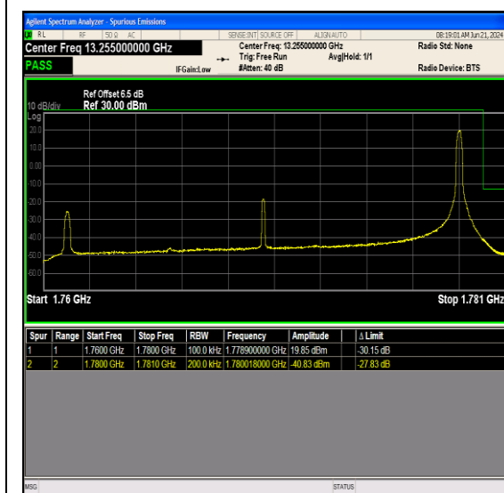
Band66_20MHz_64QAM_132072_100RB#0
