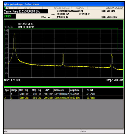
Band66_20MHz_16QAM_132572_1RB#0
