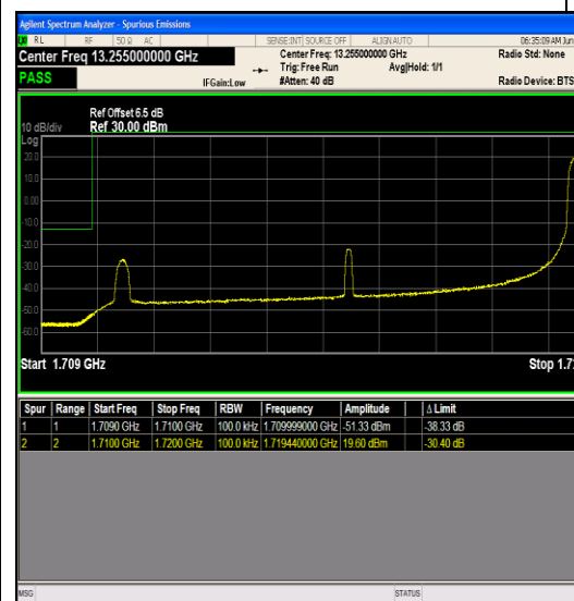
Band66_10MHz_QPSK_132622_50RB#0
