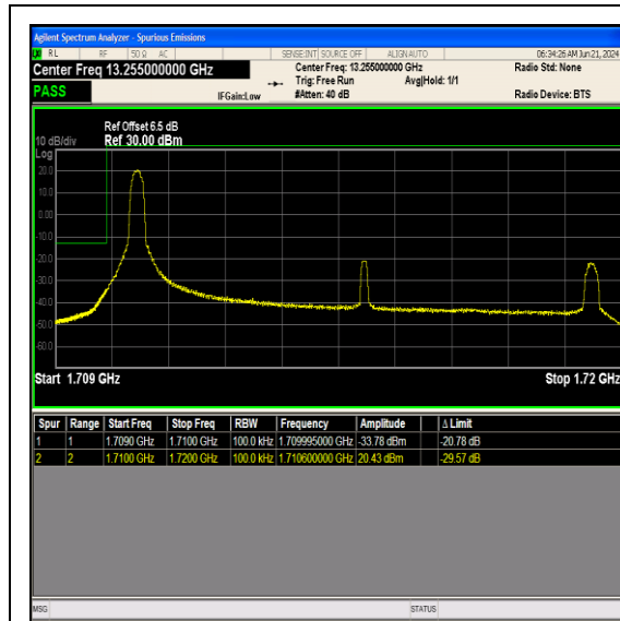
Band66_10MHz_16QAM_132022_1RB#0
