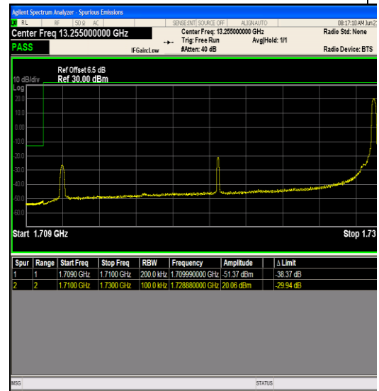
Band66_20MHz_16QAM_132072_1RB#99
