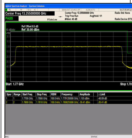
Band66_10MHz_16QAM_132622_1RB#0
