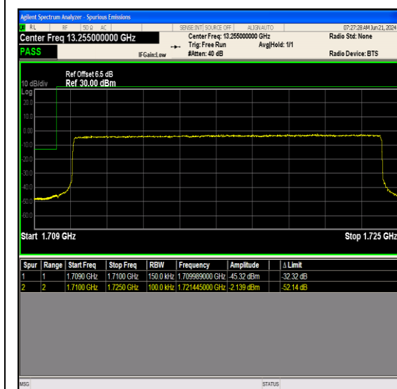
Band66_15MHz_64QAM_132047_1RB#0
