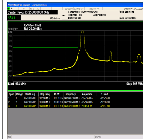
Band71_5MHz_64QAM_133147_1RB#0
