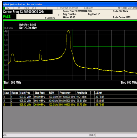
Band71_5MHz_64QAM_133447_1RB#24
