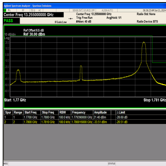
Band66_10MHz_QPSK_132622_1RB#49
