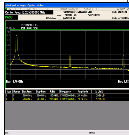
Band66_20MHz_64QAM_132572_1RB#0
