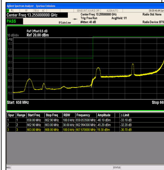
Band71_5MHz_64QAM_133147_1RB#24
