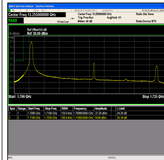
Band66_15MHz_64QAM_132047_1RB#0
