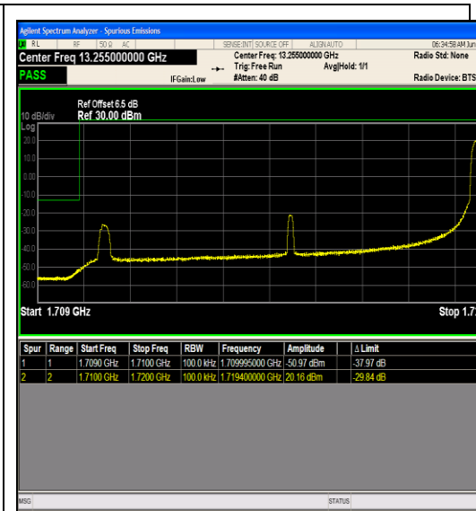
Band66_10MHz_16QAM_132022_1RB#49
