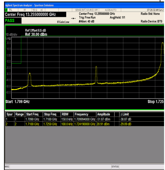
Band66_15MHz_QPSK_132047_1RB#74
