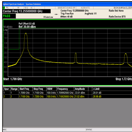
Band66_10MHz_QPSK_132022_1RB#0
