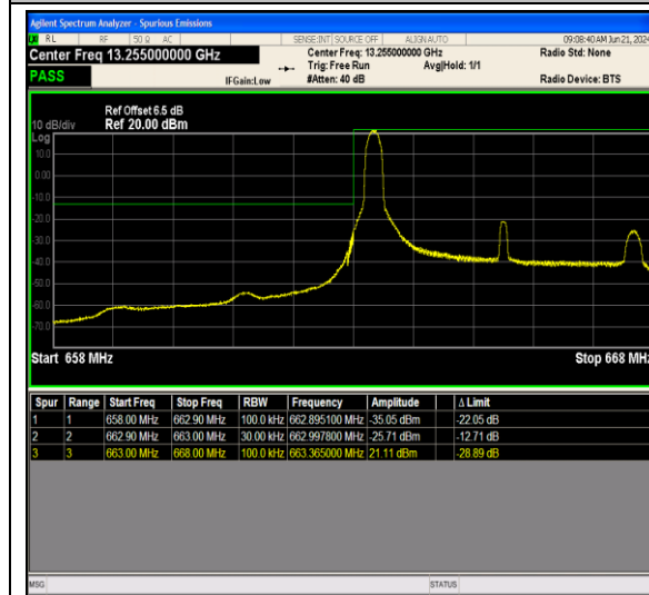
Band71_5MHz_QPSK_133147_1RB#0
