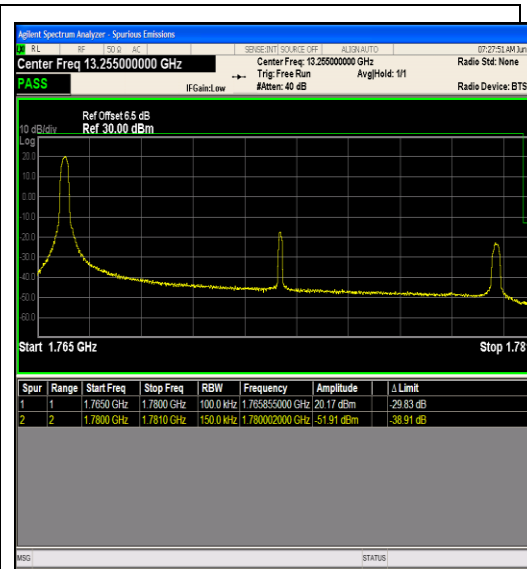
Band66_15MHz_16QAM_132597_1RB#0
