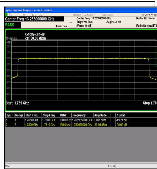
Band66_15MHz_QPSK_132597_75RB#0
