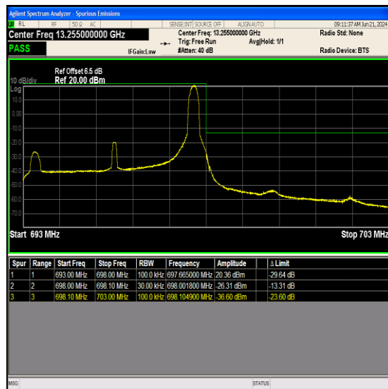
Band71_5MHz_16QAM_133447_1RB#24
