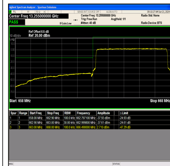
Band71_5MHz_64QAM_133147_1RB#0
