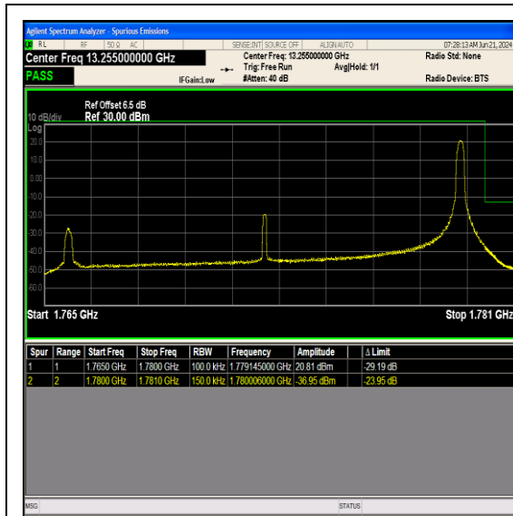
Band66_15MHz_QPSK_132597_1RB#74
