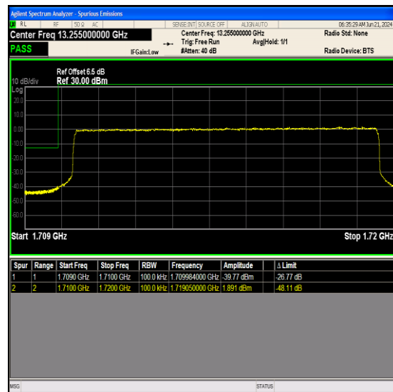
Band66_10MHz_16QAM_132022_50RB#0
