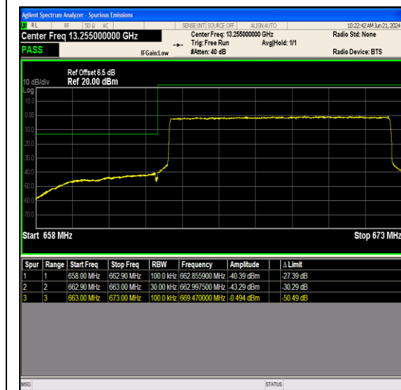
Band71_10MHz_64QAM_133172_50RB#0
