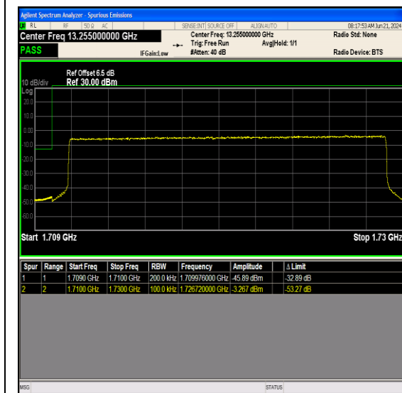
Band66_20MHz_64QAM_132072_100RB#0
