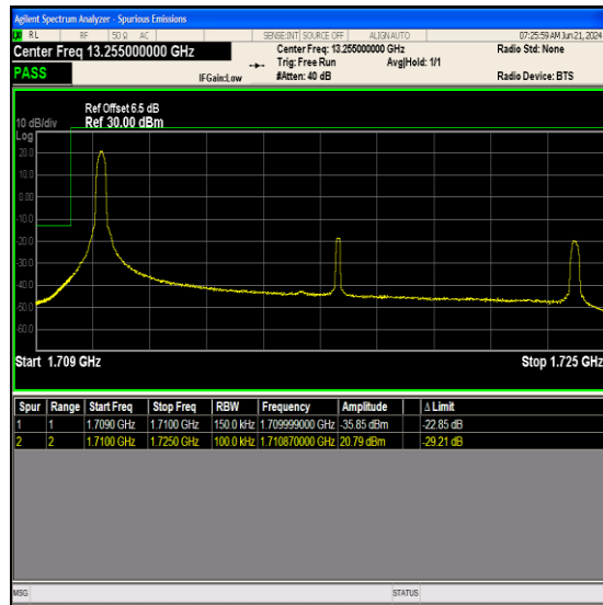
Band66_15MHz_QPSK_132047_1RB#0
