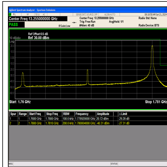
Band66_20MHz_16QAM_132572_1RB#99
