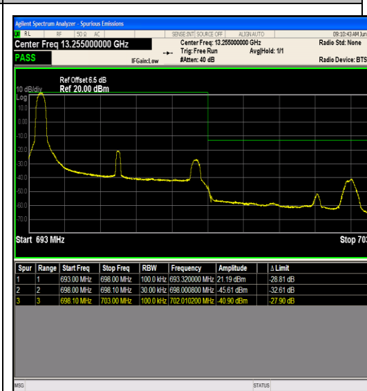
Band71_5MHz_QPSK_133447_1RB#0
