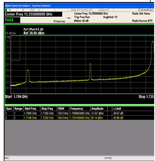
Band66_15MHz_16QAM_132047_1RB#74
