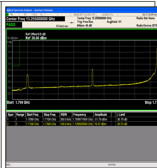
Band66_20MHz_64QAM_132072_1RB#99
