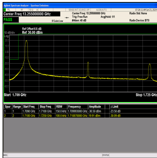
Band66_15MHz_16QAM_132047_1RB#0
