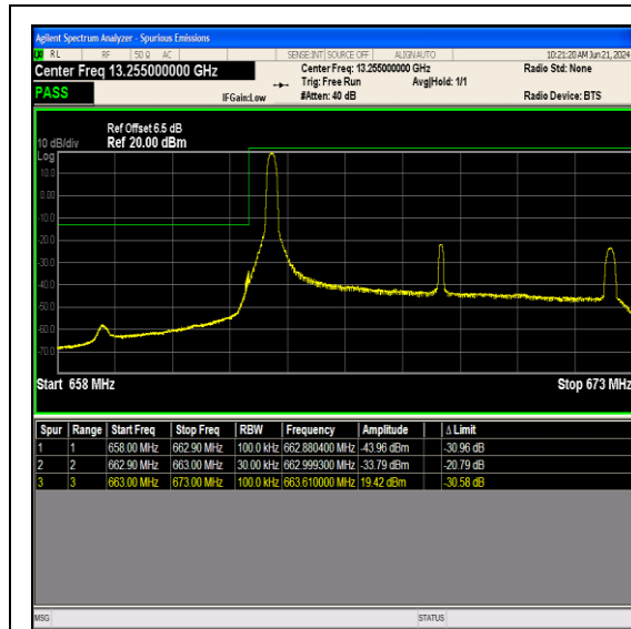
Band71_10MHz_64QAM_133172_1RB#0
