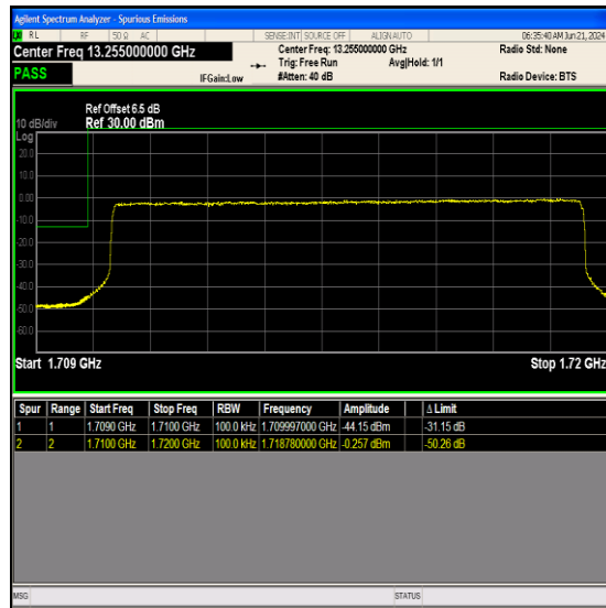
Band66_10MHz_64QAM_132022_50RB#0
