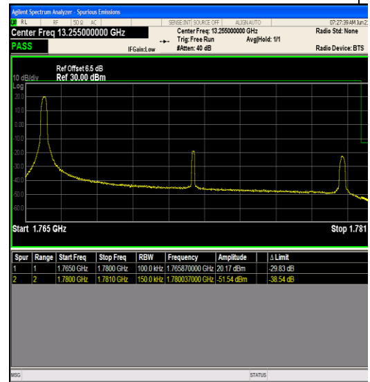
Band66_15MHz_QPSK_132597_1RB#0
