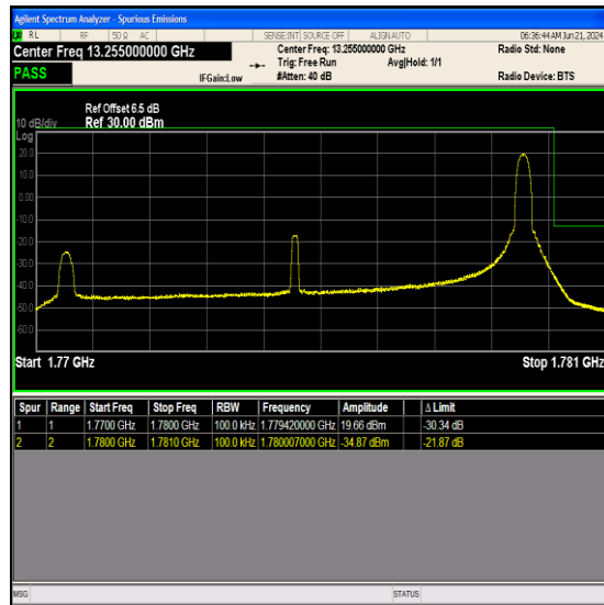
Band66_10MHz_64QAM_132622_1RB#49
