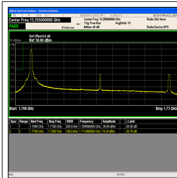
Band66_20MHz_64QAM_132072_1RB#0
