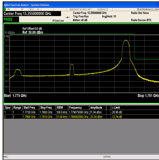
Band66_5MHz_16QAM_132647_1RB#24
