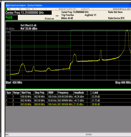
Band71_5MHz_QPSK_133147_1RB#24
