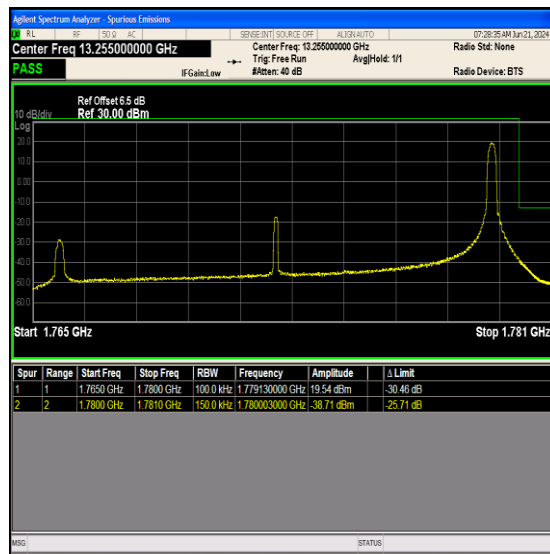
Band66_15MHz_64QAM_132597_1RB#74
