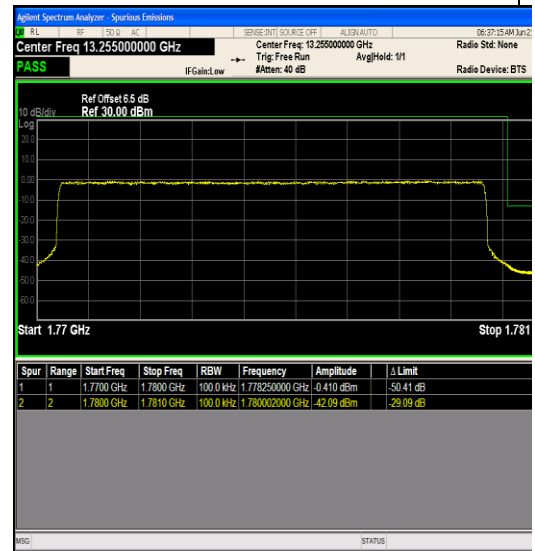
Band66_10MHz_64QAM_132622_50RB#0
