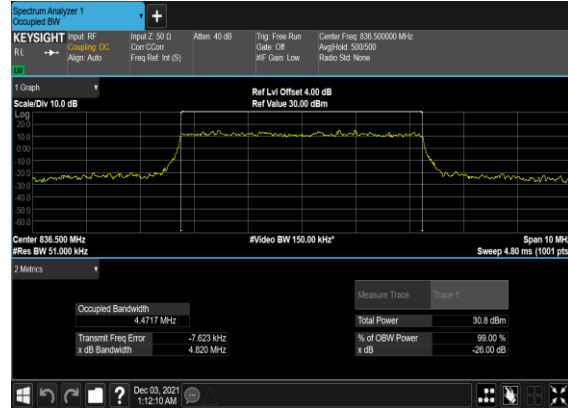
B7_N5(5M)_DFT-s- OFDM_QPSK_Outer_Full_Mid_CH
