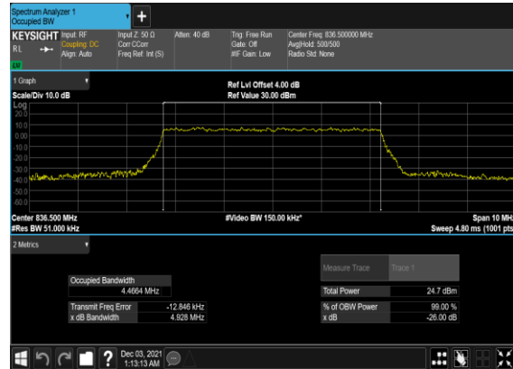
B7_N5(5M)_CP-OFDM_256 QAM_Outer_Full_Mid_CH
