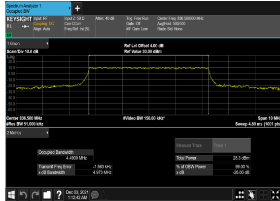
B7_N5(5M)_CP-OFDM_16 QAM_Outer_Full_Mid_CH
