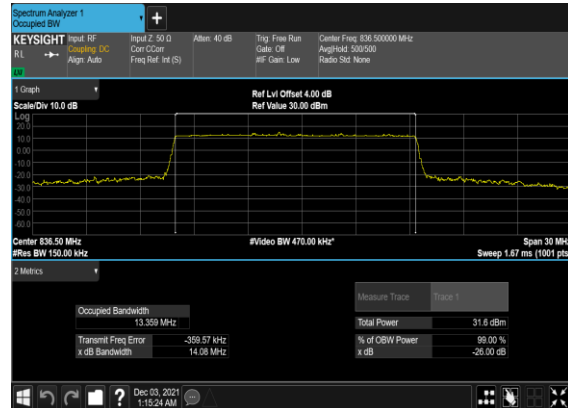
B7_N5(15M)_DFT-s- OFDM_QPSK_Outer_Full_Mid_CH
