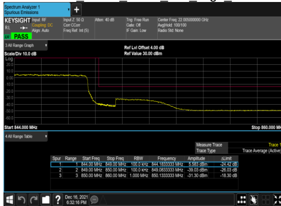
B7_N5(10M)_DFT-s- OFDM_BPSK_Outer_Full_High_CH
