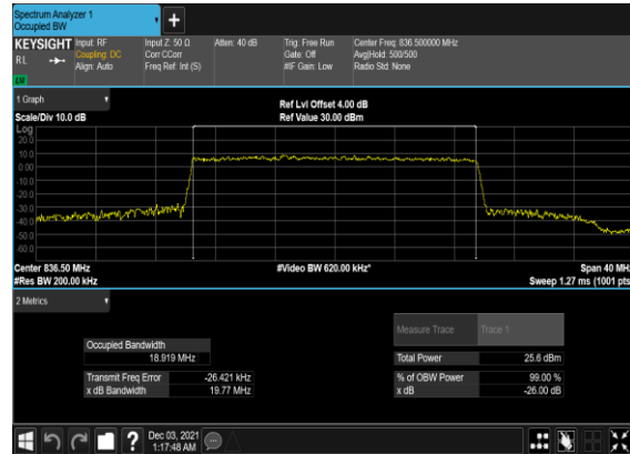
B7_N5(20M)_CP-OFDM_256 QAM_Outer_Full_Mid_CH
