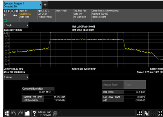
B7_N5(20M)_CP-OFDM_16 QAM_Outer_Full_Mid_CH
