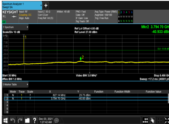
B7_N5(20M)_DFT-s- OFDM_BPSK_Edge_1RB_Left_Mid_CH
