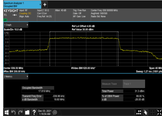
B7_N5(20M)_DFT-s- OFDM_QPSK_Outer_Full_Mid_CH
