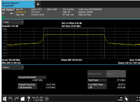
B7_N5(5M)_CP- OFDM_QPSK_Outer_Full_Mid_CH
