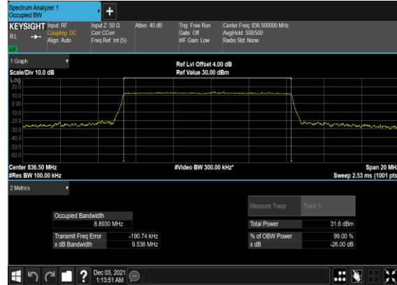
B7_N5(10M)_DFT-s- OFDM_QPSK_Outer_Full_Mid_CH
