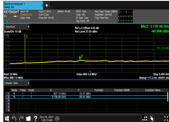
B7_N5(20M)_DFT-s- OFDM_QPSK_Edge_1RB_Left_Mid_CH
