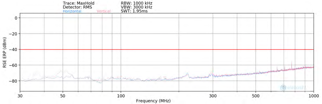
Plot 8-267. Radiated spurious emission Plot_30 MHz to 1000 MHz (n48_1C_10M_QPSK - Mid Channel) (Sector 1)
