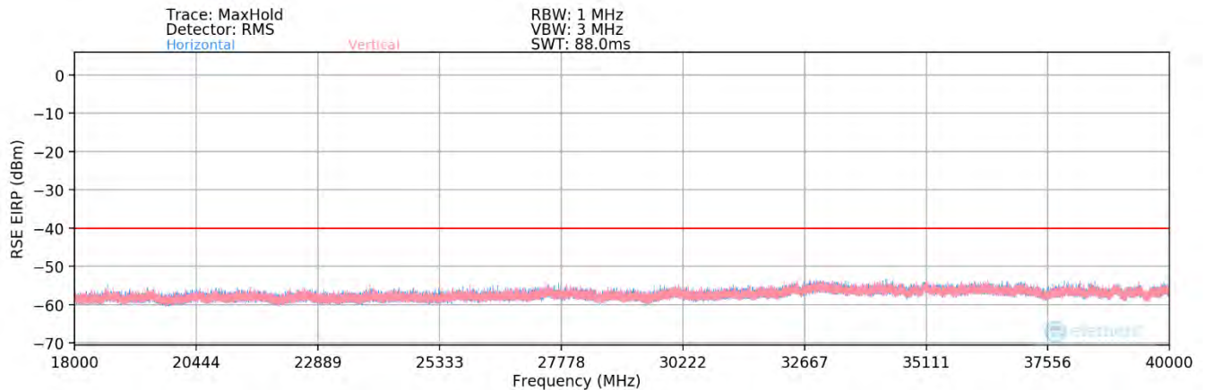
Plot 8-272. Radiated spurious emission Plot_18 GHz to 40 GHz (n48_1C_10M_QPSK - High Channel_4T) (Sector 1)
