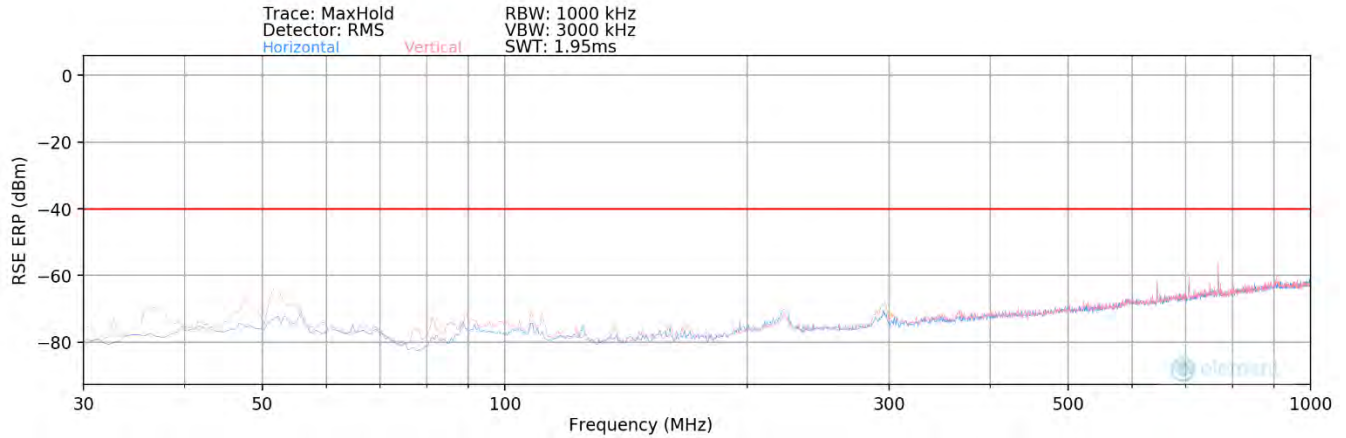
Plot 8-291. Radiated spurious emission Plot_30 MHz to 1000 MHz (n48_2C_40M+40M_QPSK - Mid Channel_8T)
