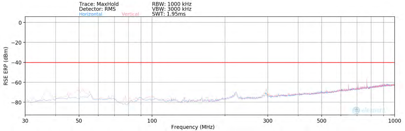
Plot 8-282. Radiated spurious emission Plot_30 MHz to 1000 MHz (n48_1C_10M_QPSK - Low Channel_8T)
