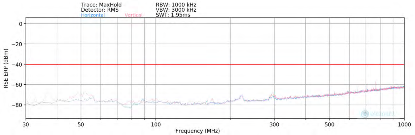
Plot 8-276. Radiated spurious emission Plot_30 MHz to 1000 MHz (n48_2C_40M+40M_Non-Contiguous_QPSK - Mid Channel_4T) (Sector 1)
