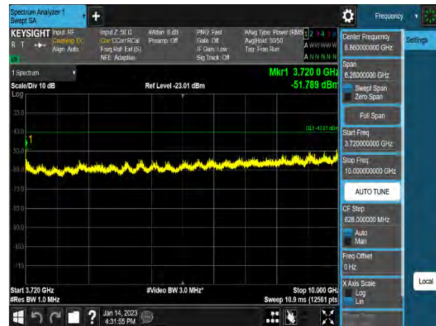
Plot 8-257. Conducted Spurious Emission Plot 3.72 GHz to 10 GHz (n48_2NC_40M+40M_QPSK - Mid Channel_2T, Port 3)
