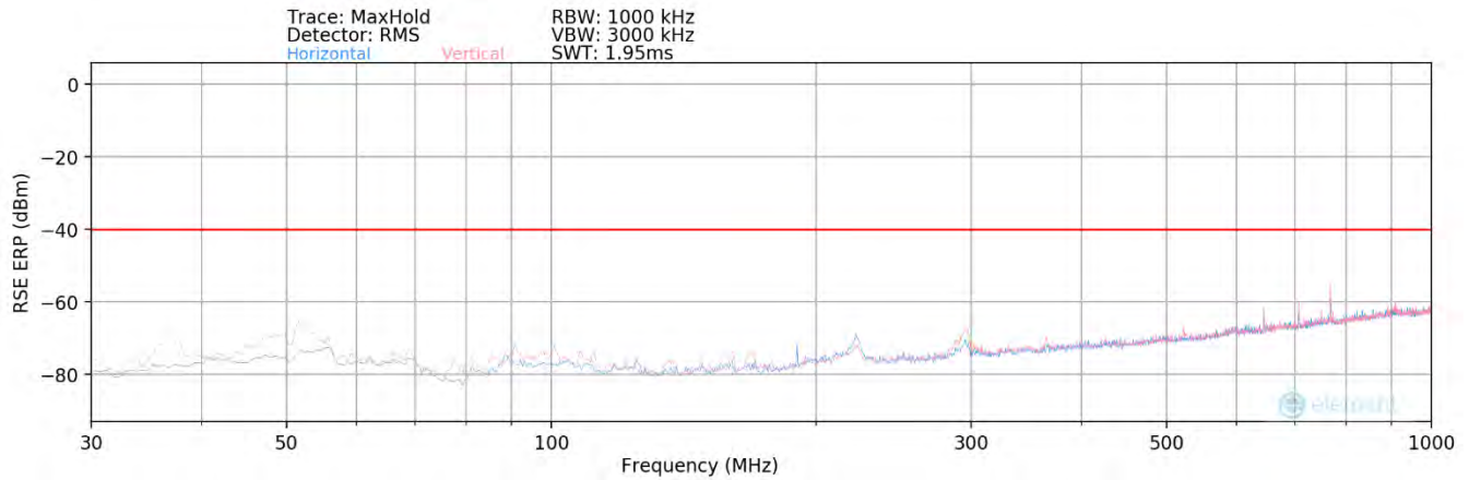
Plot 8-288. Radiated spurious emission Plot_30 MHz to 1000 MHz (n48_1C_10M_QPSK - High Channel_8T)
