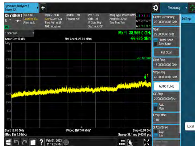
Plot 8-259. Conducted Spurious Emission Plot 18 GHz to 40 GHz (n48_2NC_40M+40M_QPSK - Mid Channel_2T, Port 3)
