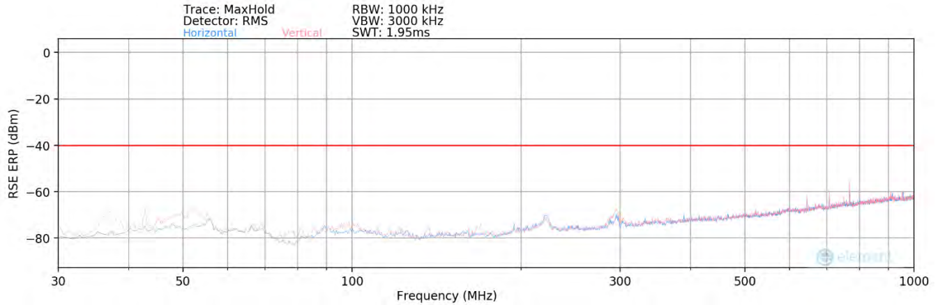
Plot 8-279. Radiated spurious emission Plot_30 MHz to 1000 MHz (n48_1C_10M_QPSK - Mid Channel_4T) (Sector 2)
