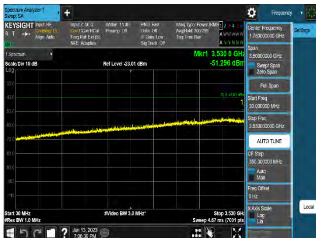
Plot 8-252. Conducted Spurious Emission Plot 30 MHz to 3.53 GHz (n48_2C_40M+40M_256QAM - Low Channel_2T, Port 4)
