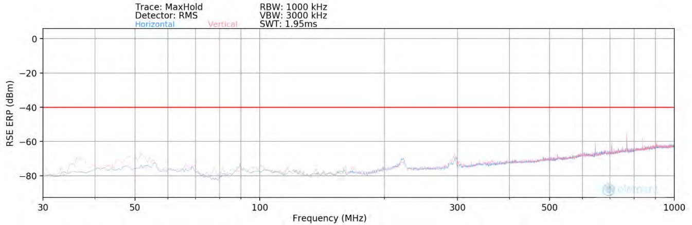
Plot 8-273. Radiated spurious emission Plot_30 MHz to 1000 MHz (n48_2C_40M+40M_QPSK - Mid Channel_4T) (Sector 1)
