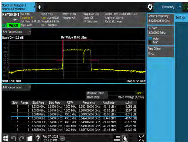
Plot 8-246. Channel Edge Emission Plot (n48_2C_30M+10M_QPSK – Mid Channel_8T, Port 1)
