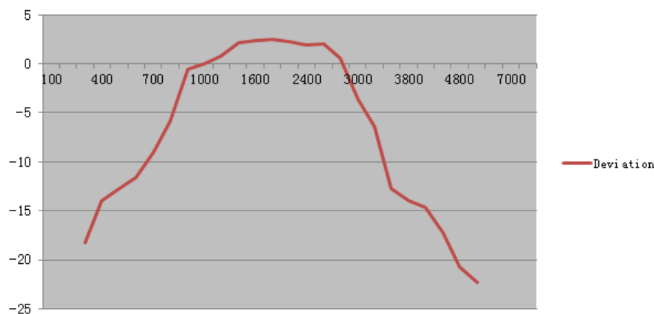
Audio Frequency Response@50%MI
