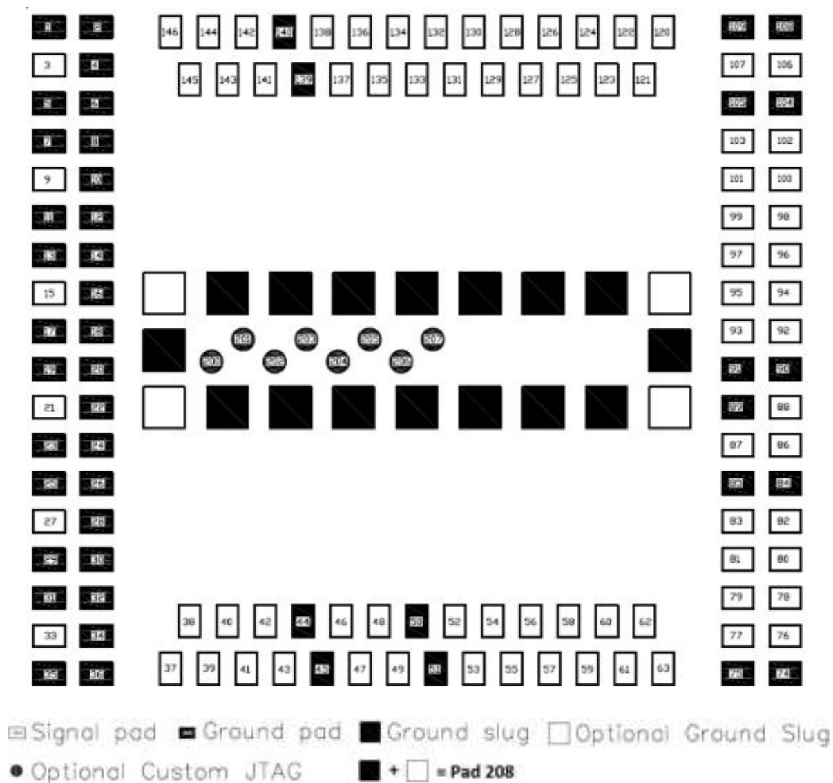
Figure 1. LGA pad diagram (top view)
