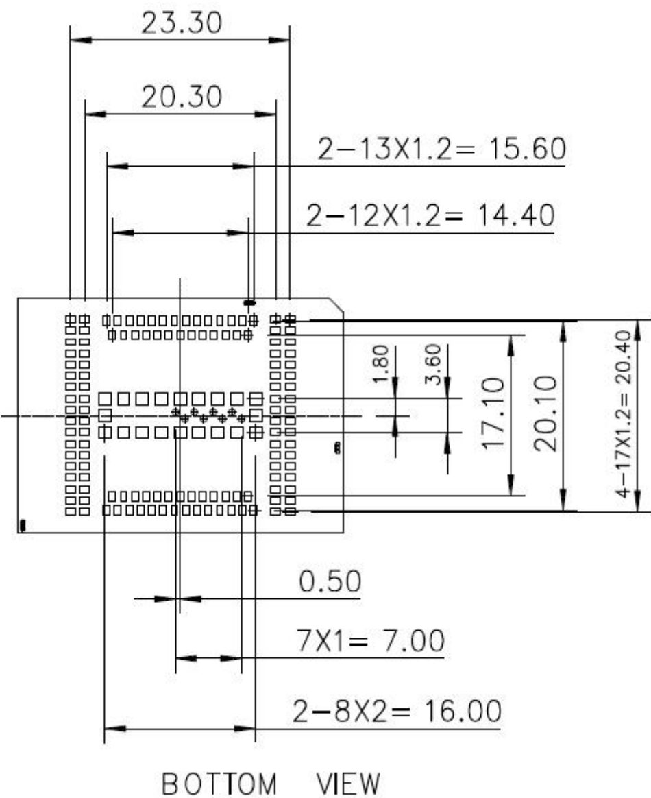
Figure 3. Pad dimension(Bottom view)
