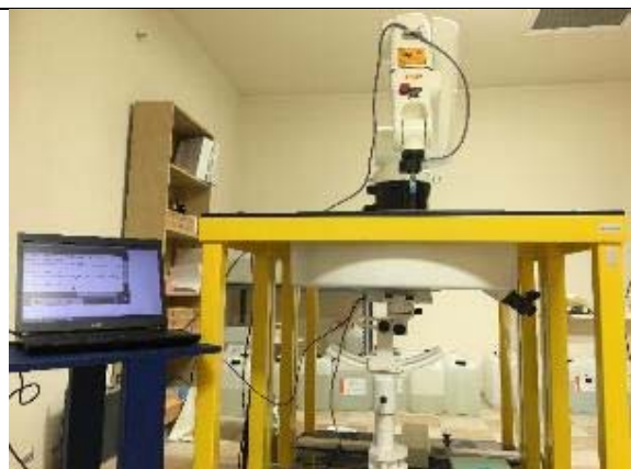
SAR Test System
