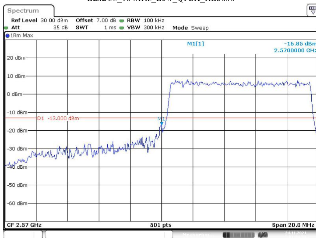
Band 38 10 MHz Low QPSK RB50#0
