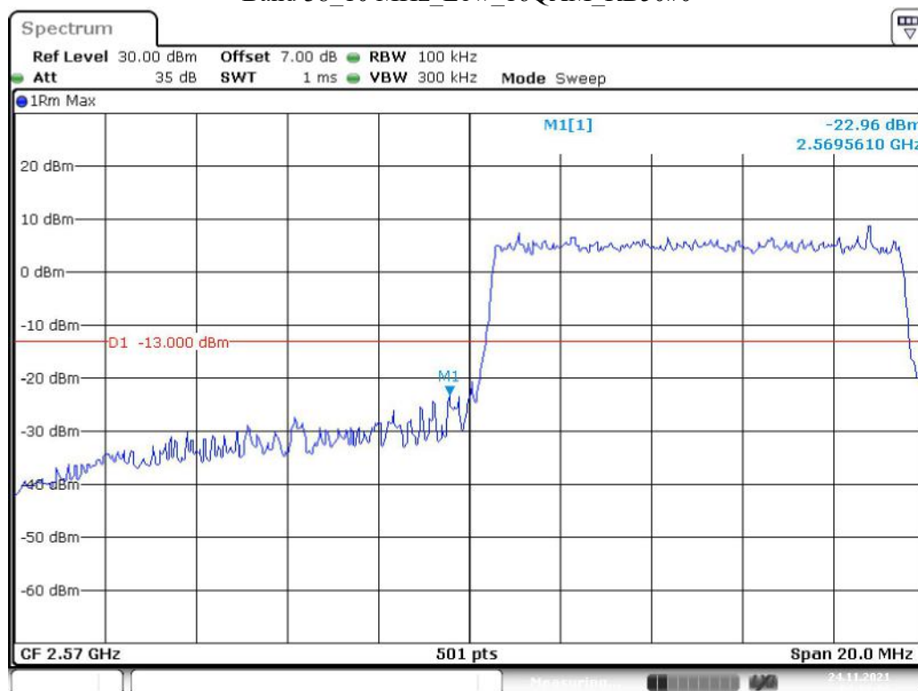
Band 38 10 MHz Low 16QAM RB50#0
