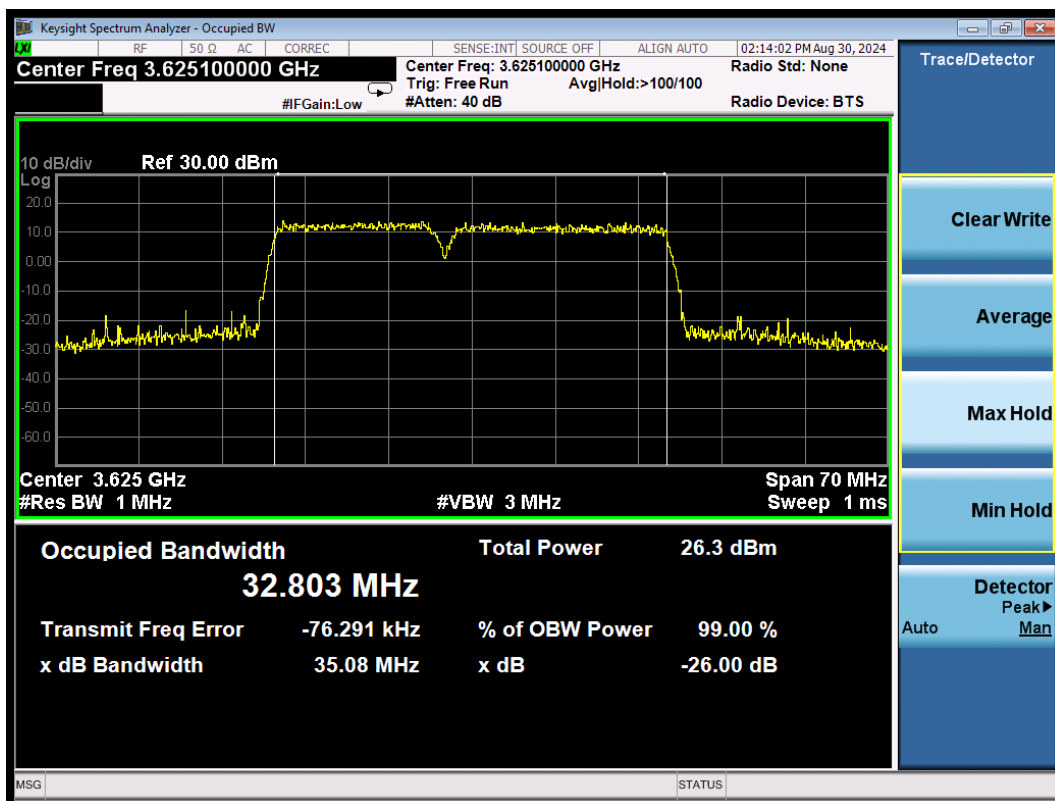
CA_48C 64QAM\15MHz+20MHz Middle
