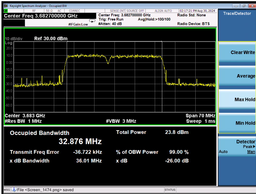
CA_48C 256QAM\15MHz+20MHz High
