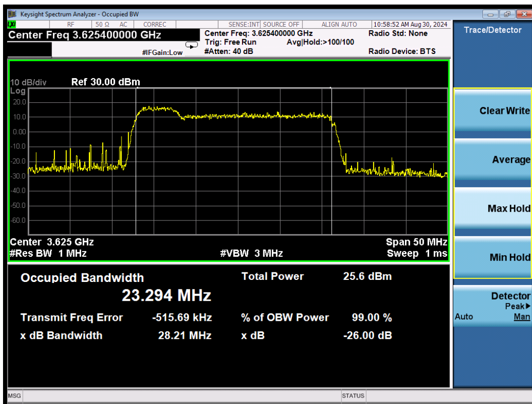
CA_48C 16QAM\5MHz+20MHz Middle
