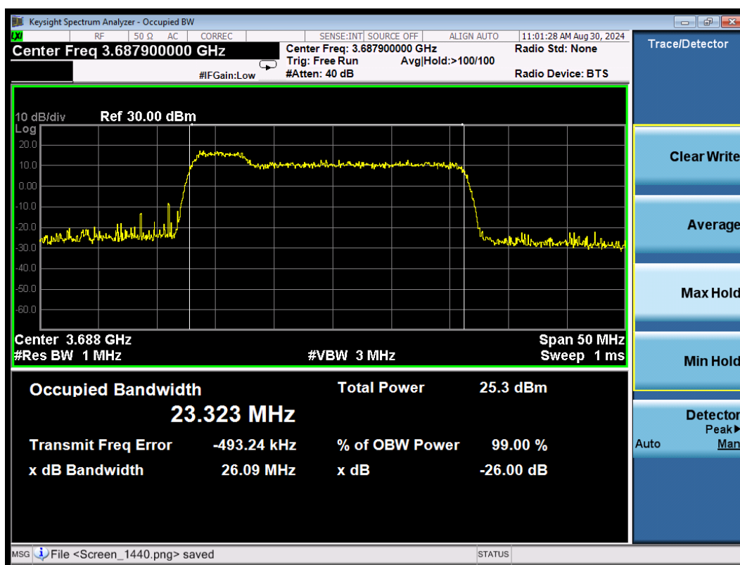
CA_48C 64QAM\5MHz+20MHz High
