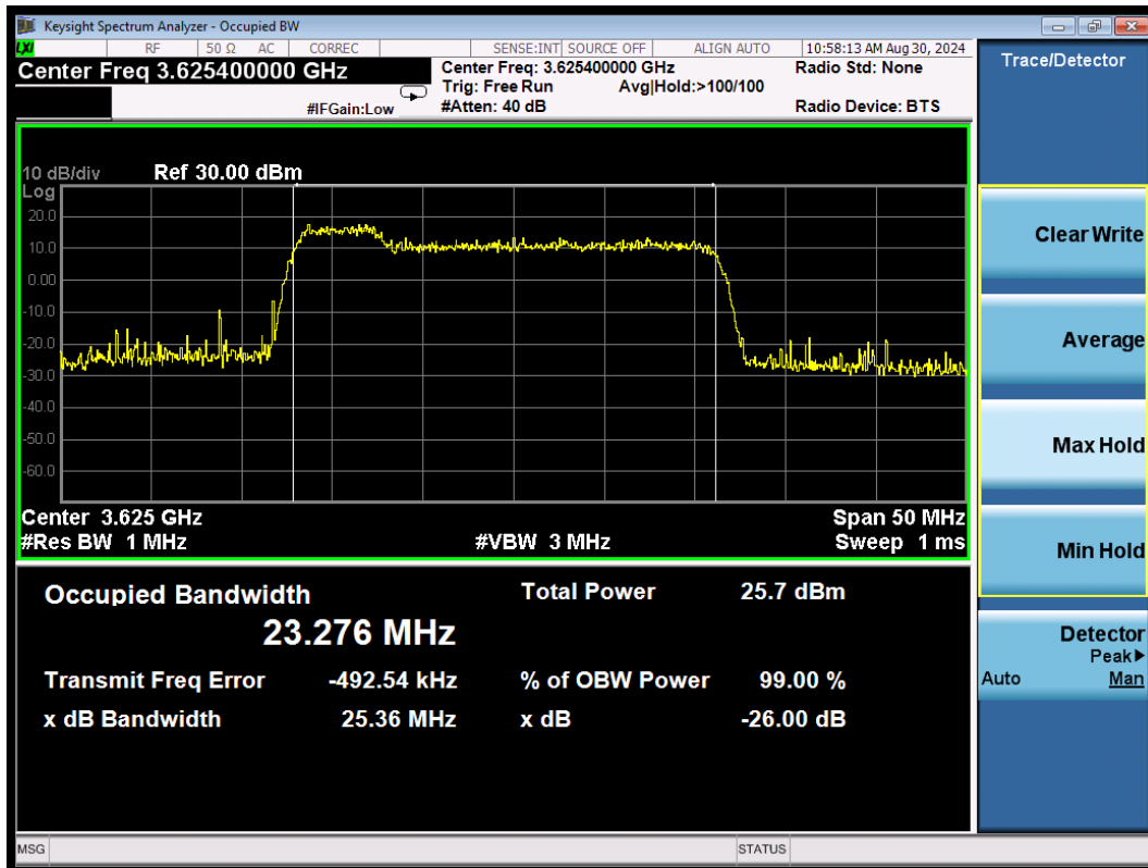
CA_48C 64QAM\5MHz+20MHz Middle
