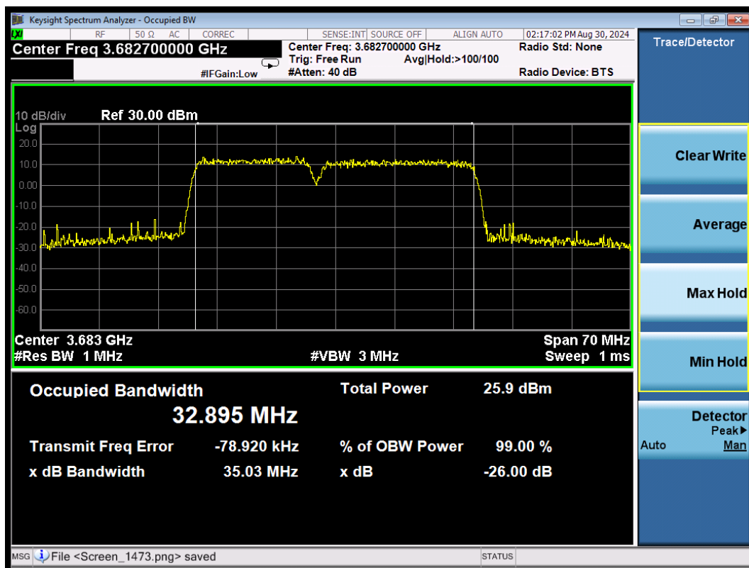
CA_48C 64QAM\15MHz+20MHz High
