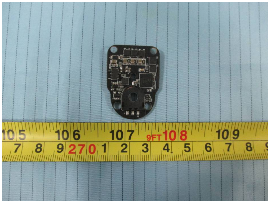
EUT – Pan-Tilt Main Board 4 Top View
