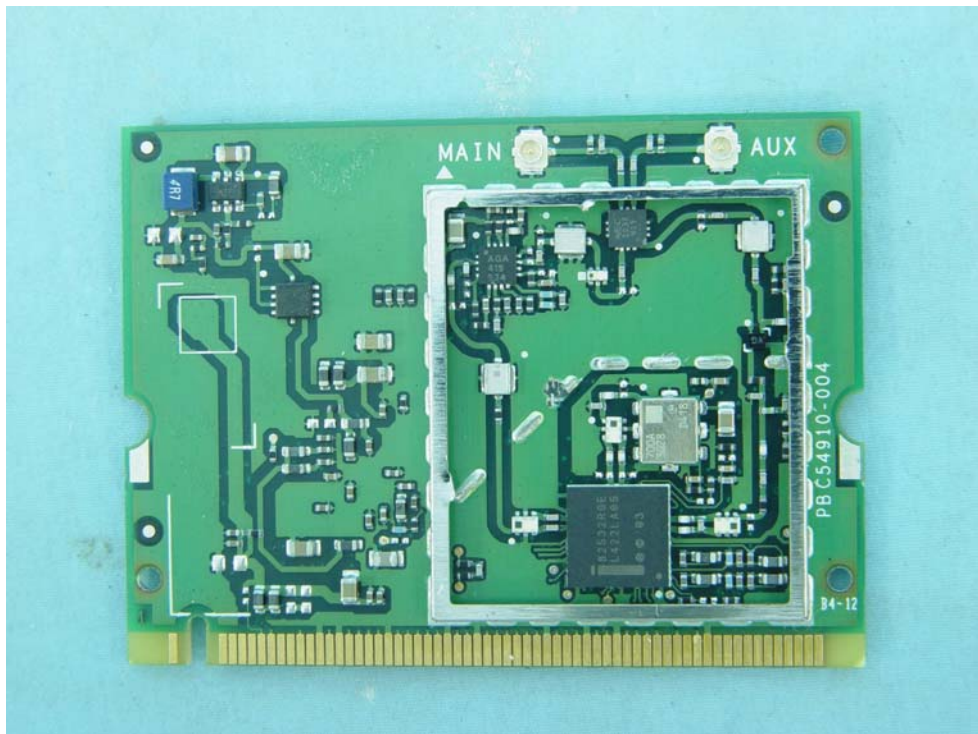
WLAN Module: Side A (without cover and shield)
