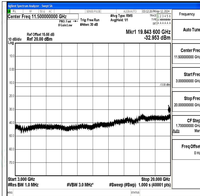
Band4_15MHz_QPSK_20325_1RB#0_3000~20000_300 0~20000
