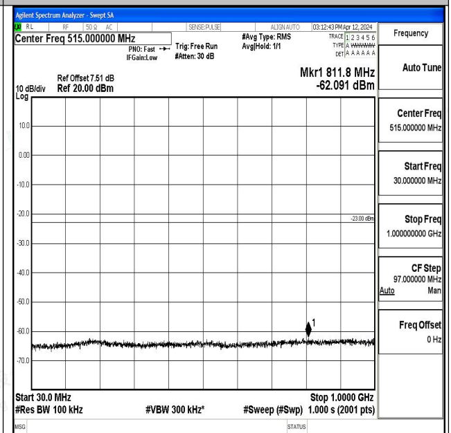
Band4_15MHz_16QAM_20325_1RB#0_30~1000_30~10 00
