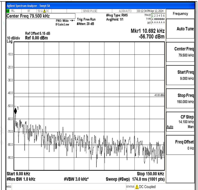
Band4_15MHz_16QAM_20325_1RB#0_0.009~0.15_0.0 09~0.15
