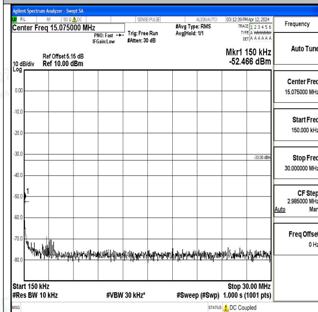
Band4_15MHz_16QAM_20325_1RB#0_0.15~30_0.15~3 0
