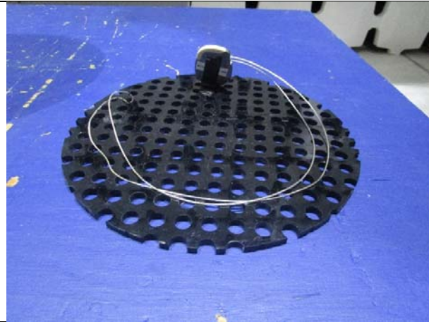
EUT Setup – Front View
