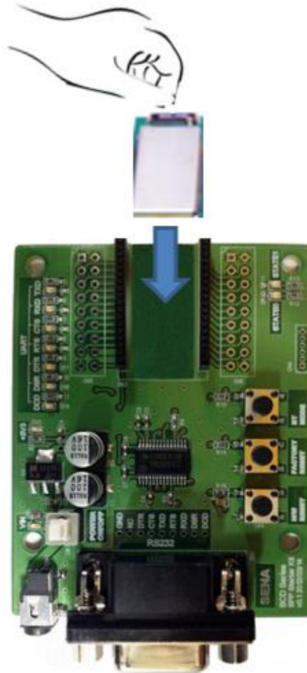
Figure 2-2 Connecting IW05 to Development Board
