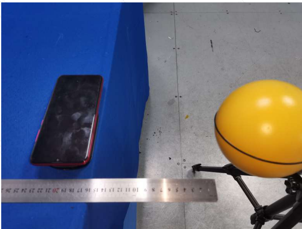
Test Position E(16cm) - Exposure photo from side edge surface-Right(TM1)
