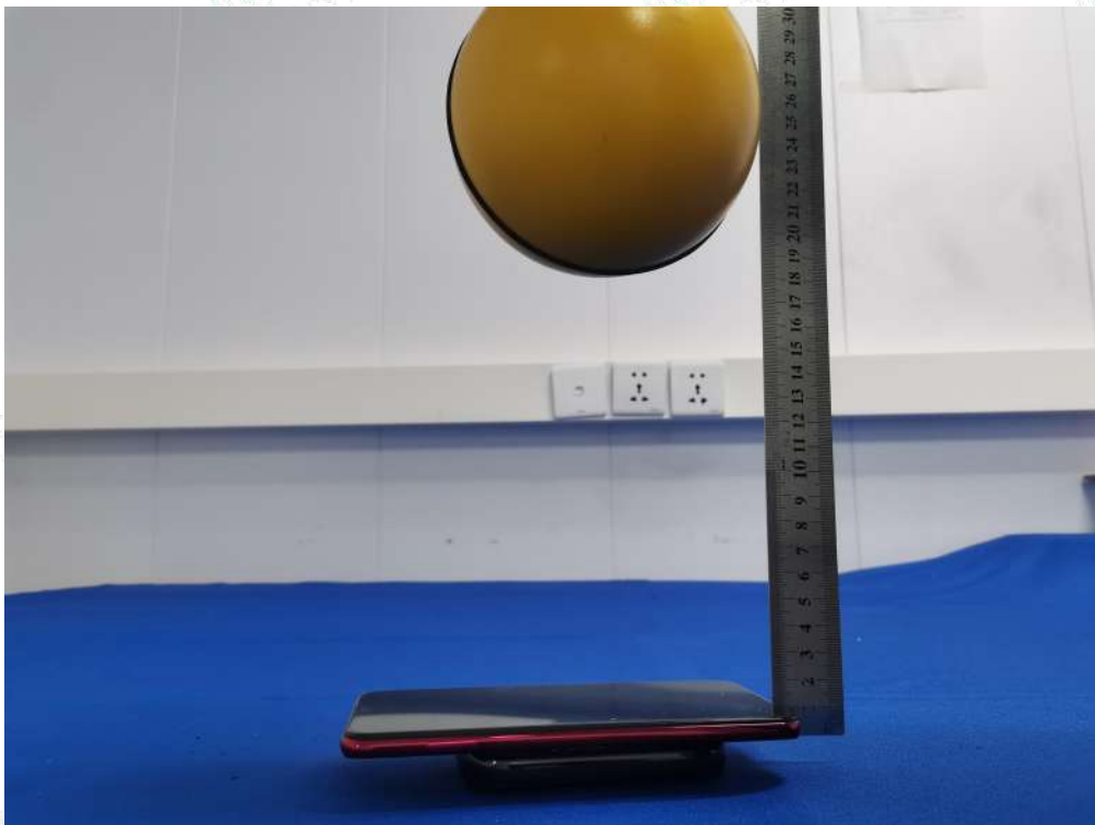
Test Position A (18cm) - Exposure photo from top surface (TM1)
