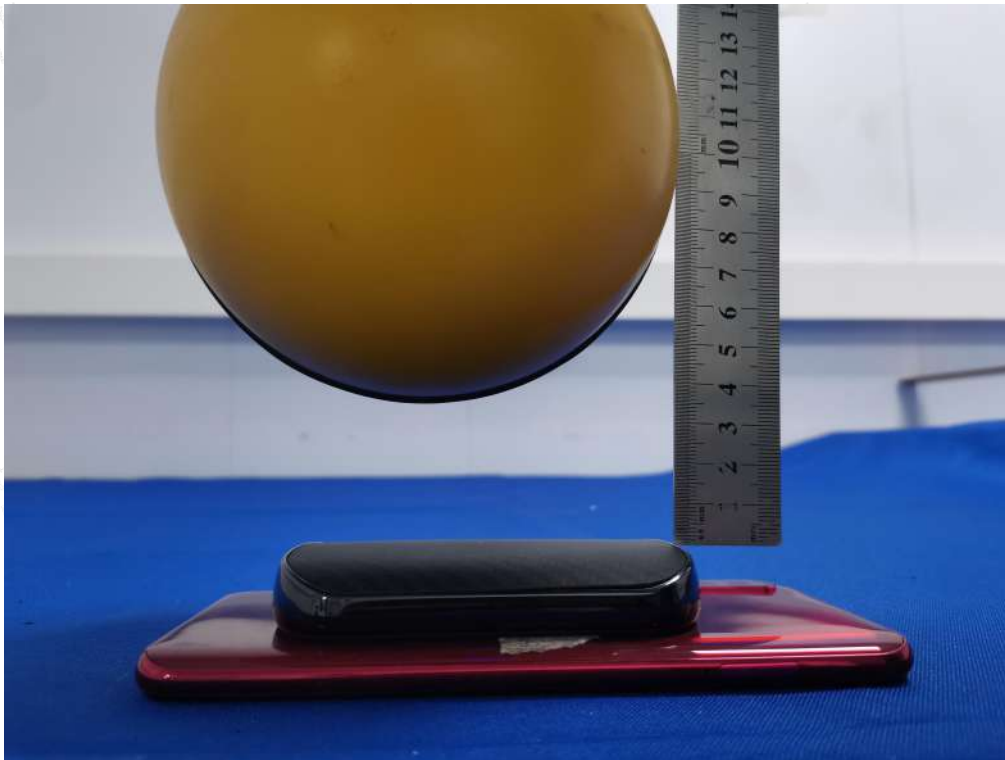
Test Position F(4cm) - Exposure photo from bottom surface(TM1)
