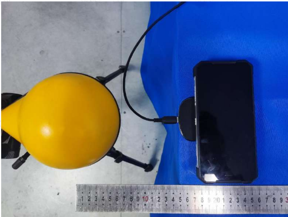
Test Position D(15cm) - Exposure photo from side edge surface-Front(TM1)
