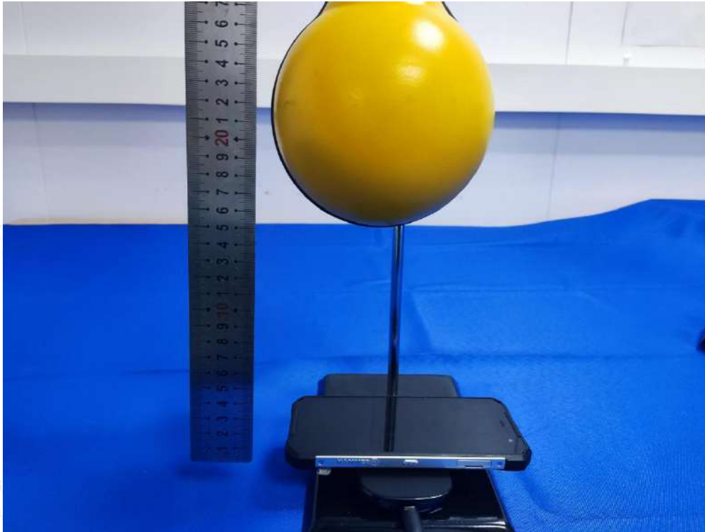
Test Position A (20cm) - Exposure photo from top surface (TM1)
