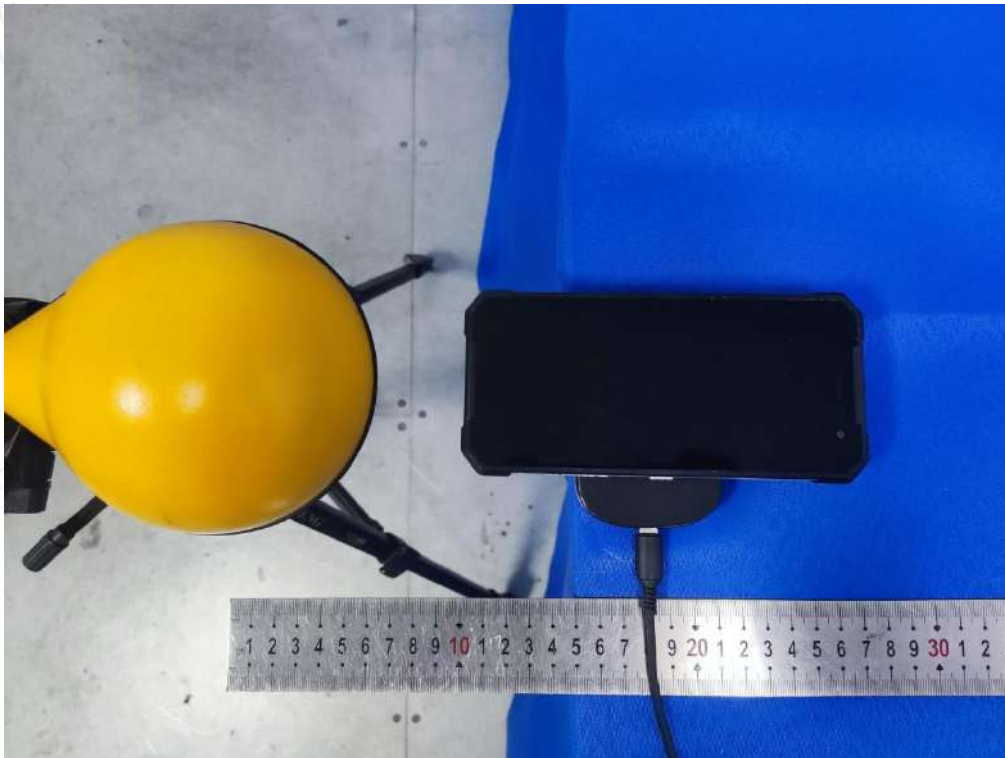
Test Position E(15cm) - Exposure photo from side edge surface-Right(TM1)
