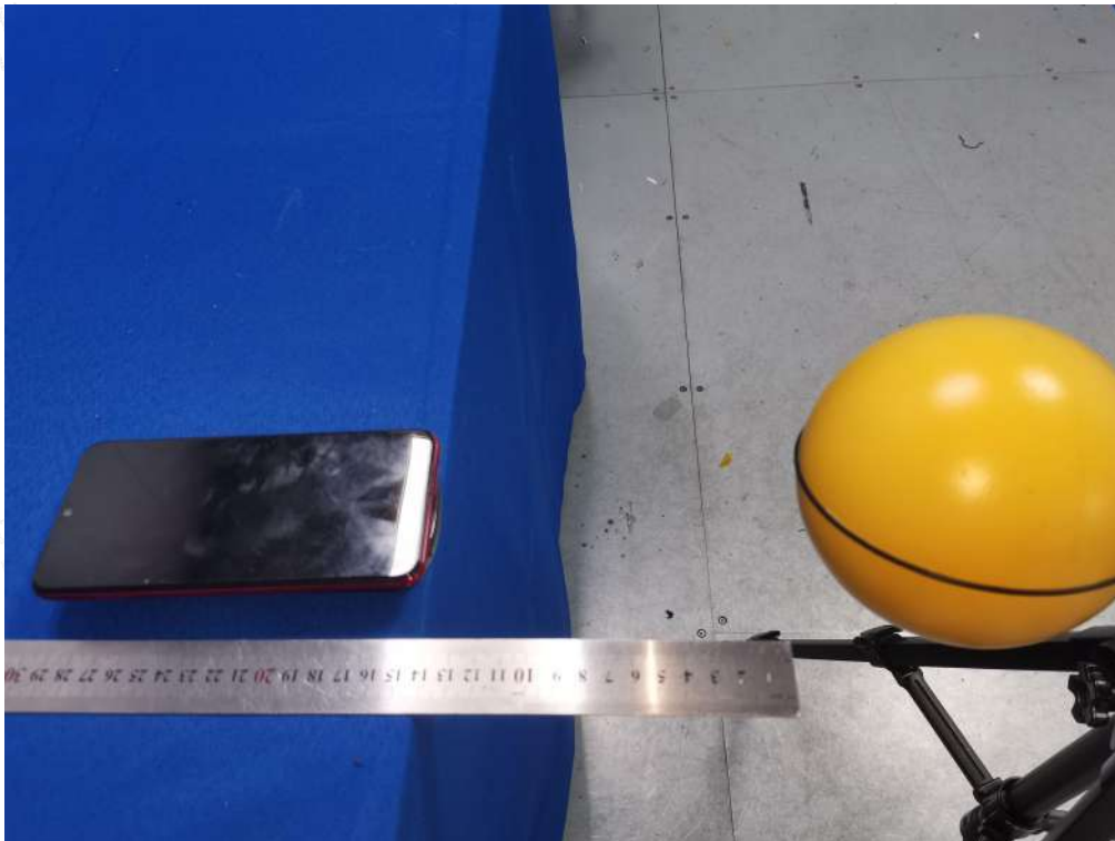
Test Position D(14cm) - Exposure photo from side edge surface-Front(TM1)
