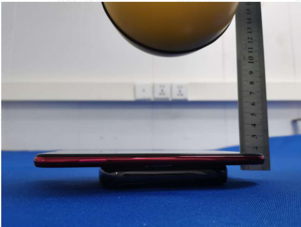
Test Position A (10cm) - Exposure photo from top surface (TM1)
