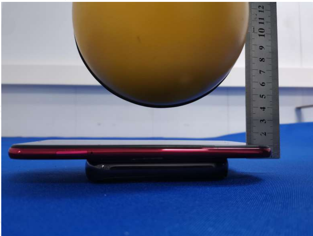
Test Position A (4cm) - Exposure photo from top surface (TM1)
