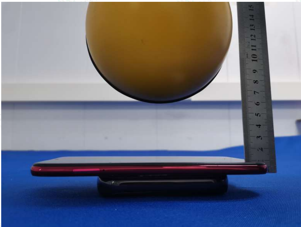
Test Position A (6cm) - Exposure photo from top surface (TM1)
