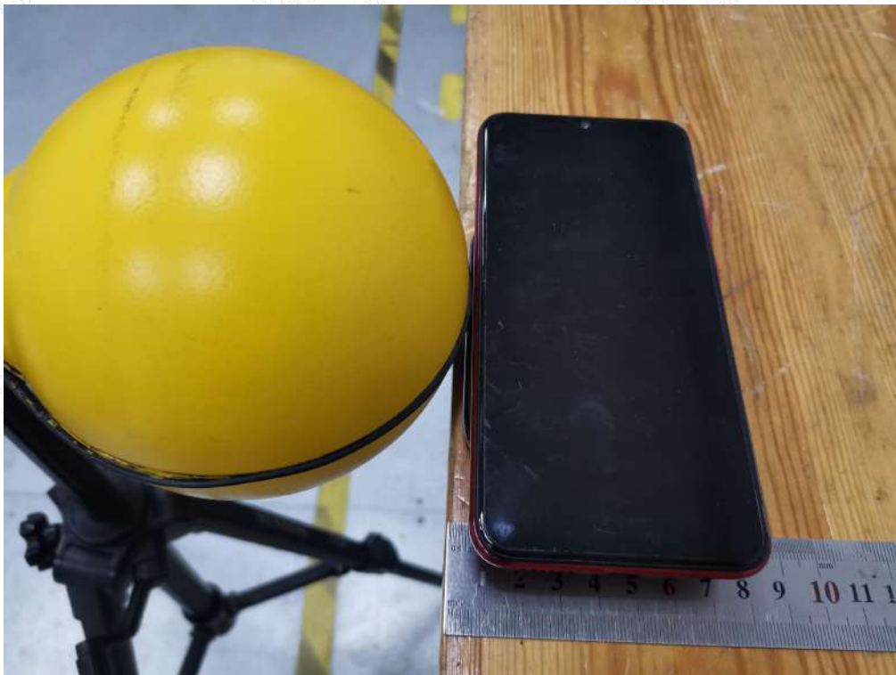
Test Position C(0cm) - Exposure photo from side edge surface-Left(TM1)
