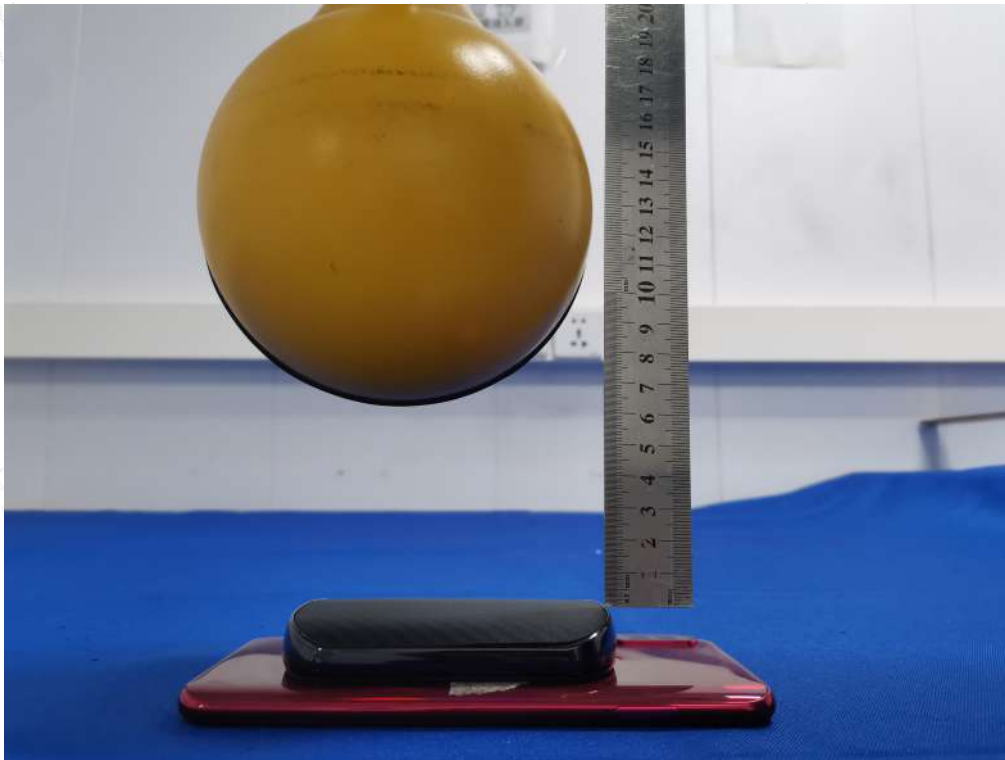
Test Position F(6cm) - Exposure photo from bottom surface(TM1)
