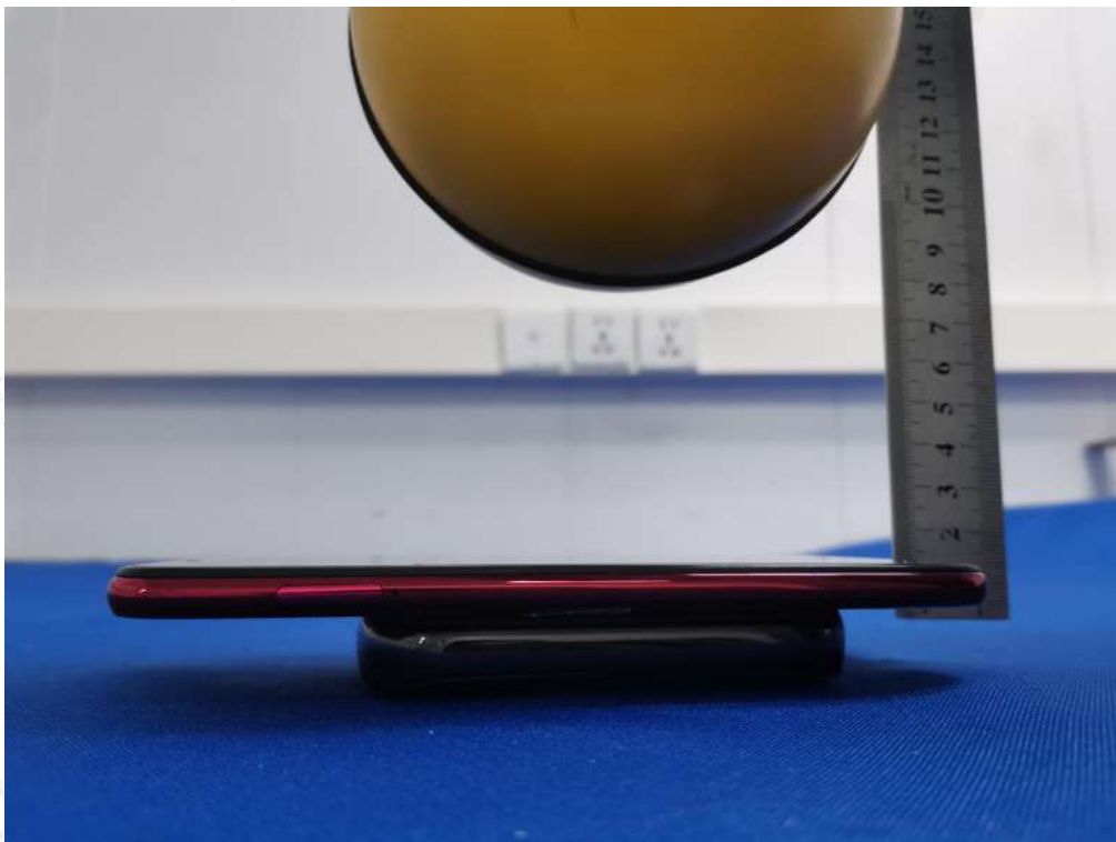
Test Position A(8cm) - Exposure photo from top surface (TM1)
