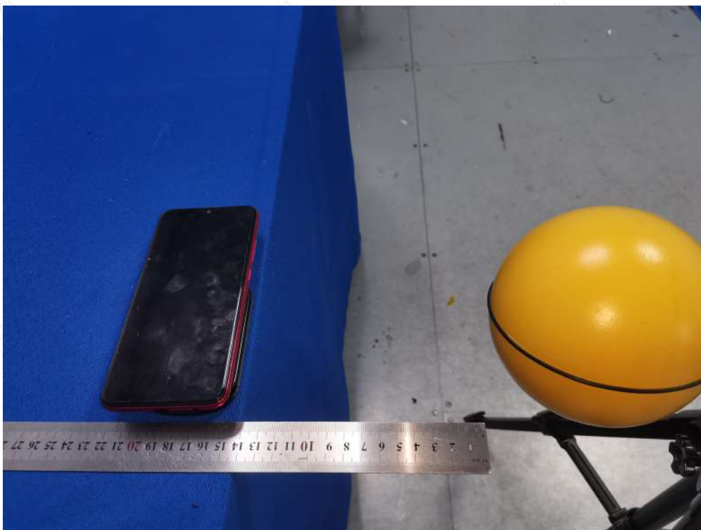
Test Position E(14cm) - Exposure photo from side edge surface-Right(TM1)
