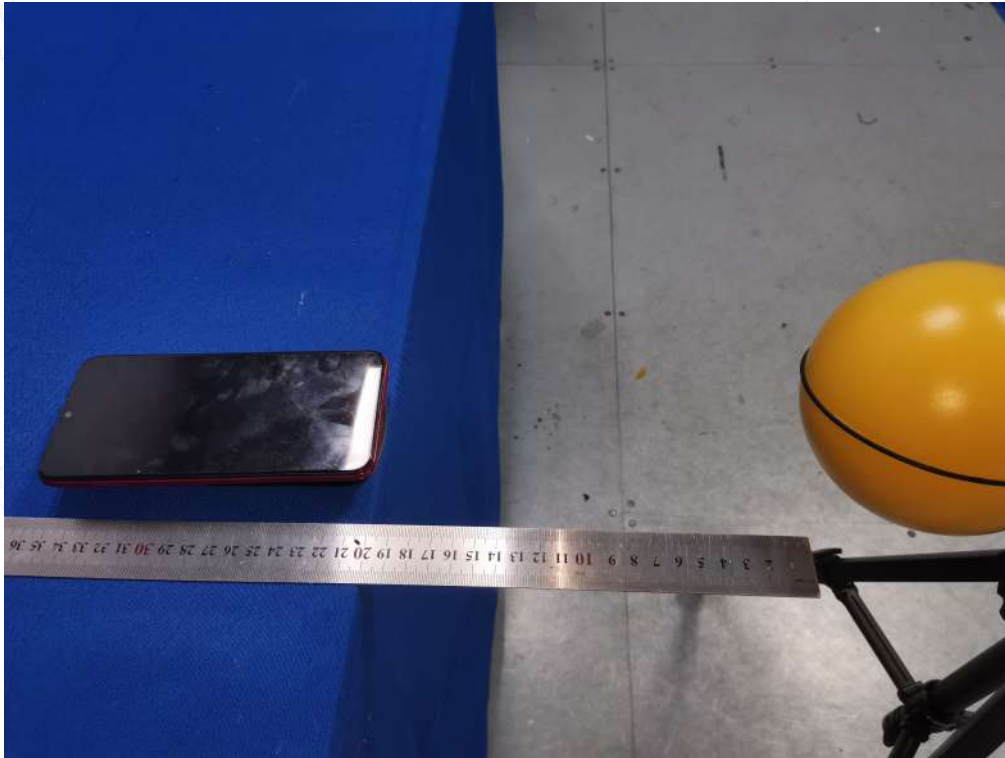
Test Position B(20cm) - Exposure photo from side edge surface-Rear(TM1)
