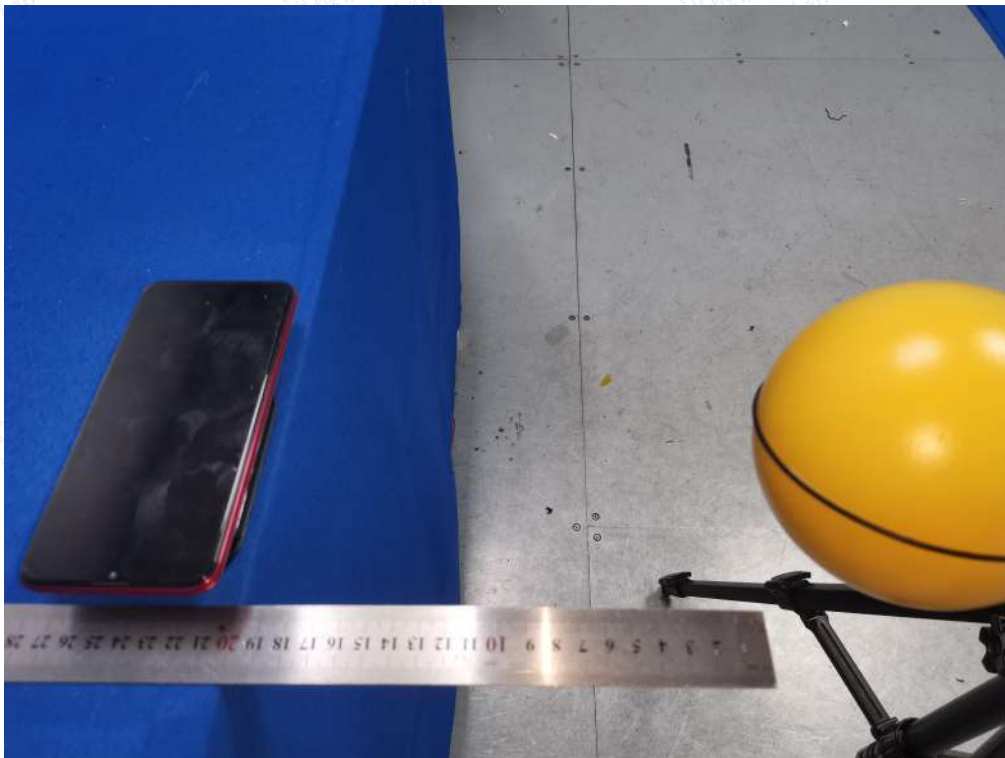
Test Position C(20cm) - Exposure photo from side edge surface-Left(TM1)
