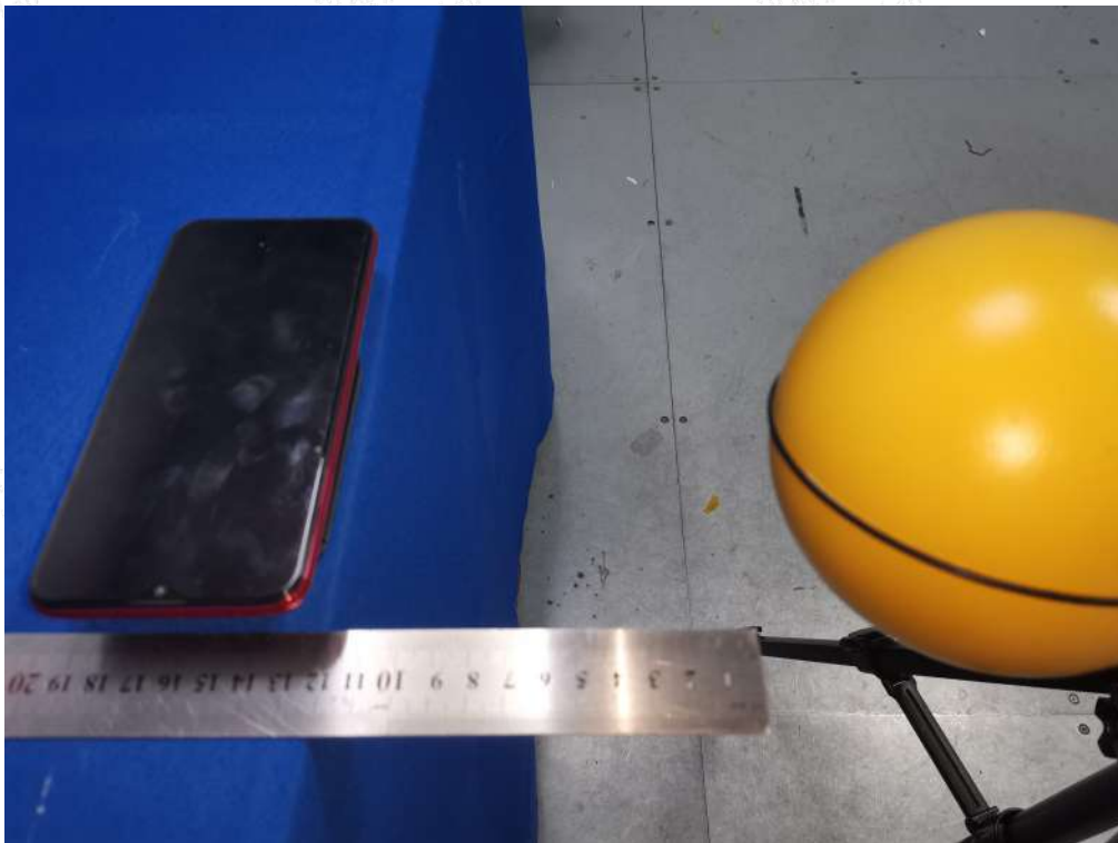
Test Position C(12cm) - Exposure photo from side edge surface-Left(TM1)
