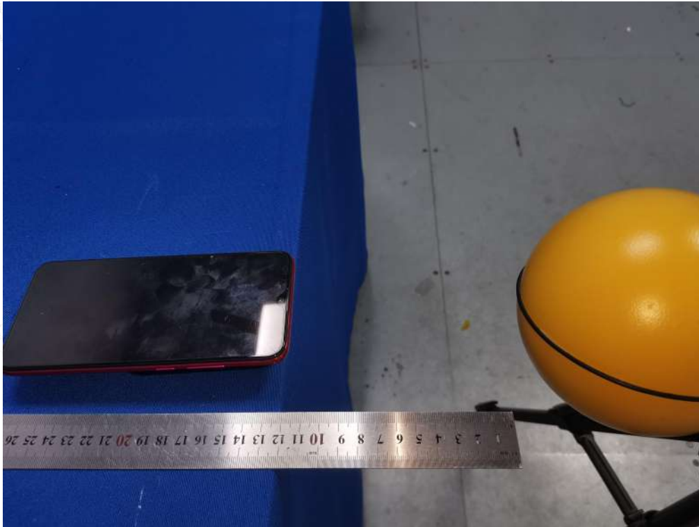
Test Position D(12cm) - Exposure photo from side edge surface-Front(TM1)
