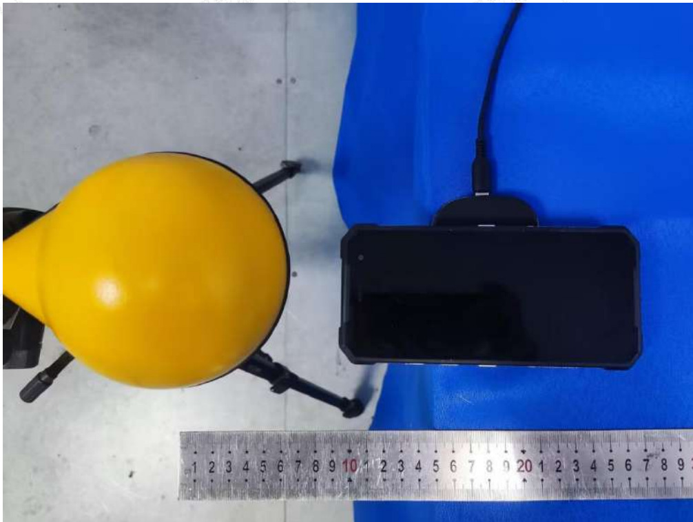
Test Position C(15cm) - Exposure photo from side edge surface-Left(TM1)
