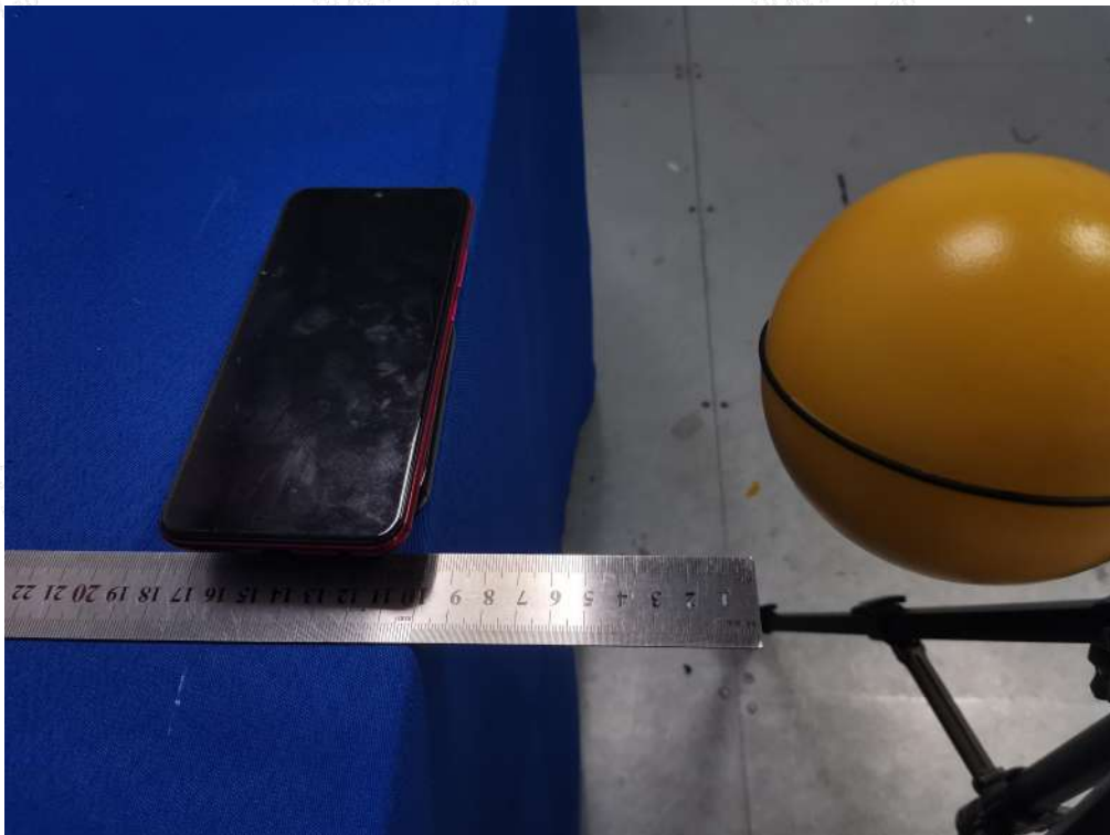
Test Position C(10cm) - Exposure photo from side edge surface-Left(TM1)
