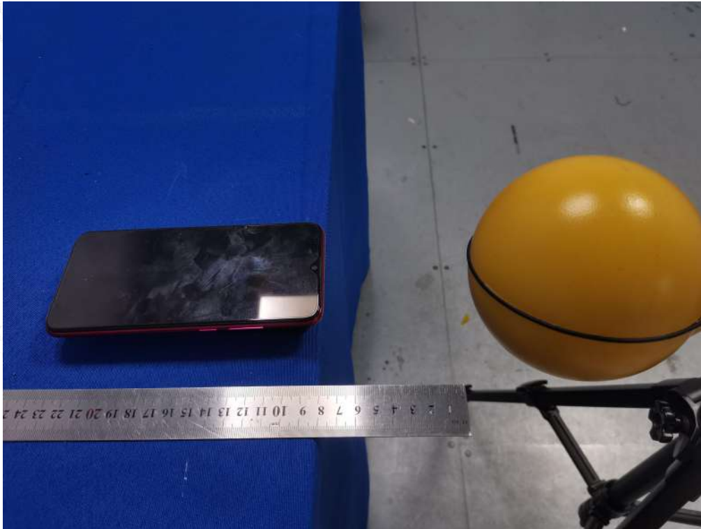
Test Position D(8cm) - Exposure photo from side edge surface-Front(TM1)
