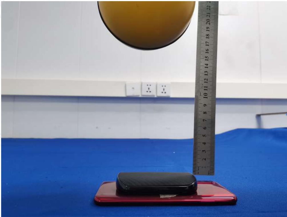
Test Position F(16cm) - Exposure photo from bottom surface(TM1)
