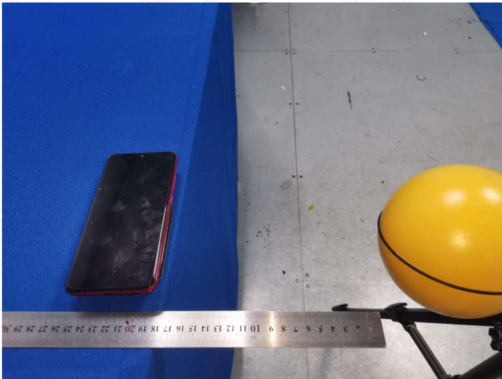
Test Position C(18cm) - Exposure photo from side edge surface-Left(TM1)
