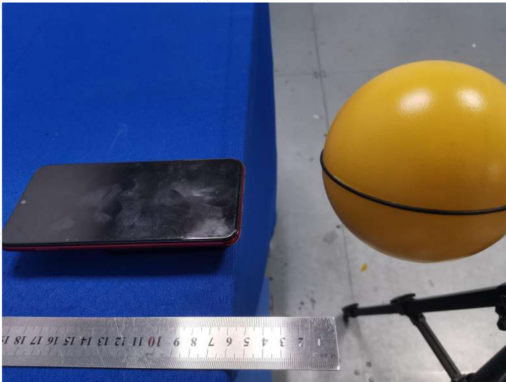
Test Position E(6cm) - Exposure photo from side edge surface-Right(TM1)
