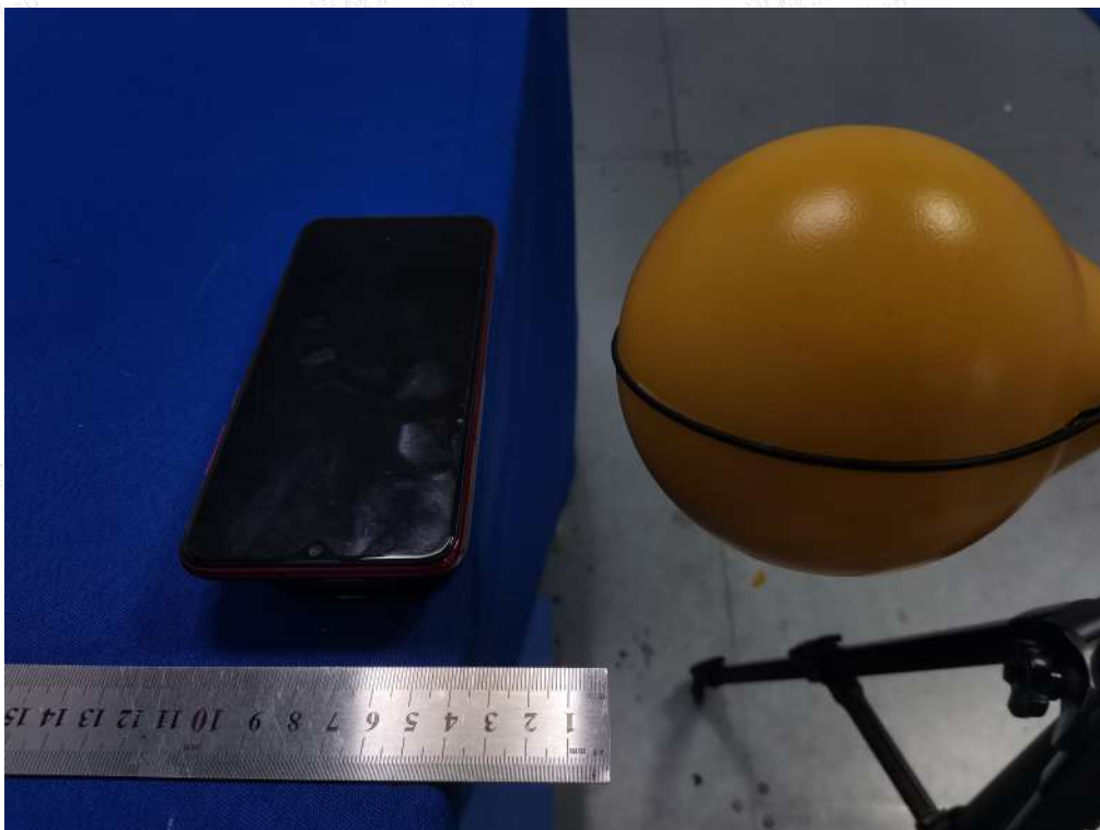
Test Position C(4cm) - Exposure photo from side edge surface-Left(TM1)
