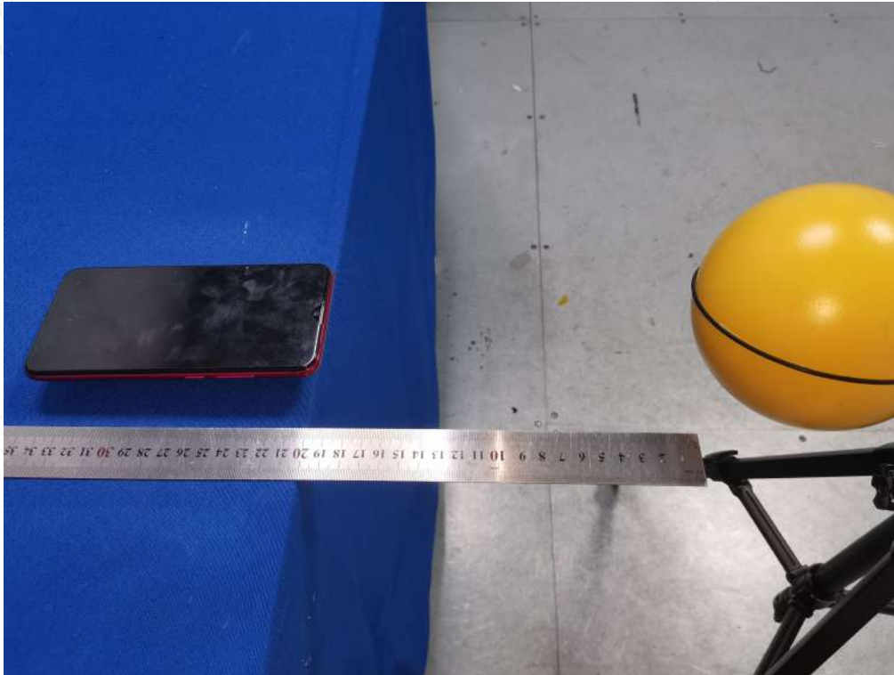
Test Position D(20cm) - Exposure photo from side edge surface-Front(TM1)
