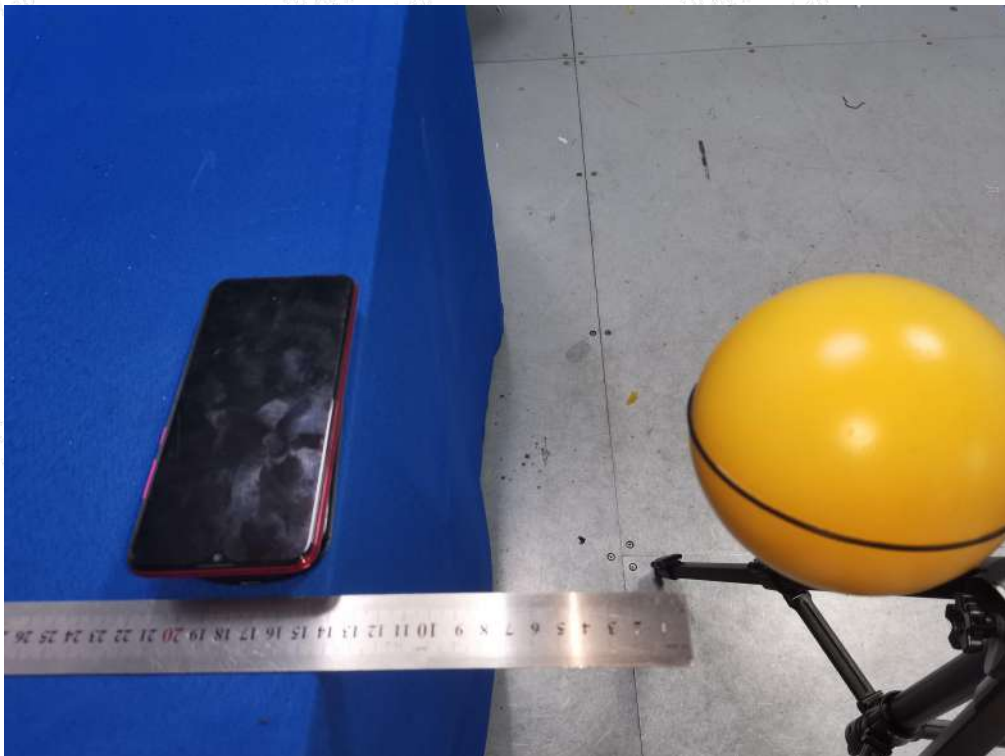
Test Position C(14cm) - Exposure photo from side edge surface-Left(TM1)
