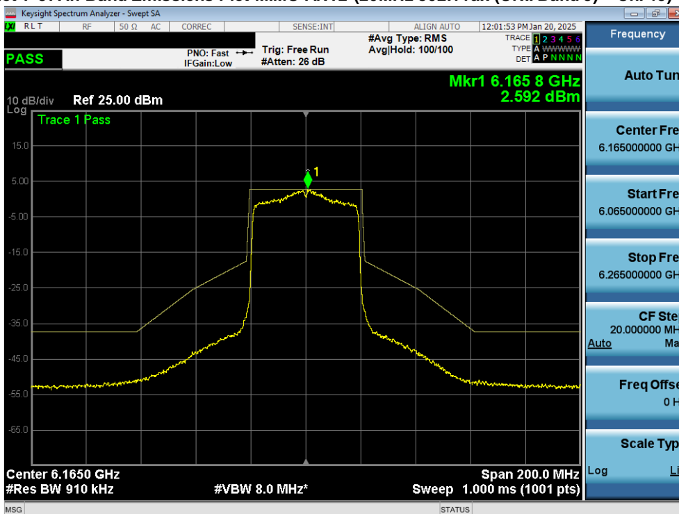
Plot 7-58. In Band Emissions Plot MIMO ANT2 (40MHz 802.11ax (UNII Band 5) – Ch. 43) – SP
