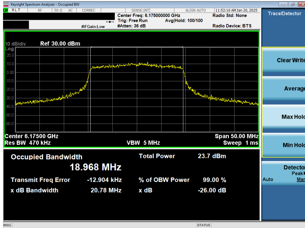
Plot 7-17. 26dB Bandwidth Plot MIMO ANT2 (20MHz 802.11ax (UNII Band 5) – Ch. 45) - SP
