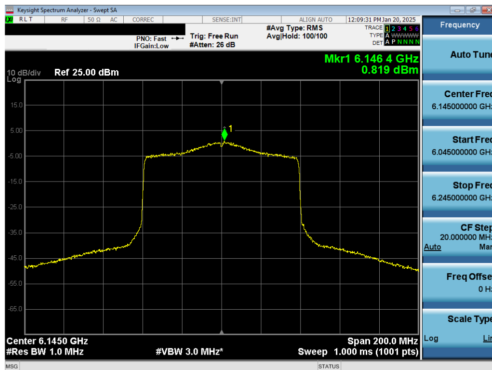
Plot 7-39. Power Spectral Density Plot MIMO ANT2 (80MHz 802.11ax (UNII Band 5) – Ch. 39) – SP
