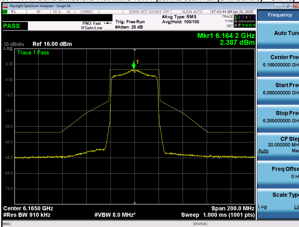
Plot 7-48. In Band Emissions Plot MIMO ANT1 (40MHz 802.11ax (UNII Band 5) – Ch. 43) – SP
