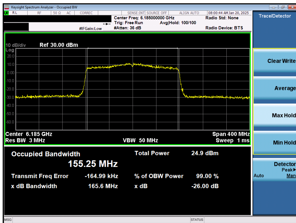
Plot 7-10. 26dB Bandwidth Plot MIMO ANT1 (160MHz 802.11ax (UNII Band 5) – Ch. 47) – SP
