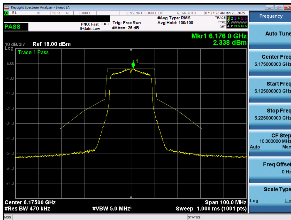
Plot 7-46. In Band Emissions Plot MIMO ANT1 (20MHz 802.11a (UNII Band 5) – Ch. 45) – SP
