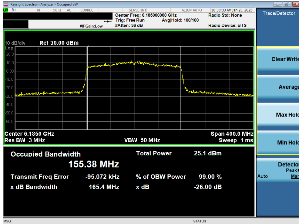
Plot 7-15. 26dB Bandwidth Plot MIMO ANT2 (160MHz 802.11ax (UNII Band 5) – Ch. 47) – LPI
