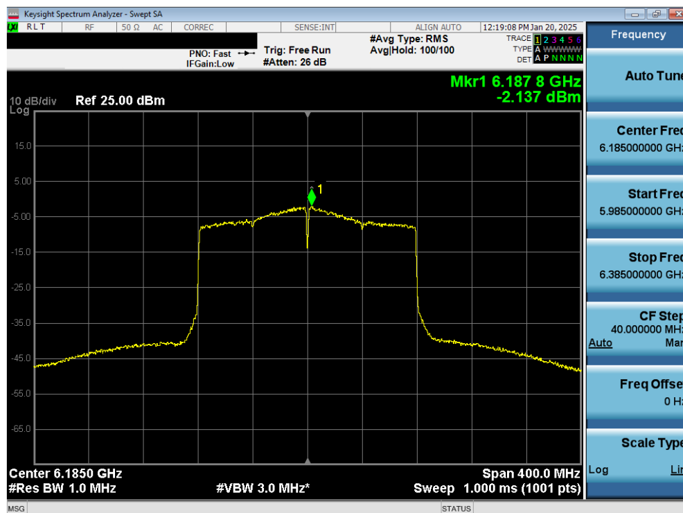
Plot 7-40. Power Spectral Density Plot MIMO ANT2 (160MHz 802.11ax (UNII Band 5) – Ch. 47) – SP
