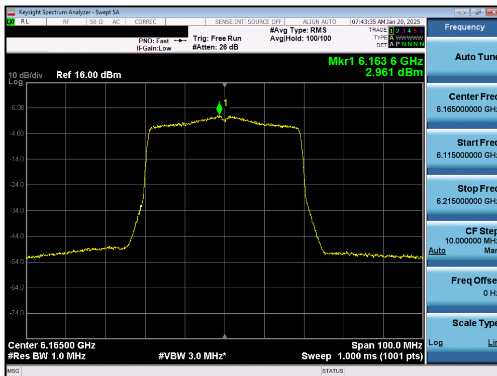
Plot 7-28. Power Spectral Density Plot MIMO ANT1 (40MHz 802.11ax (UNII Band 5) – Ch. 43) – SP
