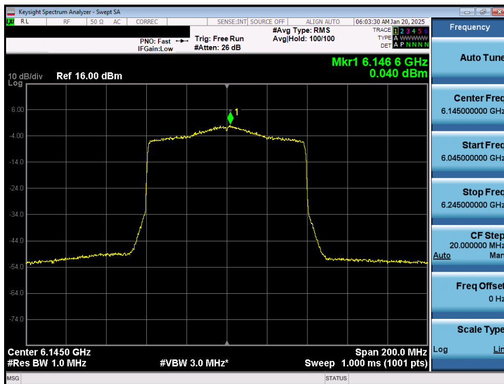
Plot 7-24. Power Spectral Density Plot MIMO ANT1 (80MHz 802.11 ax (UNII Band 5) – Ch. 39) – LPI
