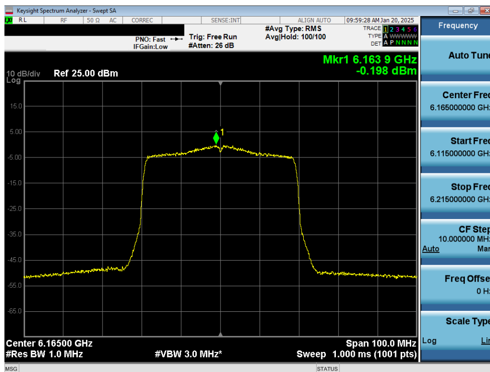
Plot 7-33. Power Spectral Density Plot MIMO ANT2 (40MHz 802.11 ax (UNII Band 5) – Ch. 43) – LPI
