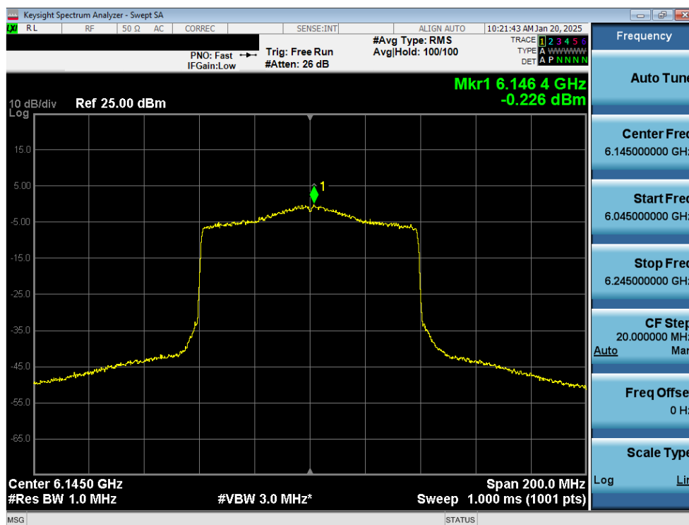
Plot 7-34. Power Spectral Density Plot MIMO ANT2 (80MHz 802.11 ax (UNII Band 5) – Ch. 39) – LPI
