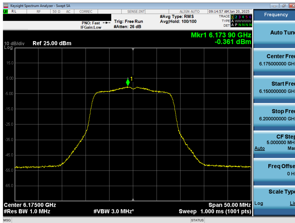
Plot 7-31. Power Spectral Density Plot MIMO ANT2 (20MHz 802.11a (UNII Band 5) – Ch. 45) - LPI
