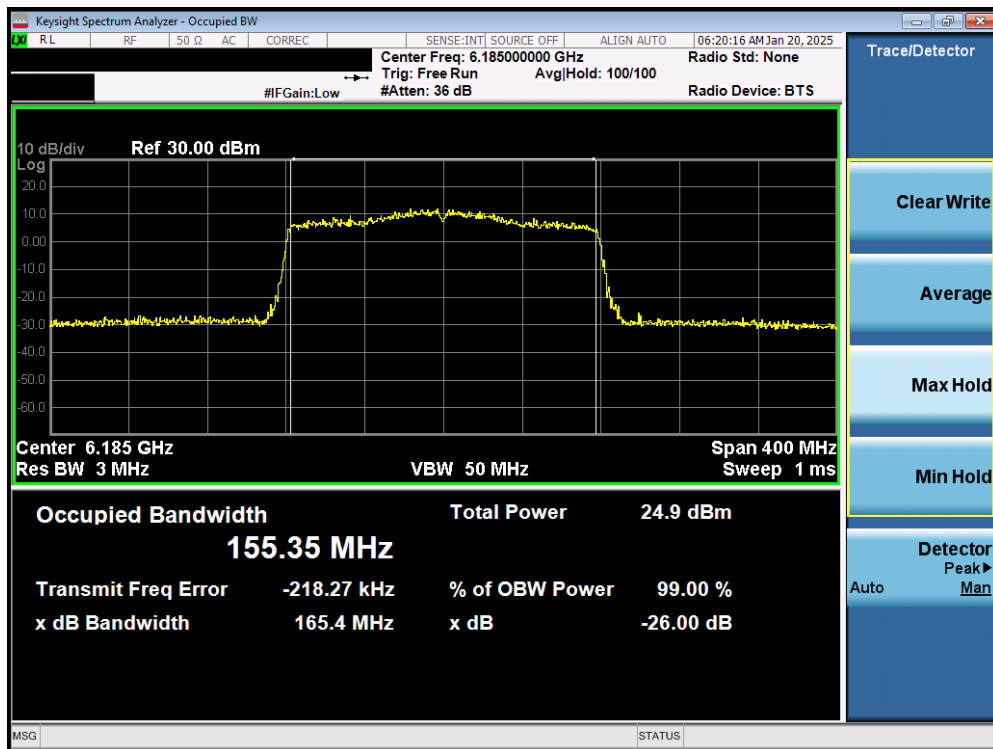
Plot 7-5. 26dB Bandwidth Plot MIMO ANT1 (160MHz 802.11ax (UNII Band 5) – Ch. 47) – LPI
