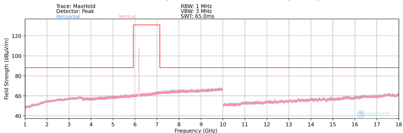
Plot 7-82. Radiated Spurious Plot 1GHz – 18GHz MIMO (802.11a – UNII Band 5 Ch. 45)
