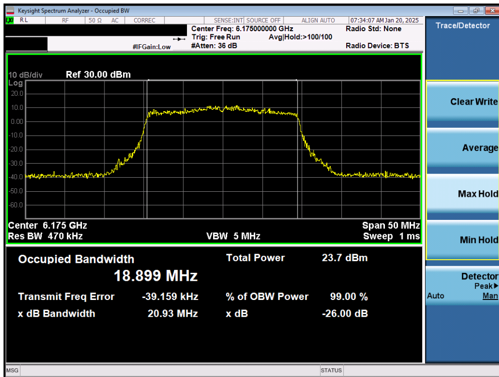
Plot 7-7. 26dB Bandwidth Plot MIMO ANT1 (20MHz 802.11ax (UNII Band 5) – Ch. 45) - SP
