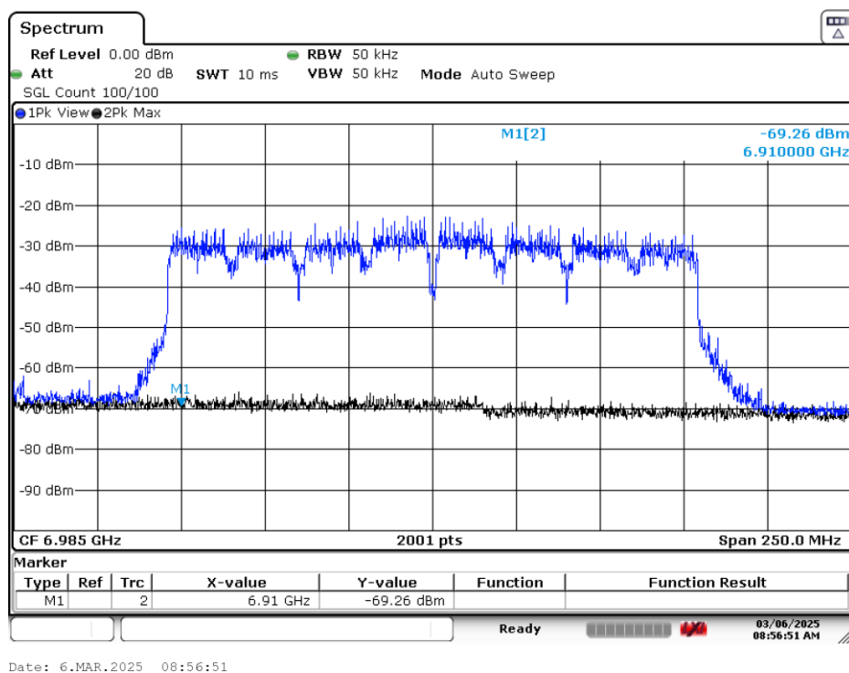
Plot 7-78. CBP 160MHz Channel - Injection Lower Edge – [6910 MHz]
