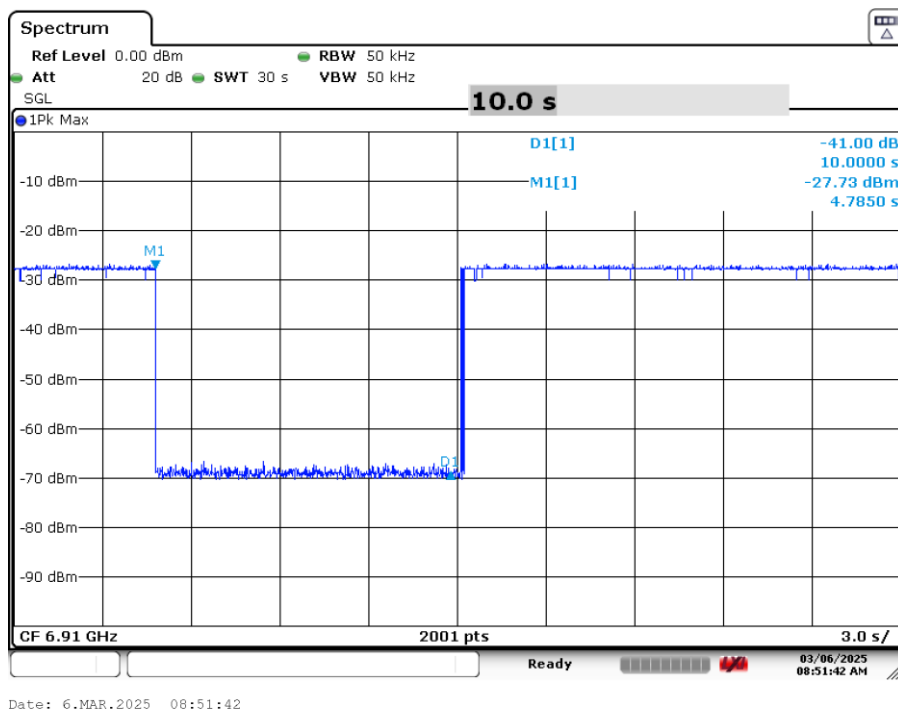
Plot 7-75. Contention Based Protocol Timing Plot (160MHz (UNII Band 8) – Ch. 207 Low)
