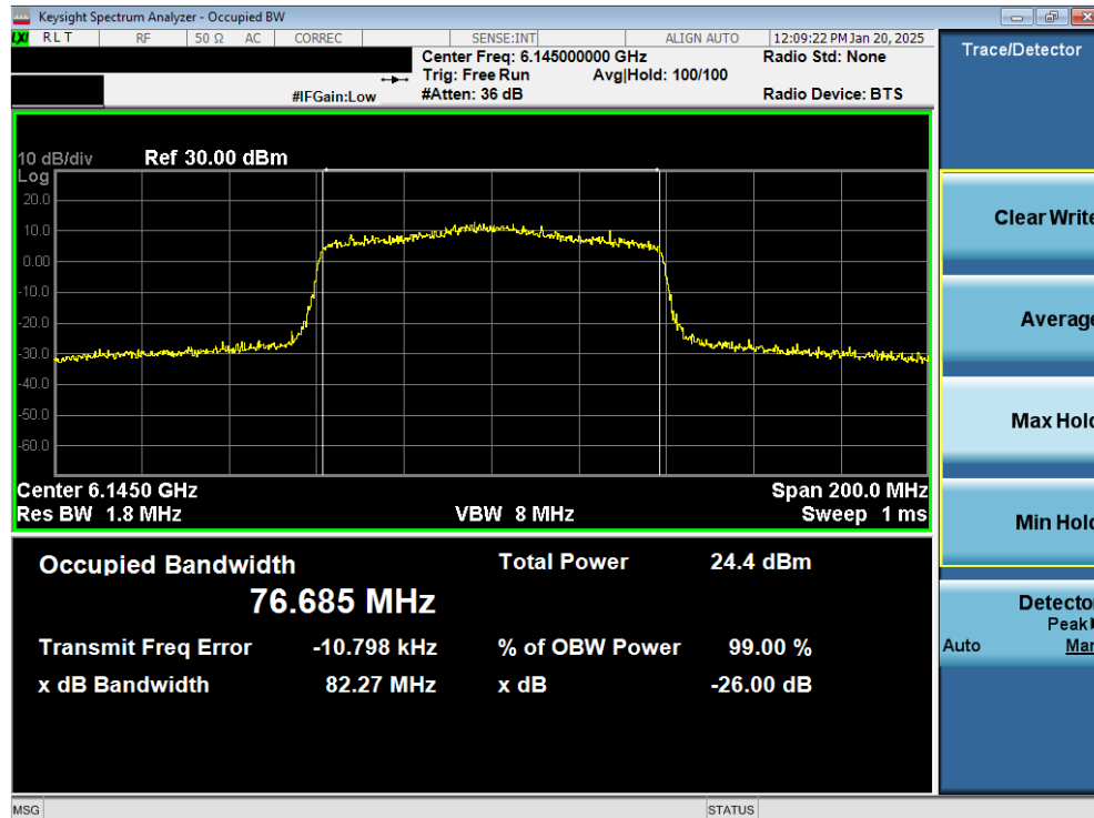
Plot 7-19. 26dB Bandwidth Plot MIMO ANT2 (80MHz 802.11ax (UNII Band 5) – Ch. 39) – SP
