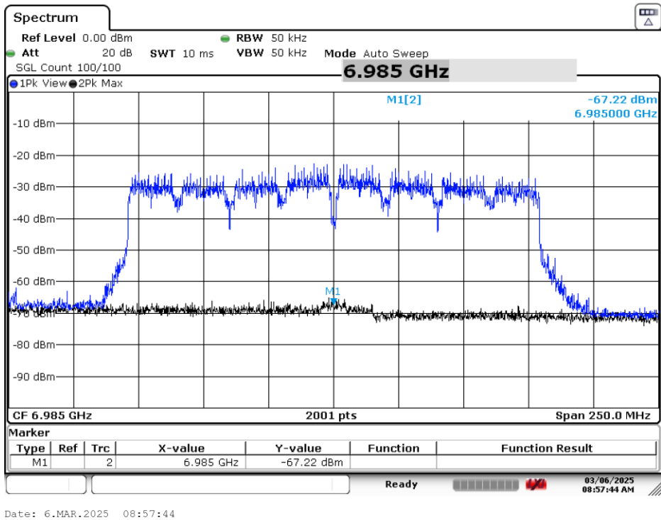
Plot 7-79. CBP 160MHz Channel - Injection Center – [6985 MHz]
