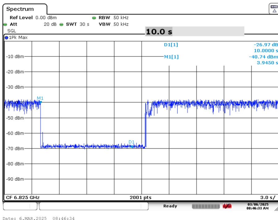
Plot 7-72. Contention Based Protocol Timing Plot (160MHz (UNII Band 7) – Ch. 175 Mid)
