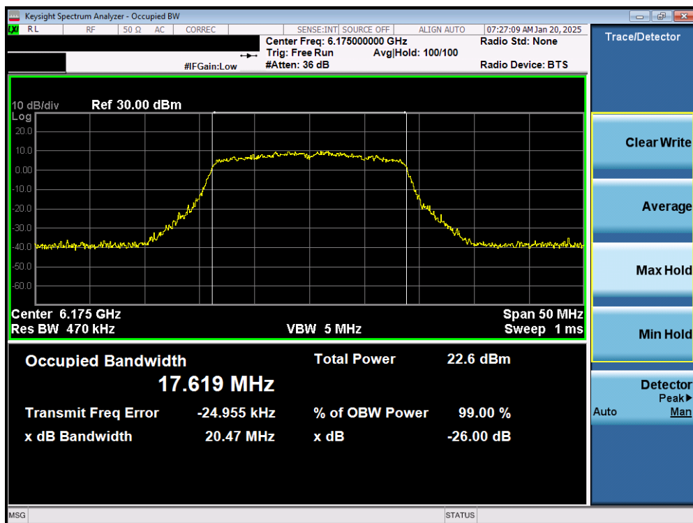
Plot 7-6. 26dB Bandwidth Plot MIMO ANT1 (20MHz 802.11a (UNII Band 5) – Ch. 45) - SP
