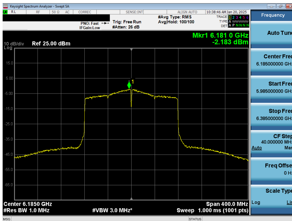
Plot 7-35. Power Spectral Density Plot MIMO ANT2 (160MHz 802.11ax (UNII Band 5) – Ch. 47) – LPI
