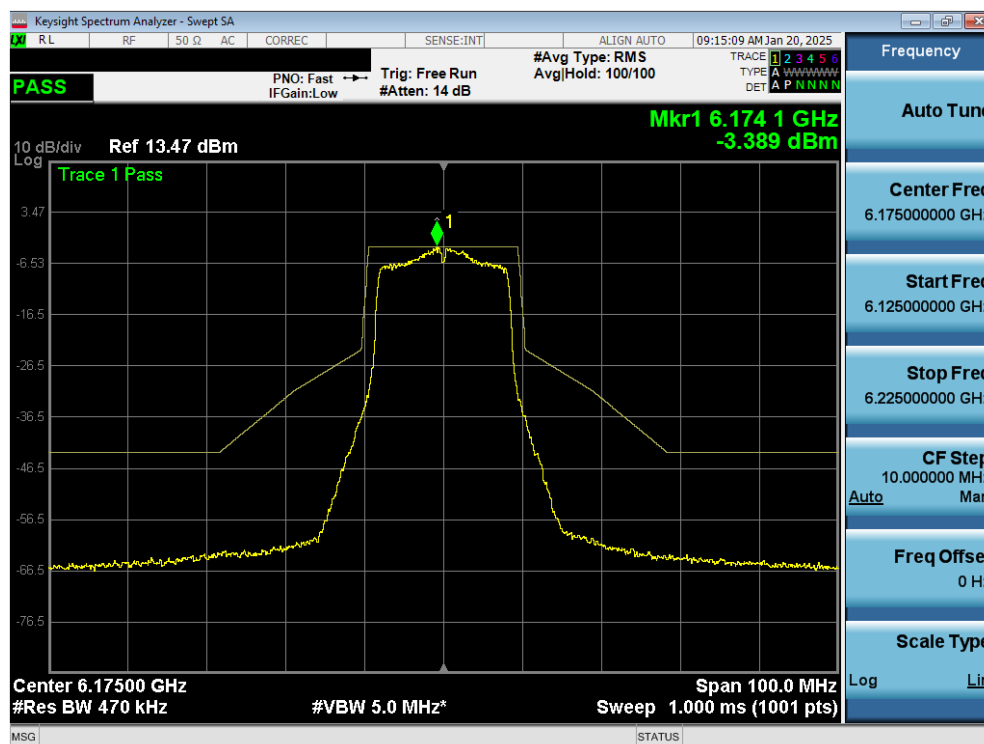
Plot 7-51. In Band Emissions Plot MIMO ANT2 (20MHz 802.11a (UNII Band 5) – Ch. 45) - LPI
