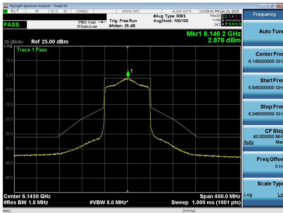
Plot 7-59. In Band Emissions Plot MIMO ANT2 (80MHz 802.11ax (UNII Band 5) – Ch. 39) – SP
