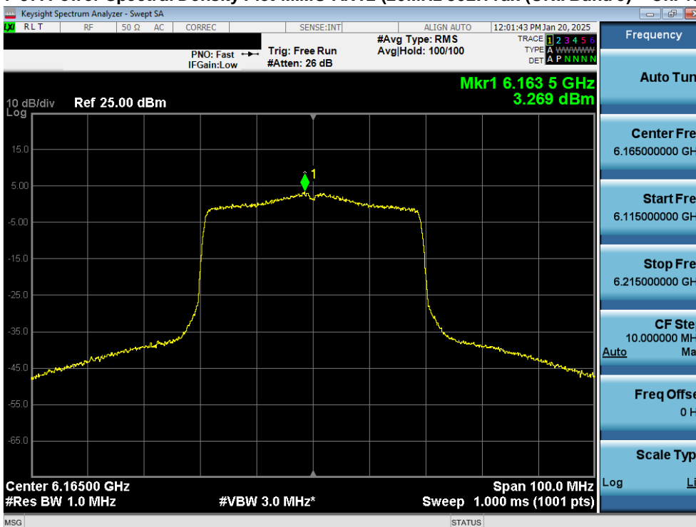
Plot 7-38. Power Spectral Density Plot MIMO ANT2 (40MHz 802.11ax (UNII Band 5) – Ch. 43) - SP
