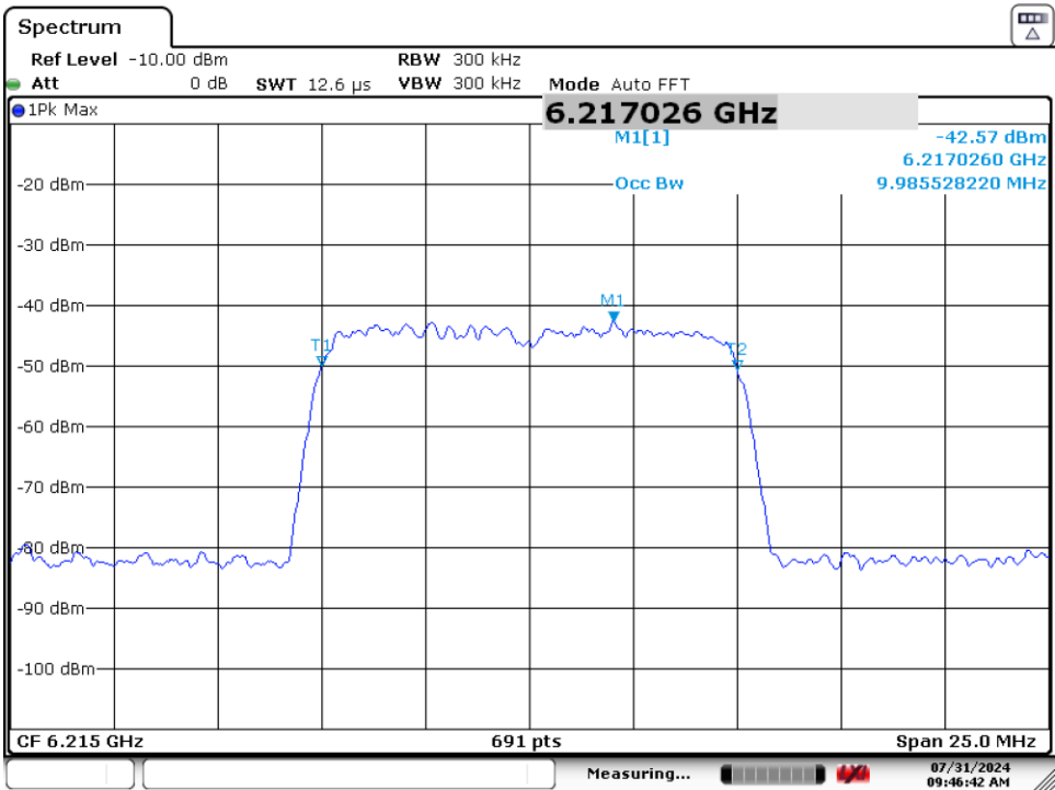
Plot 7-61. AWGN Signal (Demonstration)
