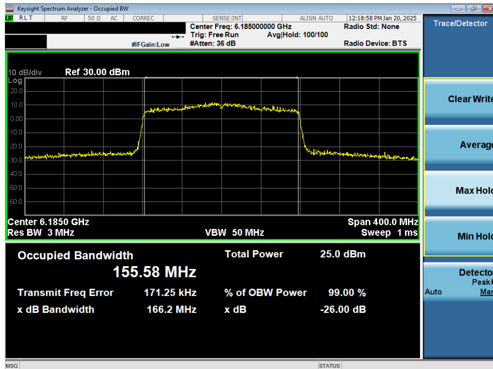
Plot 7-20. 26dB Bandwidth Plot MIMO ANT2 (160MHz 802.11ax (UNII Band 5) – Ch. 47) – SP
