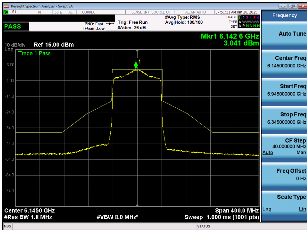
Plot 7-49. In Band Emissions Plot MIMO ANT1 (80MHz 802.11ax (UNII Band 5) – Ch. 39) – SP
