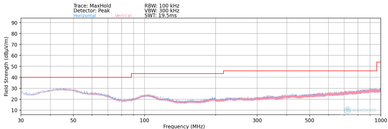
Plot 7-81. Radiated Spurious Plot below 1GHz MIMO (802.11a)
