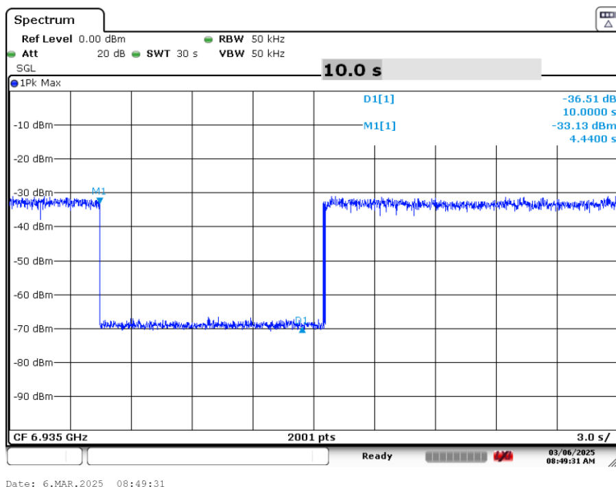
Plot 7-74. Contention Based Protocol Timing Plot (20MHz (UNII Band 8) – Ch. 197)
