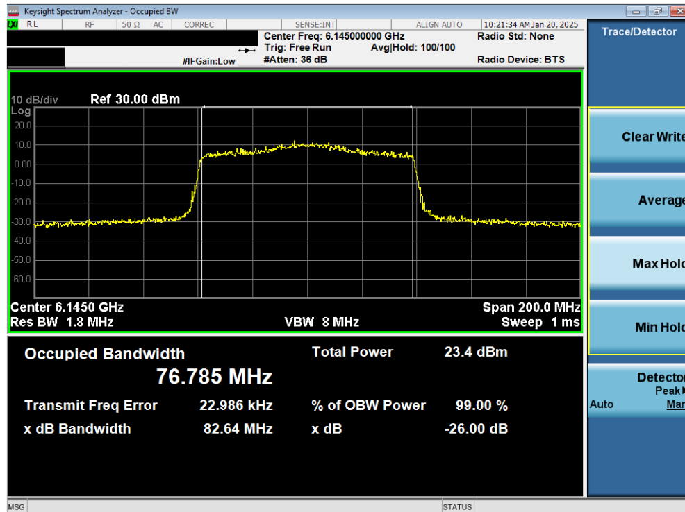
Plot 7-14. 26dB Bandwidth Plot MIMO ANT2 (80MHz 802.11ax (UNII Band 5) – Ch. 39) - LPI
