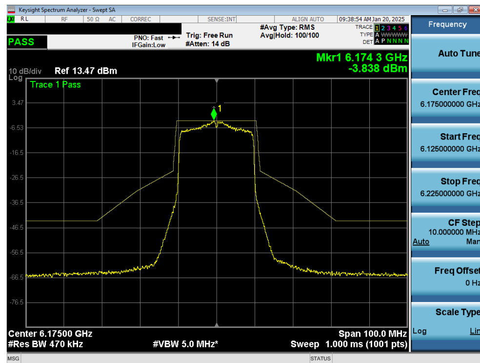
Plot 7-52. In Band Emissions Plot MIMO ANT2 (20MHz 802.11ax (UNII Band 5) – Ch. 45) - LPI
