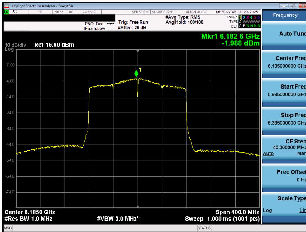
Plot 7-25. Power Spectral Density Plot MIMO ANT1 (160MHz 802.11ax (UNII Band 5) – Ch. 47) – LPI
