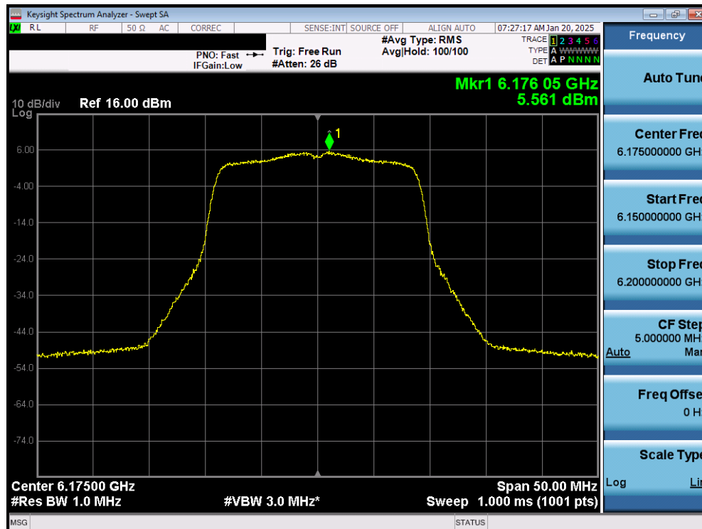
Plot 7-26. Power Spectral Density Plot MIMO ANT1 (20MHz 802.11a (UNII Band 5) – Ch. 45) – SP
