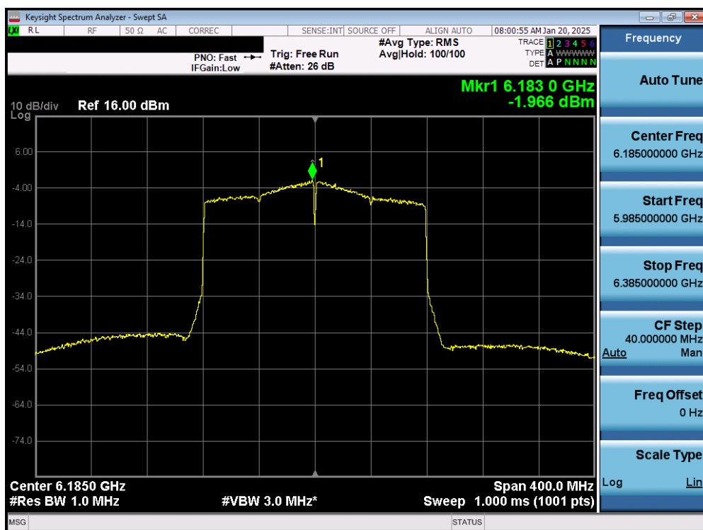
Plot 7-30. Power Spectral Density Plot MIMO ANT1 (160MHz 802.11ax (UNII Band 5) – Ch. 47) – SP
