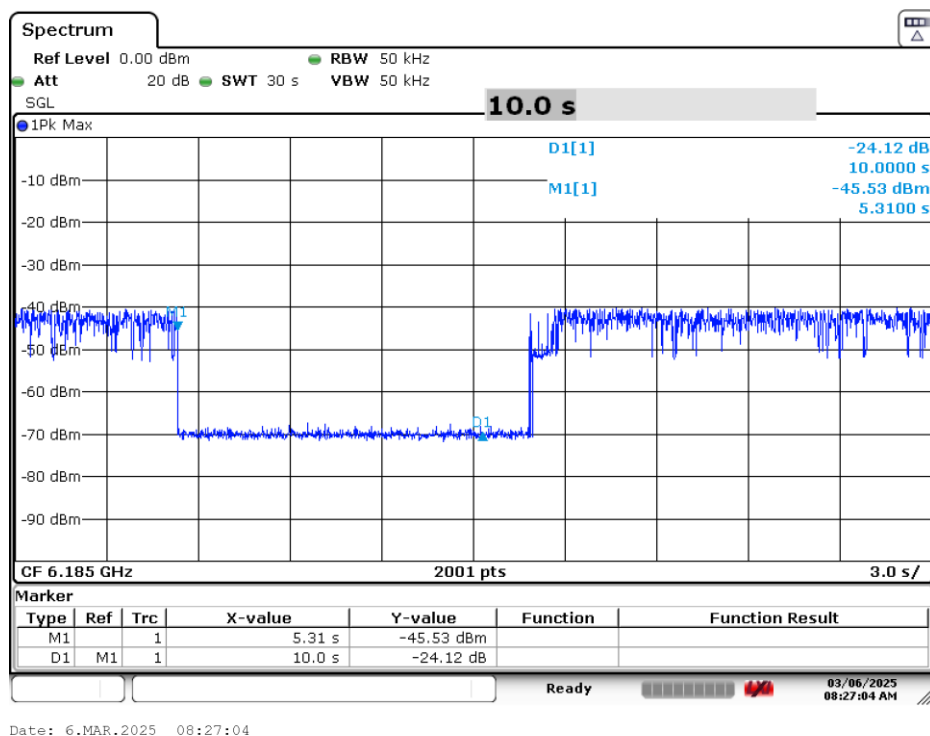
Plot 7-64. Contention Based Protocol Timing Plot (160MHz (UNII Band 5) – Ch. 47 Mid)
