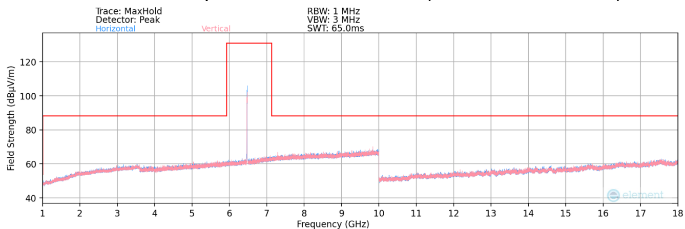
Plot 7-83. Radiated Spurious Plot 1GHz – 18GHz MIMO (802.11a – UNII Band 6 Ch. 105)
