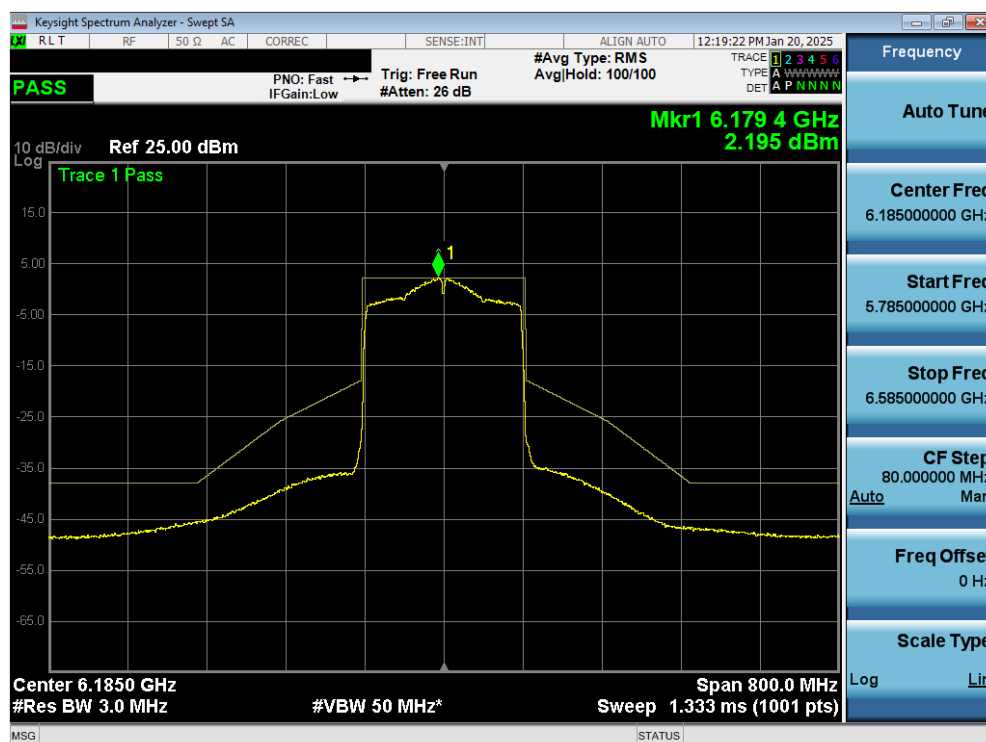
Plot 7-60. In Band Emissions Plot MIMO ANT2 (160MHz 802.11ax (UNII Band 5) – Ch. 47) – SP
