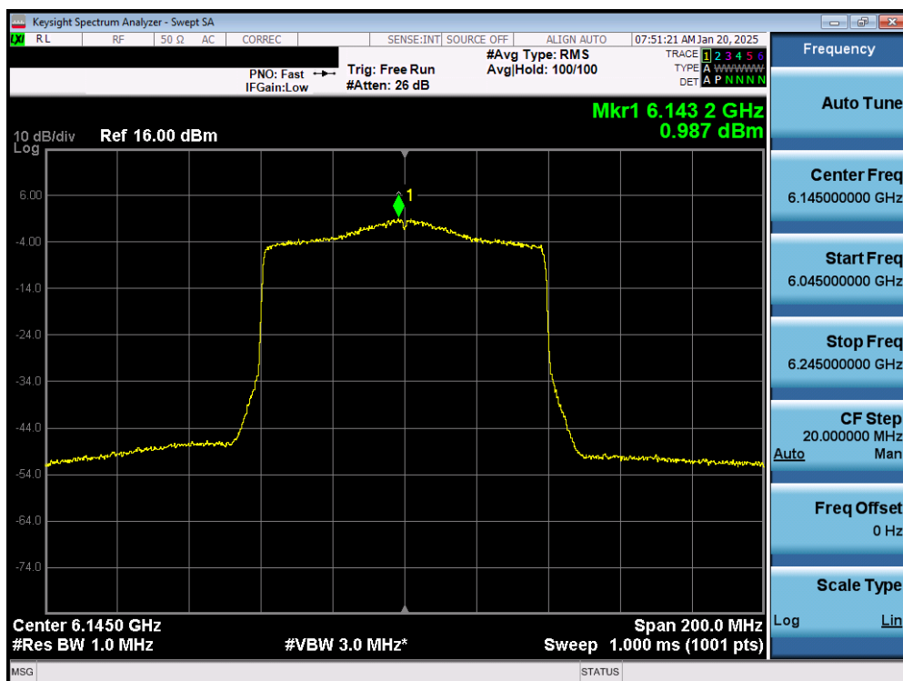
Plot 7-29. Power Spectral Density Plot MIMO ANT1 (80MHz 802.11ax (UNII Band 5) – Ch. 39) – SP
