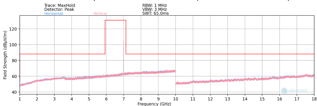
Plot 7-85. Radiated Spurious Plot 1GHz – 18GHz MIMO (802.11a – U Band 8 Ch. 209)
