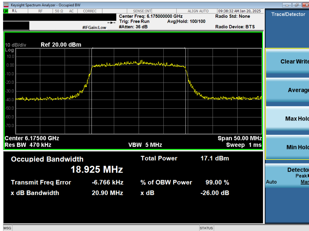
Plot 7-12. 26dB Bandwidth Plot MIMO ANT2 (20MHz 802.11ax (UNII Band 5) – Ch. 45) - LPI
