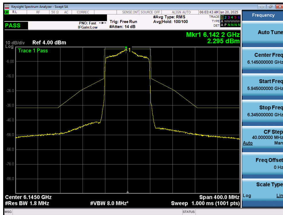
Plot 7-44. In Band Emissions Plot MIMO ANT1 (80MHz 802.11ax (UNII Band 5) – Ch. 39) – LPI
