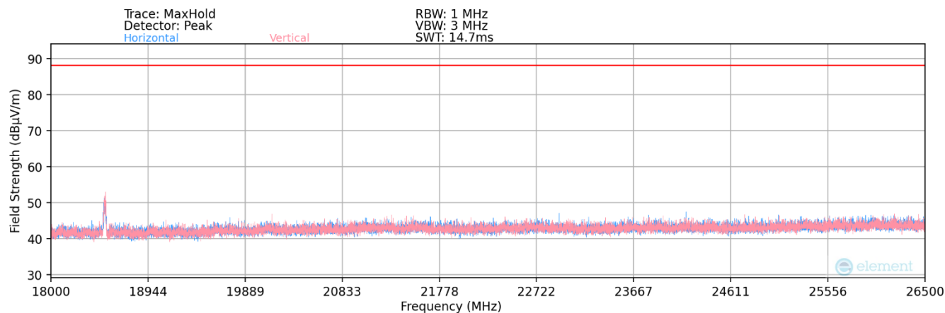
Plot 7-86. Radiated Spurious Plot 18GHz - 26.5GHz (802.11a)
