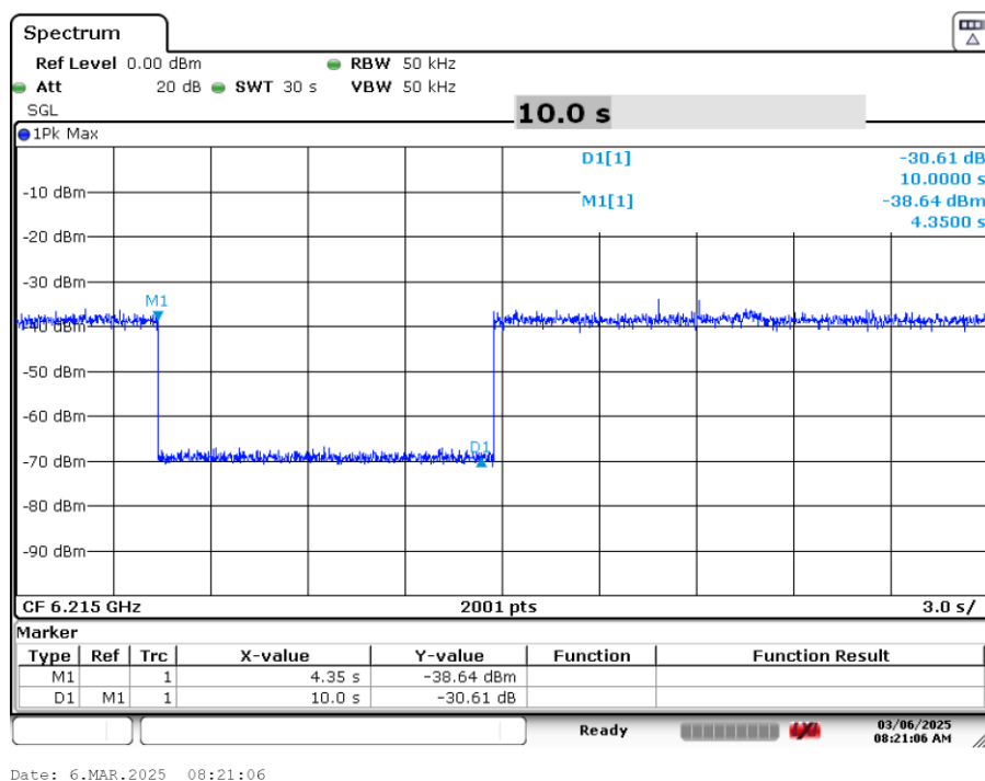
Plot 7-62. Contention Based Protocol Timing Plot (20MHz (UNII Band 5) – Ch. 53)
