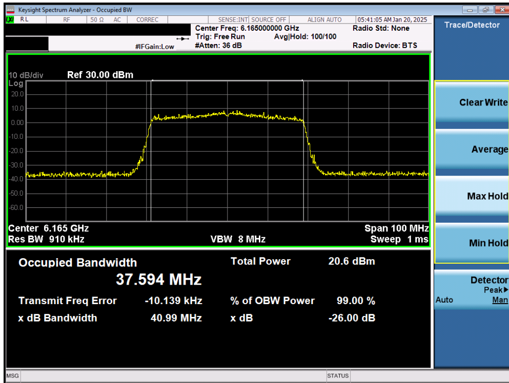
Plot 7-3. 26dB Bandwidth Plot MIMO ANT1 (40MHz 802.11ax (UNII Band 5) – Ch. 43) – LPI
