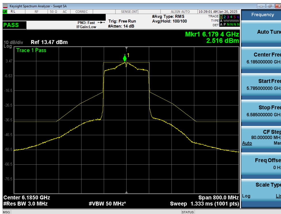
Plot 7-55. In Band Emissions Plot MIMO ANT2 (160MHz 802.11ax (UNII Band 5) – Ch. 47) – LPI
