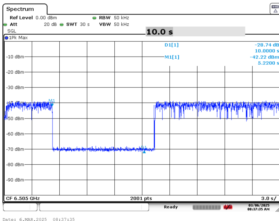
Plot 7-68. Contention Based Protocol Timing Plot (160MHz (UNII Band 6) – Ch. 111 Mid)
