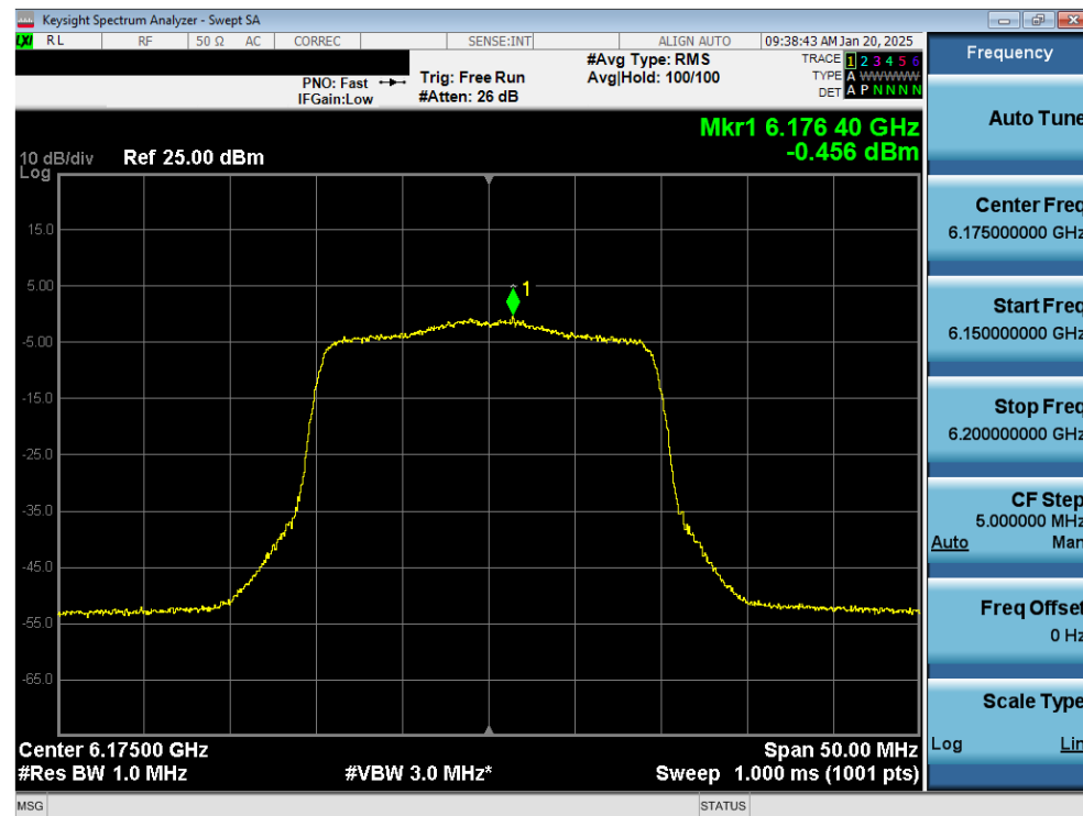
Plot 7-32. Power Spectral Density Plot MIMO ANT2 (20MHz 802.11ax (UNII Band 5) – Ch. 45) - LPI
