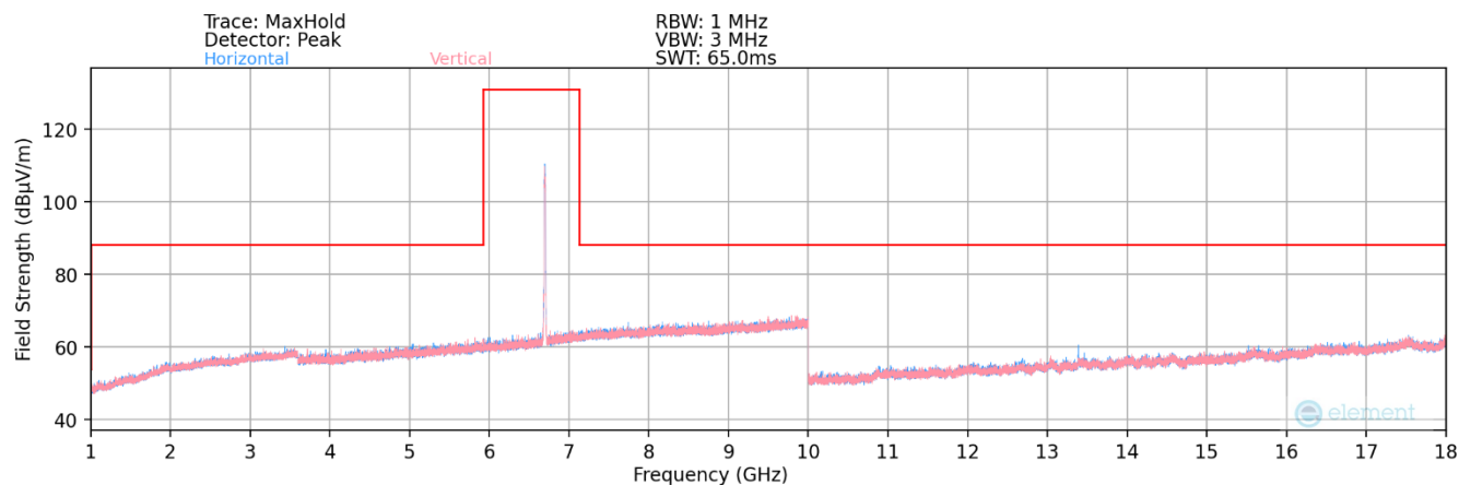
Plot 7-84. Radiated Spurious Plot 1GHz – 18GHz MIMO (802.11a – UNII Band 7 Ch. 149)
