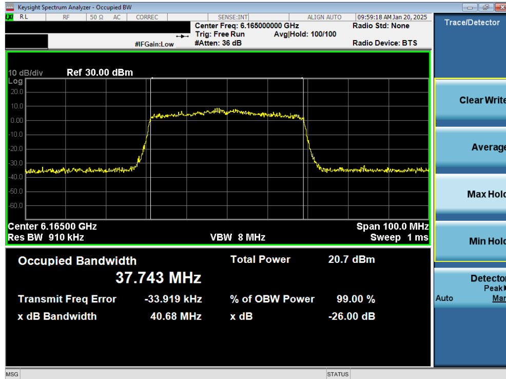
Plot 7-13. 26dB Bandwidth Plot MIMO ANT2 (40MHz 802.11ax (UNII Band 5) – Ch. 43) - LPI
