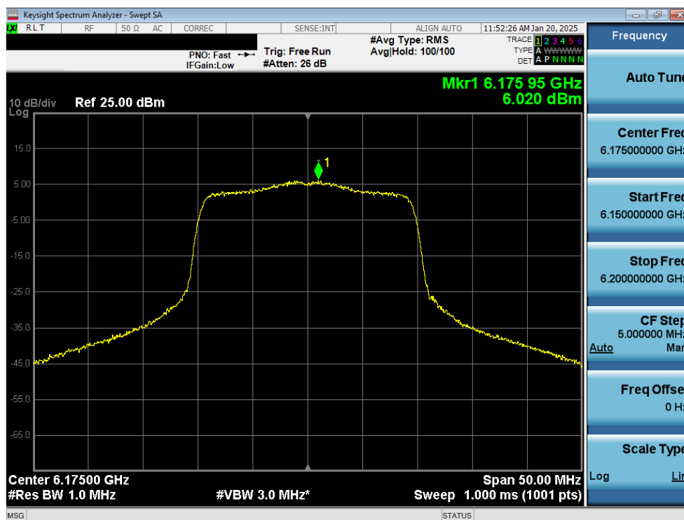
Plot 7-37. Power Spectral Density Plot MIMO ANT2 (20MHz 802.11ax (UNII Band 5) – Ch. 45) - SP
