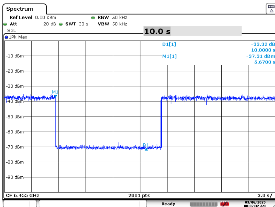
Plot 7-66. Contention Based Protocol Timing Plot (20MHz (UNII Band 6) – Ch. 101)
