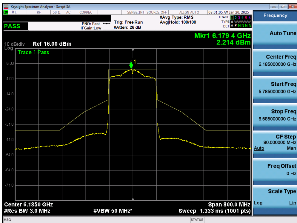
Plot 7-50. In Band Emissions Plot MIMO ANT1 (160MHz 802.11ax (UNII Band 5) – Ch. 47) – SP
