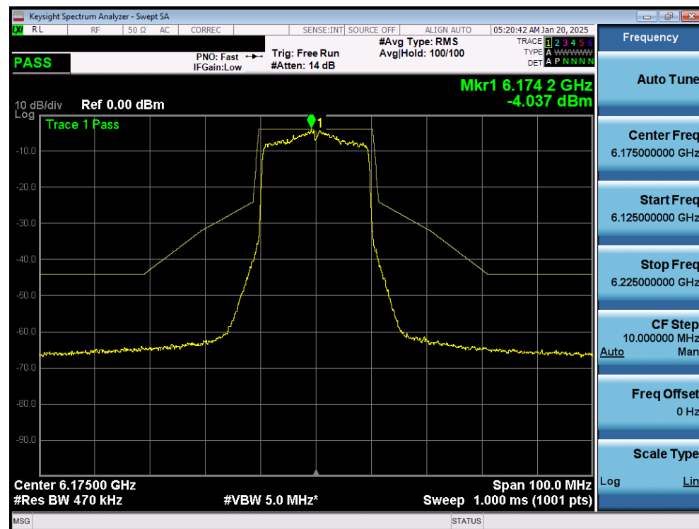
Plot 7-42. In Band Emissions Plot MIMO ANT1 (20MHz 802.11ax (UNII Band 5) – Ch. 45) - LPI
