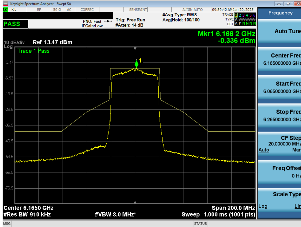
Plot 7-53. In Band Emissions Plot MIMO ANT2 (40MHz 802.11ax (UNII Band 5) – Ch. 43) – LPI
