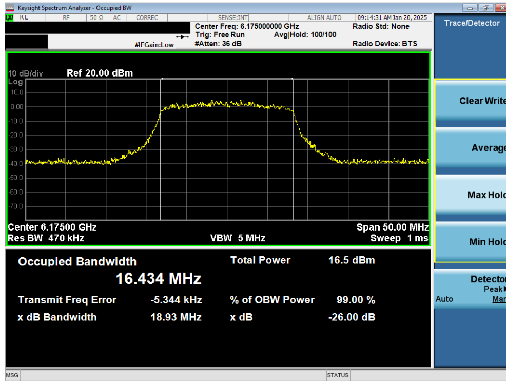
Plot 7-11. 26dB Bandwidth Plot MIMO ANT2 (20MHz 802.11a (UNII Band 5) – Ch. 45) - LPI
