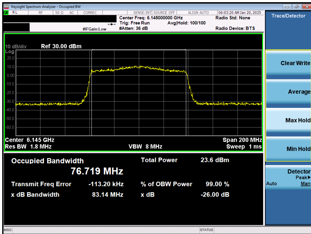
Plot 7-4. 26dB Bandwidth Plot MIMO ANT1 (80MHz 802.11ax (UNII Band 5) – Ch. 39) – LPI
