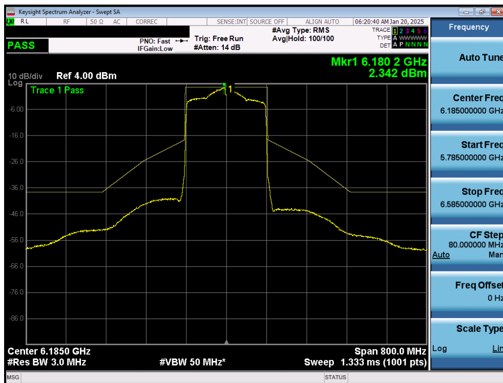
Plot 7-45. In Band Emissions Plot MIMO ANT1 (160MHz 802.11ax (UNII Band 5) – Ch. 47) – LPI
