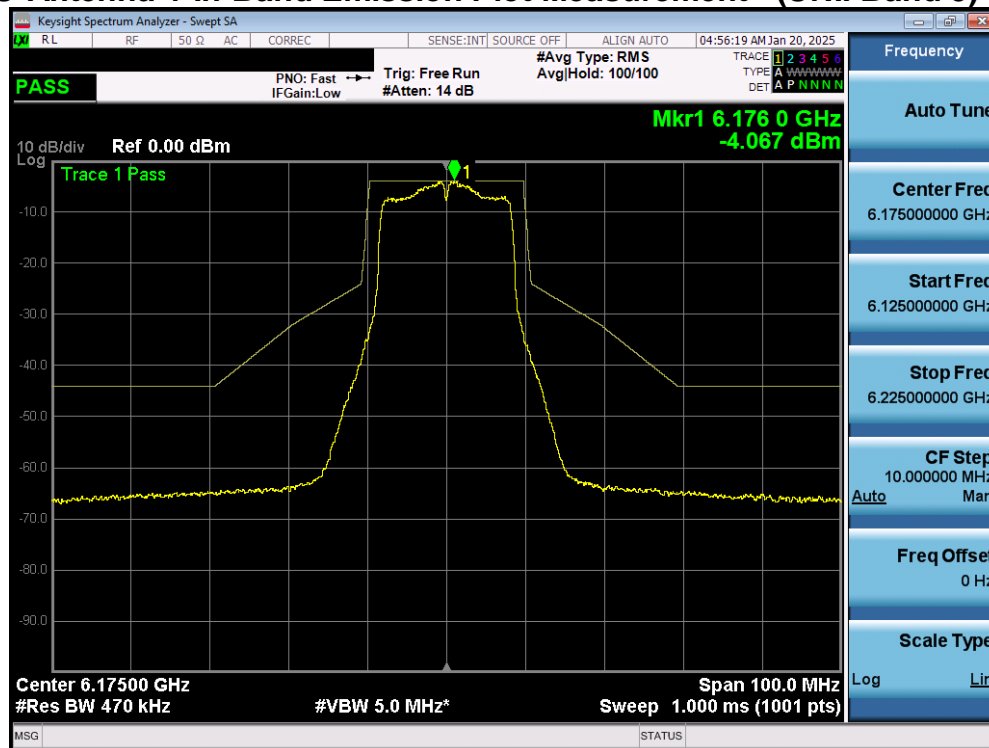
Plot 7-41. In Band Emissions Plot MIMO ANT1 (20MHz 802.11a (UNII Band 5) – Ch. 45) - LPI
