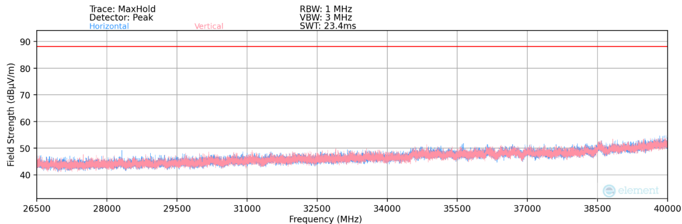
Plot 7-87. Radiated Spurious Plot 26.5GHz - 40GHz (802.11a)
