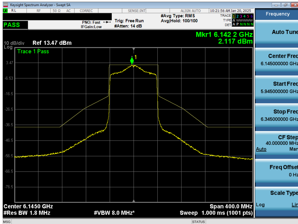
Plot 7-54. In Band Emissions Plot MIMO ANT2 (80MHz 802.11ax (UNII Band 5) – Ch. 39) – LPI
