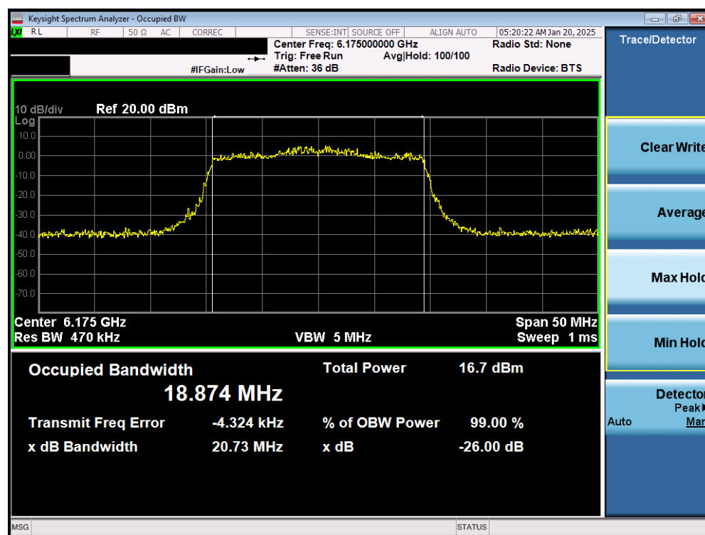
Plot 7-2. 26dB Bandwidth Plot MIMO ANT1 (20MHz 802.11ax (UNII Band 5) – Ch. 45) – LPI
