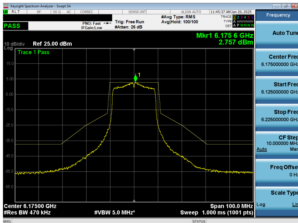
Plot 7-56. In Band Emissions Plot MIMO ANT2 (20MHz 802.11a (UNII Band 5) – Ch. 45) – SP
