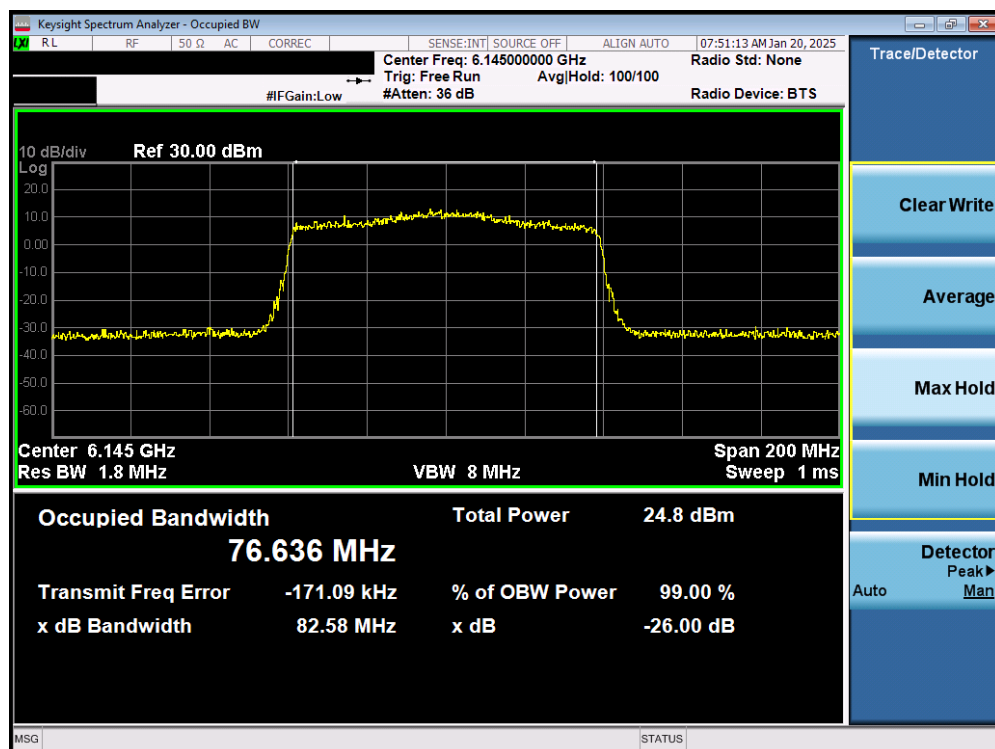
Plot 7-9. 26dB Bandwidth Plot MIMO ANT1 (80MHz 802.11ax (UNII Band 5) – Ch. 39) – SP
