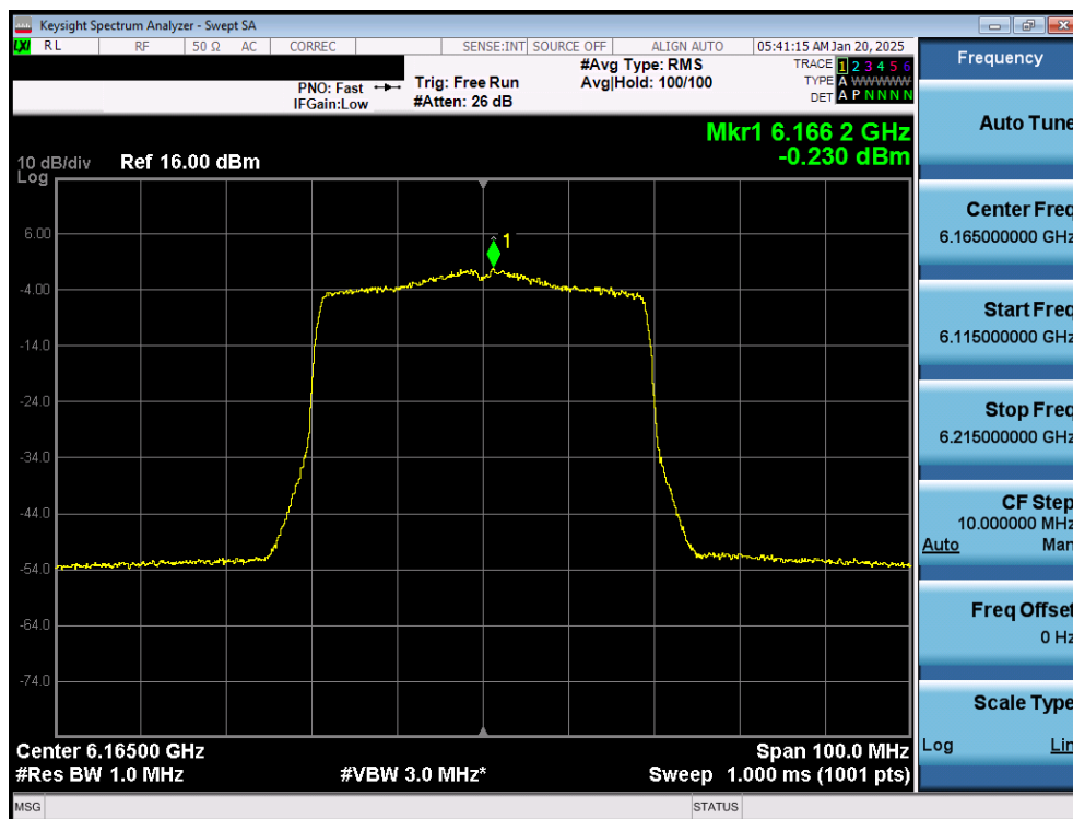
Plot 7-23. Power Spectral Density Plot MIMO ANT1 (40MHz 802.11 ax (UNII Band 5) – Ch. 43) – LPI
