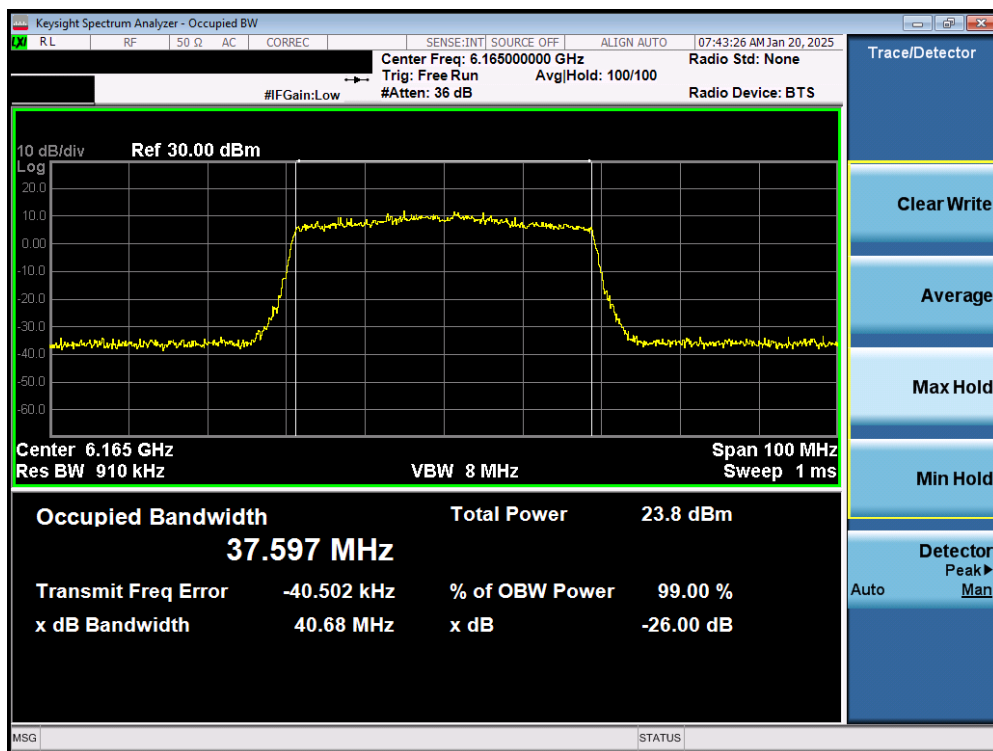
Plot 7-8. 26dB Bandwidth Plot MIMO ANT1 (40MHz 802.11ax (UNII Band 5) – Ch. 43) - SP
