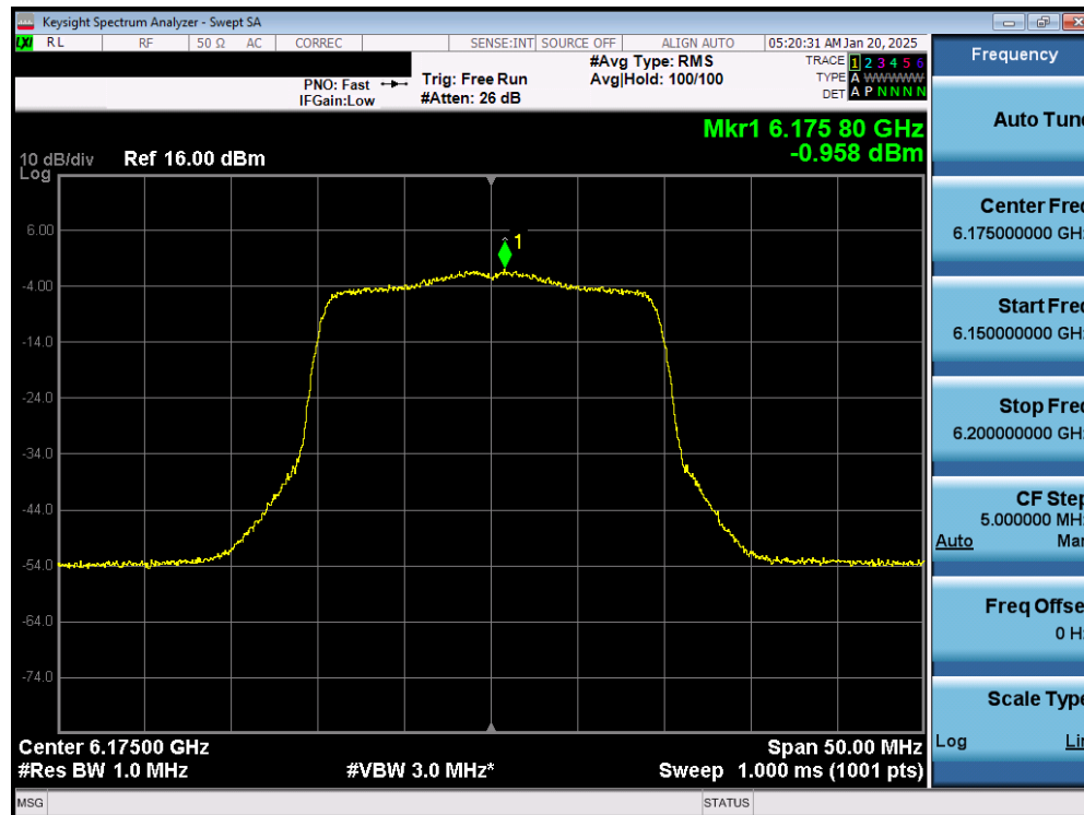
Plot 7-22. Power Spectral Density Plot MIMO ANT1 (20MHz 802.11ax (UNII Band 5) – Ch. 45) – LPI
