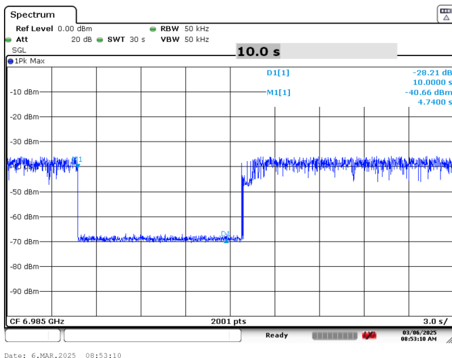
Plot 7-76. Contention Based Protocol Timing Plot (160MHz (UNII Band 8) – Ch. 207 Mid)
