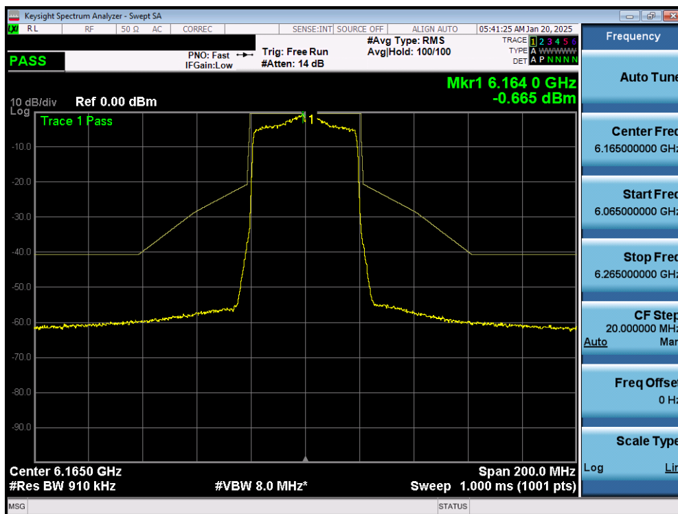
Plot 7-43. In Band Emissions Plot MIMO ANT1 (40MHz 802.11ax (UNII Band 5) – Ch. 43) – LPI
