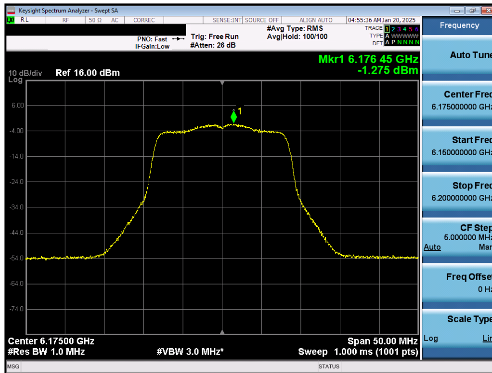
Plot 7-21. Power Spectral Density Plot MIMO ANT1 (20MHz 802.11a (UNII Band 5) – Ch. 45) – LPI
