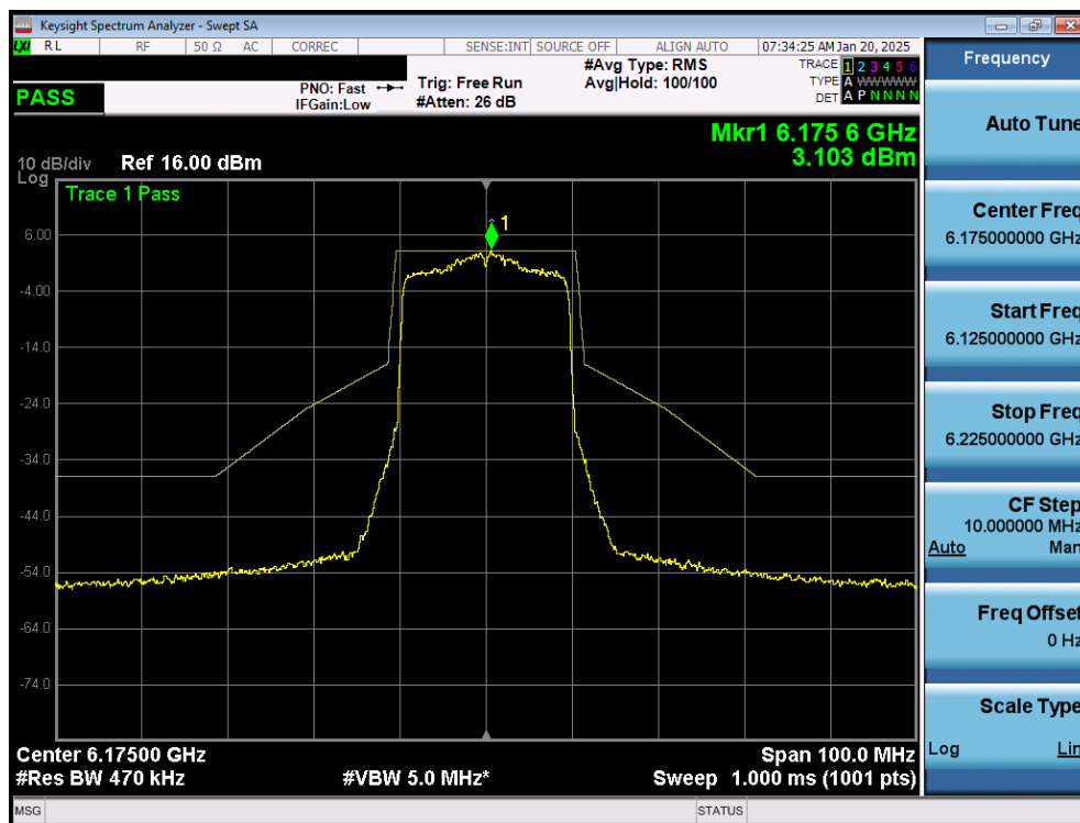
Plot 7-47. In Band Emissions Plot MIMO ANT1 (20MHz 802.11ax (UNII Band 5) – Ch. 45) – SP
