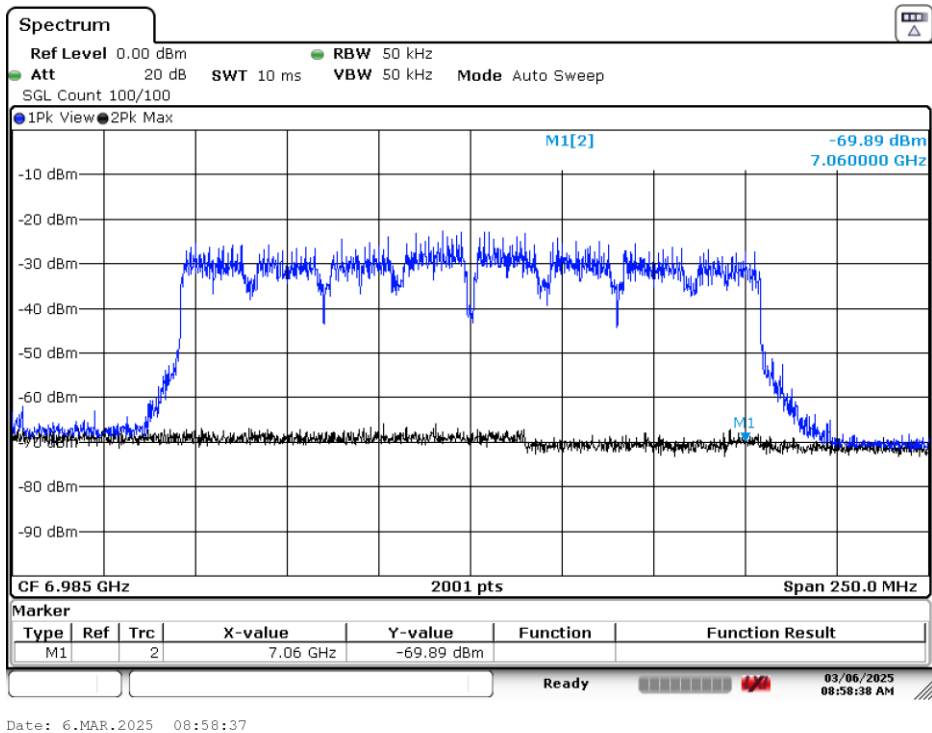
Plot 7-80. CBP 160MHz Channel - Injection Upper Edge – [7060 MHz]
