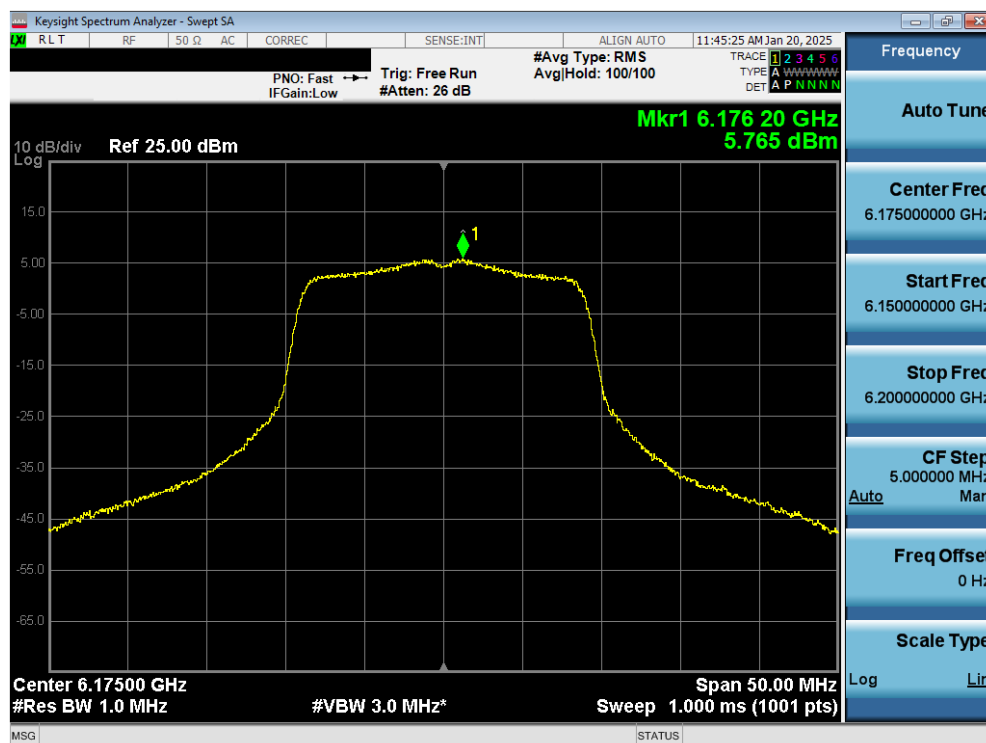
Plot 7-36. Power Spectral Density Plot MIMO ANT2 (20MHz 802.11a (UNII Band 5) – Ch. 45) – SP
