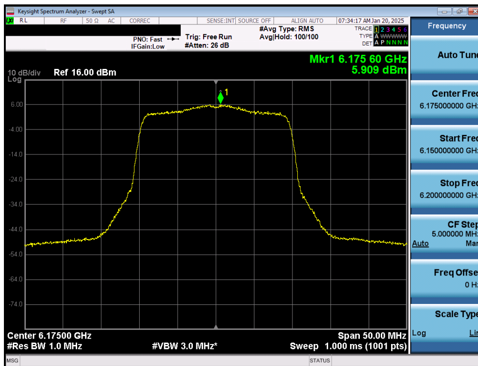
Plot 7-27. Power Spectral Density Plot MIMO ANT1 (20MHz 802.11ax (UNII Band 5) – Ch. 45) – SP
