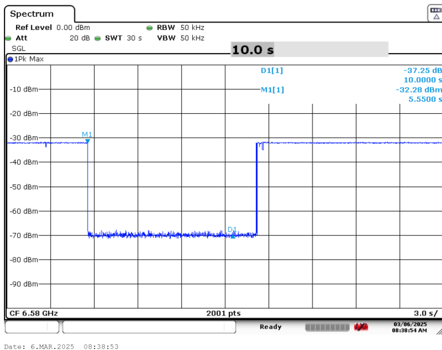
Plot 7-69. Contention Based Protocol Timing Plot (160MHz (UNII Band 6) – Ch. 111 High)
