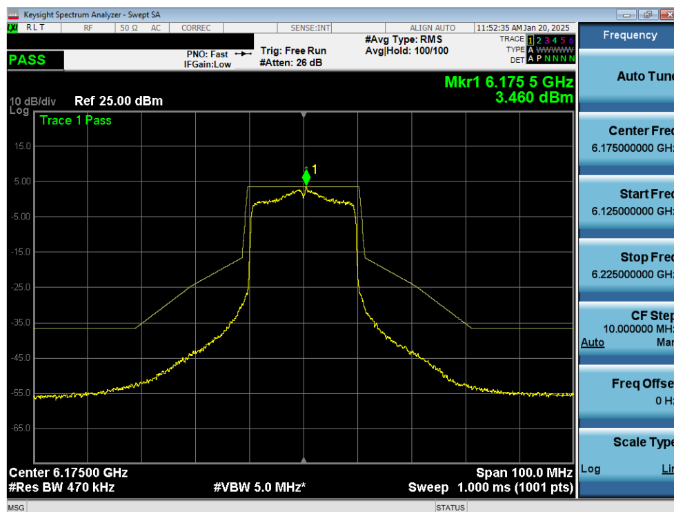
Plot 7-57. In Band Emissions Plot MIMO ANT2 (20MHz 802.11ax (UNII Band 5) – Ch. 45) – SP
