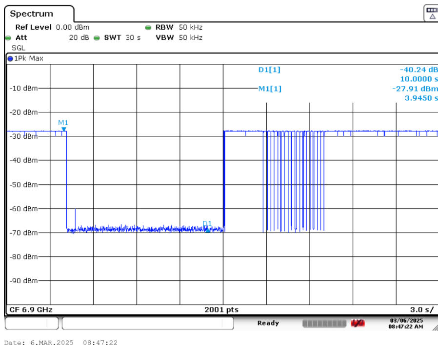
Plot 7-73. Contention Based Protocol Timing Plot (160MHz (UNII Band 7) – Ch. 175 High)
