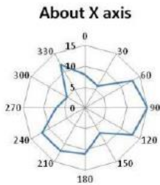
Radiation gain diagram
